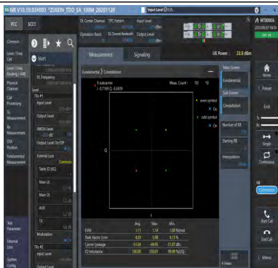
1-N78-3450-3550-PC3-30-100-M-1-DFT-PI2BPSK-Outer_Full-270@0-Ant1-see graph-PASS
