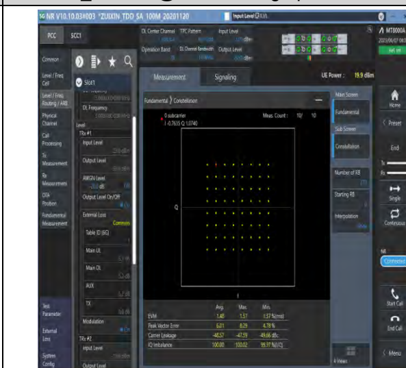
1-N78-3450-3550-PC3-30-100-M-8-CP-64QAM-Outer_Full-273@0-Ant1-see graph-PASS
