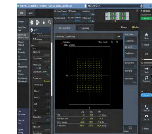
1-N78-3450-3550-PC3-30-100-M-5-DFT-256QAM-Outer_Full-270@0-Ant1-see graph-PASS
