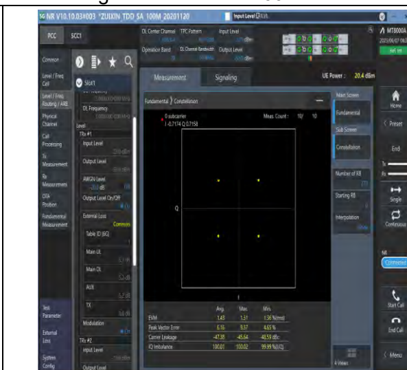
1-N78-3450-3550-PC3-30-100-M-6-CP-QPSK-Outer_Full-273@0-Ant1-see graph-PASS
