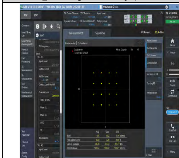
1-N78-3450-3550-PC3-30-100-M-7-CP-16QAM-Outer_Full-273@0-Ant1-see graph-PASS
