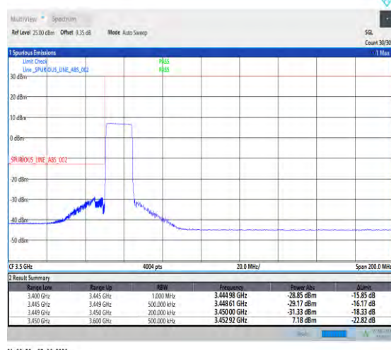
1-N78-3450-3550-PC3-30-15-L-6-CP-QPSK-Outer_Full-38@0-Ant1-1--PASS-see graph
