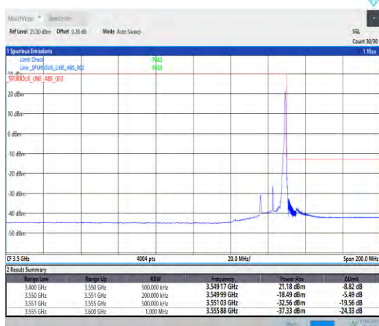
1-N78-3450-3550-PC3-30-15-H-5-CP-QPSK-Edge_1RB_Right-1@37-Ant1-1--PASS-see graph
