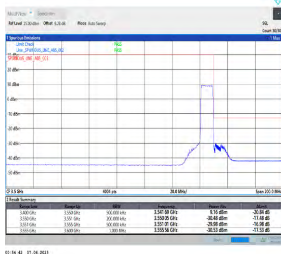
1-N78-3450-3550-PC3-30-10-H-6-CP-QPSK-Outer_Full-24@0-Ant1-1--PASS-see graph
