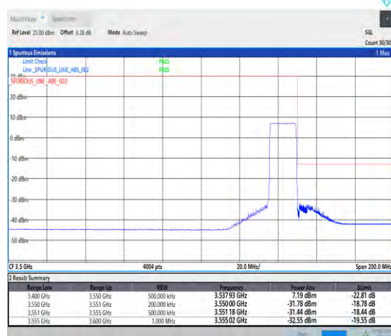
1-N78-3450-3550-PC3-30-15-H-6-CP-QPSK-Outer_Full-38@0-Ant1-1--PASS-see graph
