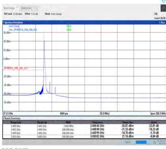
1-N78-3450-3550-PC3-30-15-L-4-CP-QPSK-Edge_1RB_Left-1@0-Ant1-1--PASS-see graph
