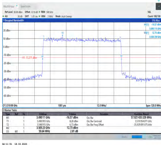
1-N78-3450-3550-PC3-30-60-H-2-DFT-PI2BPSK-Outer_Full-162@0-Ant1-57.921-59.64-≤60-PASS
