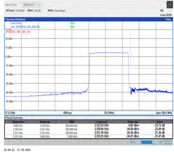
1-N78-3450-3550-PC3-30-50-H-3-DFT-PI2BPSK-Outer_Full-128@0-Ant1-1--PASS-see graph
