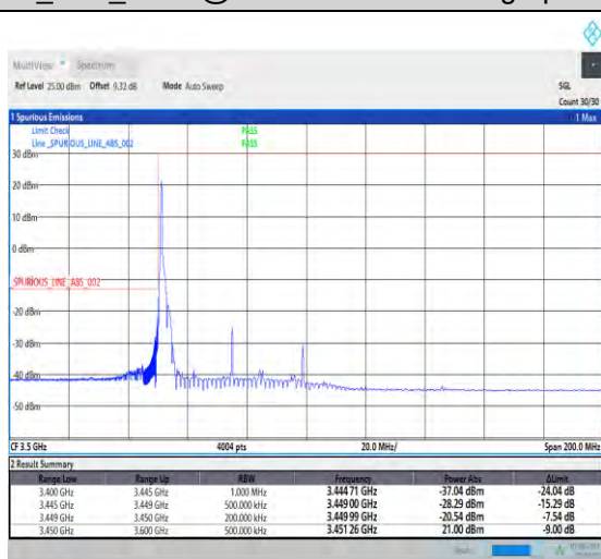
1-N78-3450-3550-PC3-30-50-L-1-DFT-PI2BPSK-Edge_1RB_Left-1@0-Ant1-1--PASS-see graph
