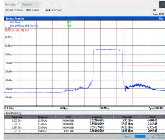
1-N78-3450-3550-PC3-30-40-H-3-DFT-PI2BPSK-Outer_Full-100@0-Ant1-1--PASS-see graph
