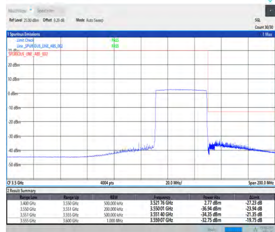
1-N78-3450-3550-PC3-30-40-H-6-CP-QPSK-Outer_Full-106@0-Ant1-1--PASS-see graph
