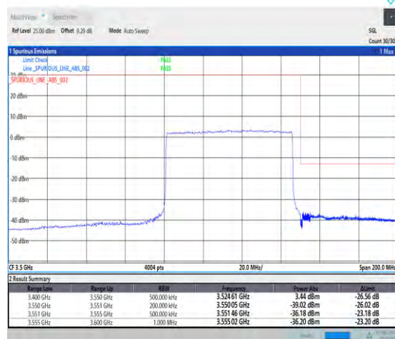
1-N78-3450-3550-PC3-30-70-H-3-DFT-PI2BPSK-Outer_Full-180@0-Ant1-1--PASS-see graph
