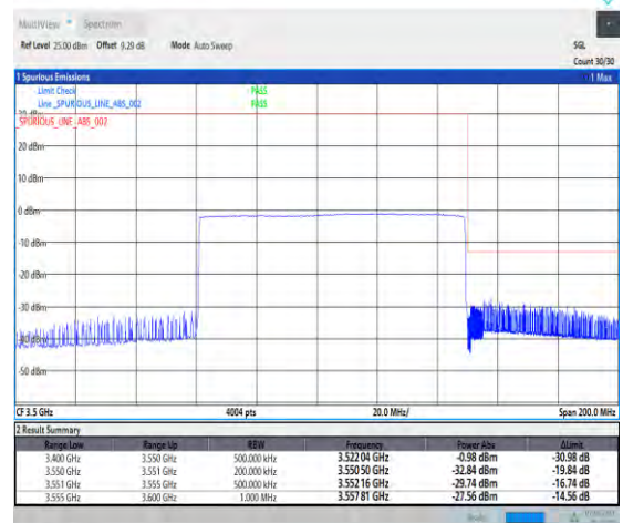
1-N78-3450-3550-PC3-30-90-H-6-CP-QPSK-Outer_Full-245@0-Ant1-1--PASS-see graph
