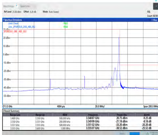
1-N78-3450-3550-PC3-30-90-H-5-CP-QPSK-Edge_1RB_Right-1@244-Ant1-1--PASS-see graph
