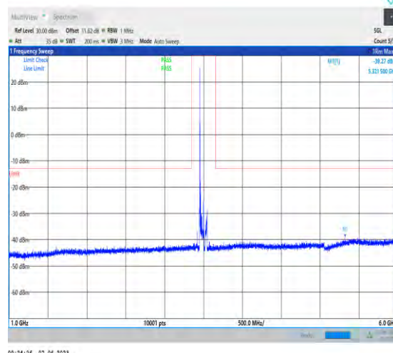
1-N78-3450-3550-PC3-30-100-M-1-N/A-DFT-PI2BPS K-Inner_1RB_Left-1@1-1000-6000-Ant1-5321.50--39 .27--13-PASS
