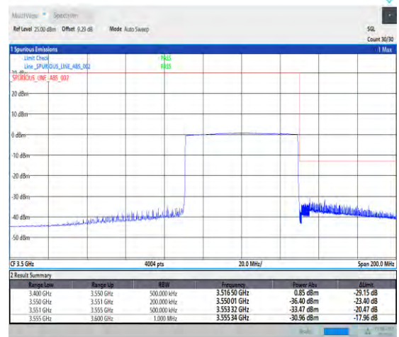
1-N78-3450-3550-PC3-30-60-H-6-CP-QPSK-Outer_Full-162@0-Ant1-1--PASS-see graph
