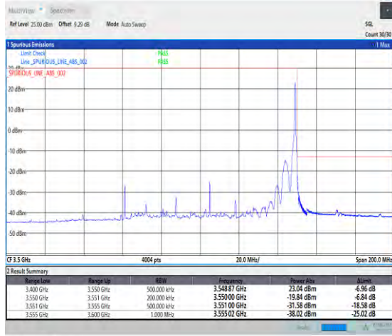
1-N78-3450-3550-PC3-30-90-H-2-DFT-PI2BPSK-Edge_1RB_Right-1@244-Ant1-1--PASS-see graph
