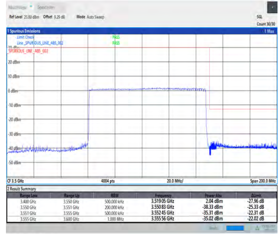
1-N78-3450-3550-PC3-30-90-H-3-DFT-PI2BPSK-Outer_Full-240@0-Ant1-1--PASS-see graph
