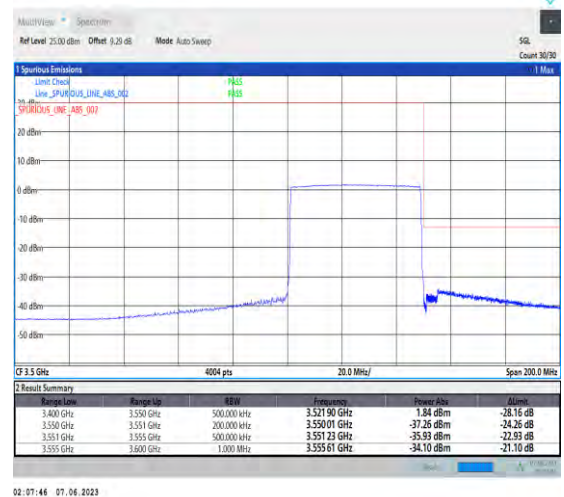
1-N78-3450-3550-PC3-30-50-H-6-CP-QPSK-Outer_Full-133@0-Ant1-1--PASS-see graph
