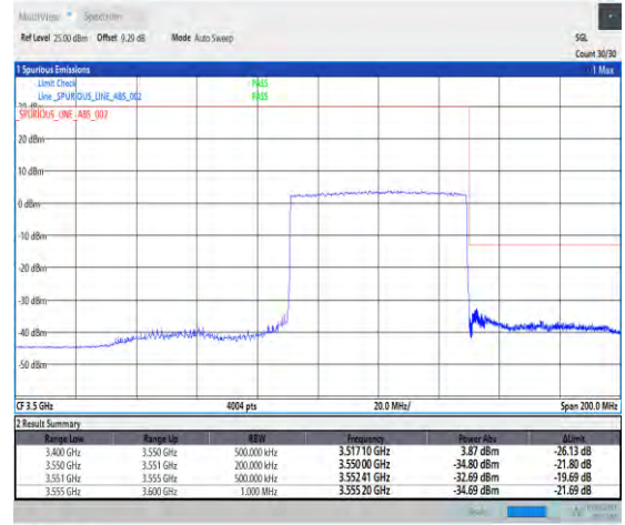
1-N78-3450-3550-PC3-30-60-H-3-DFT-PI2BPSK-Outer_Full-162@0-Ant1-1--PASS-see graph
