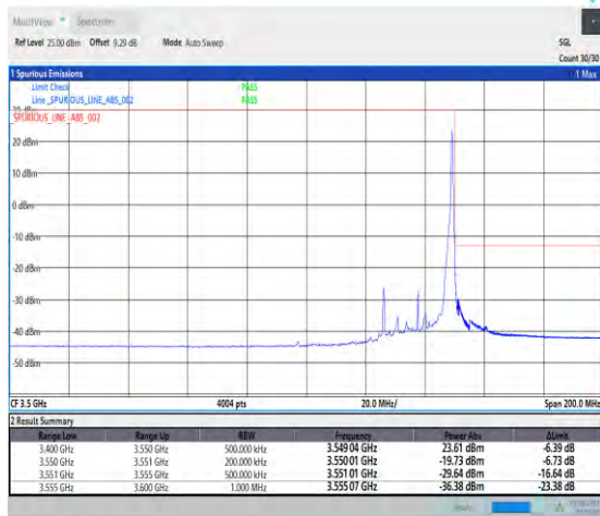
1-N78-3450-3550-PC3-30-25-H-2-DFT-PI2BPSK-Edge_1RB_Right-1@64-Ant1-1--PASS-see graph
