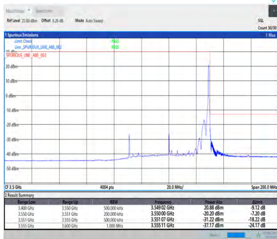
1-N78-3450-3550-PC3-30-60-H-5-CP-QPSK-Edge_1RB_Right-1@161-Ant1-1--PASS-see graph
