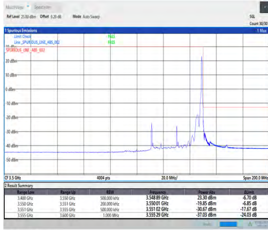
1-N78-3450-3550-PC3-30-40-H-2-DFT-PI2BPSK-Edge_1RB_Right-1@105-Ant1-1--PASS-see graph
