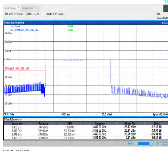
1-N78-3450-3550-PC3-30-80-L-6-CP-QPSK-Outer_Full-217@0-Ant1-1--PASS-see graph
