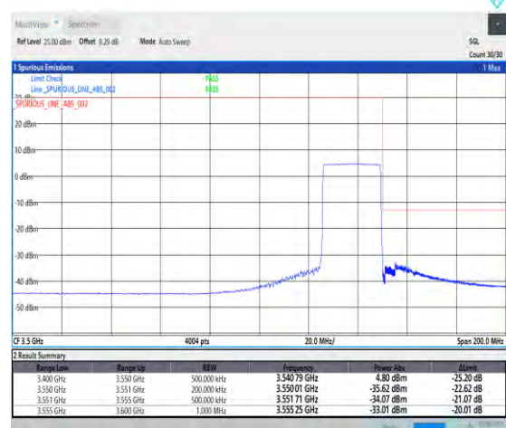
1-N78-3450-3550-PC3-30-25-H-6-CP-QPSK-Outer_Full-65@0-Ant1-1--PASS-see graph
