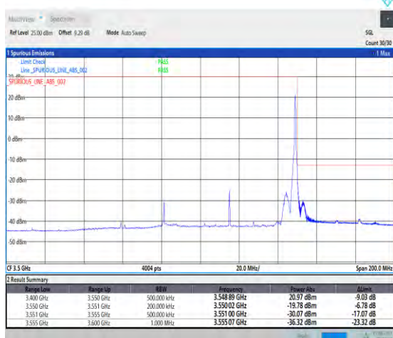
1-N78-3450-3550-PC3-30-70-H-5-CP-QPSK-Edge_1RB_Right-1@188-Ant1-1--PASS-see graph
