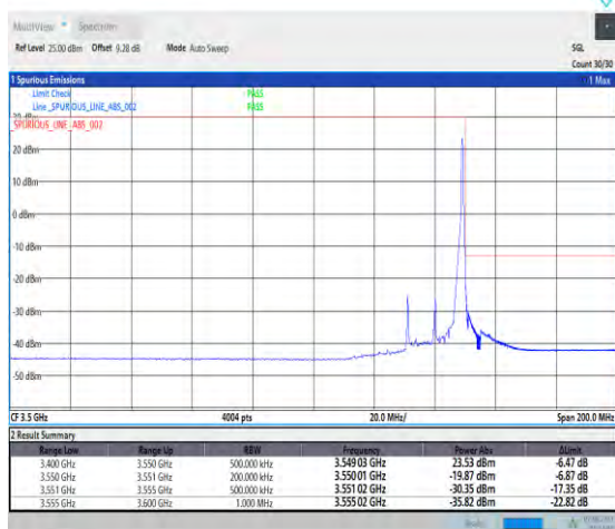
1-N78-3450-3550-PC3-30-20-H-2-DFT-PI2BPSK-Edge_1RB_Right-1@50-Ant1-1--PASS-see graph
