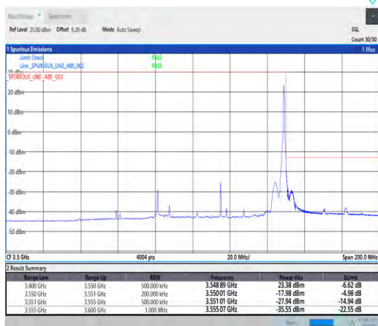
1-N78-3450-3550-PC3-30-70-H-2-DFT-PI2BPSK-Edge_1RB_Right-1@188-Ant1-1--PASS-see graph
