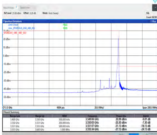
1-N78-3450-3550-PC3-30-25-H-5-CP-QPSK-Edge_1RB_Right-1@64-Ant1-1--PASS-see graph
