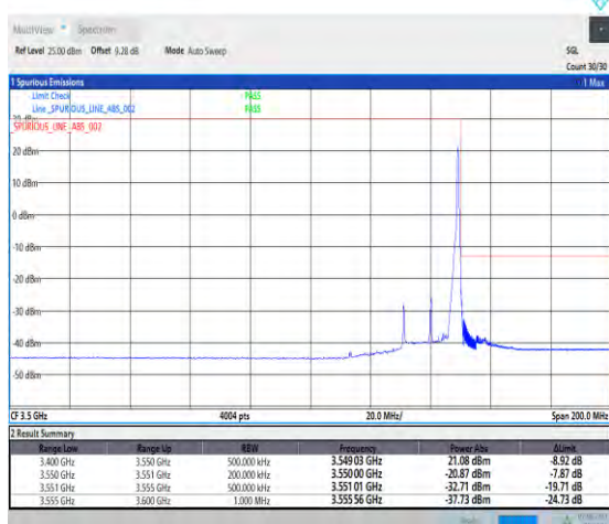
1-N78-3450-3550-PC3-30-20-H-5-CP-QPSK-Edge_1RB_Right-1@50-Ant1-1--PASS-see graph
