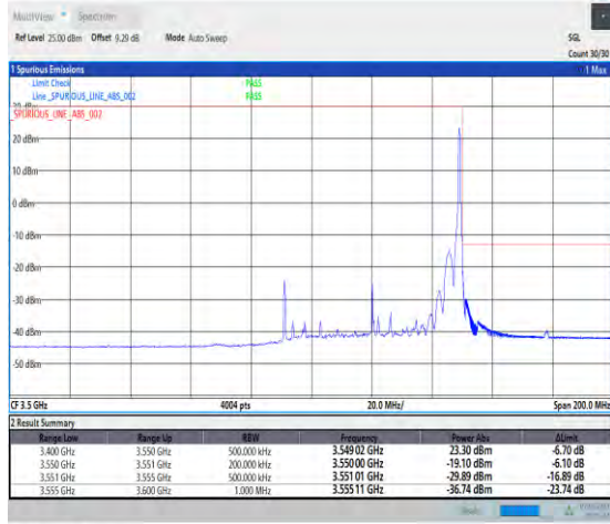
1-N78-3450-3550-PC3-30-60-H-2-DFT-PI2BPSK-Edge_1RB_Right-1@161-Ant1-1--PASS-see graph
