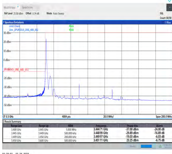
1-N78-3450-3550-PC3-30-80-L-1-DFT-PI2BPSK-Edge_1RB_Left-1@0-Ant1-1--PASS-see graph
