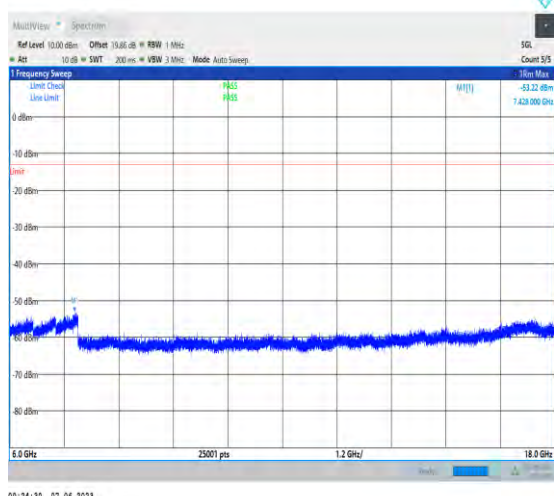
1-N78-3450-3550-PC3-30-100-M-1-N/A-DFT-PI2BP SK-Inner_1RB_Left-1@1-6000-18000-Ant1-7428.00 --53.22--13-PASS
