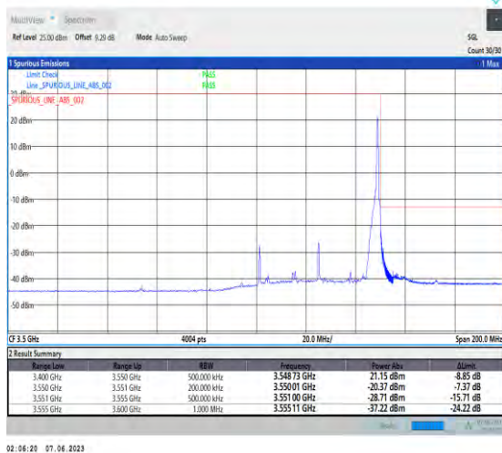
1-N78-3450-3550-PC3-30-50-H-5-CP-QPSK-Edge_1RB_Right-1@132-Ant1-1--PASS-see graph
