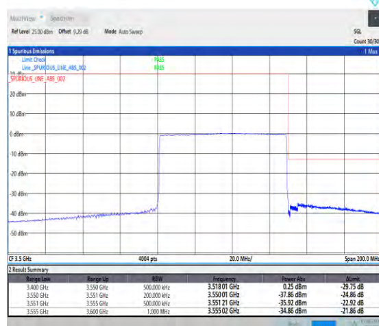
1-N78-3450-3550-PC3-30-70-H-6-CP-QPSK-Outer_Full-189@0-Ant1-1--PASS-see graph
