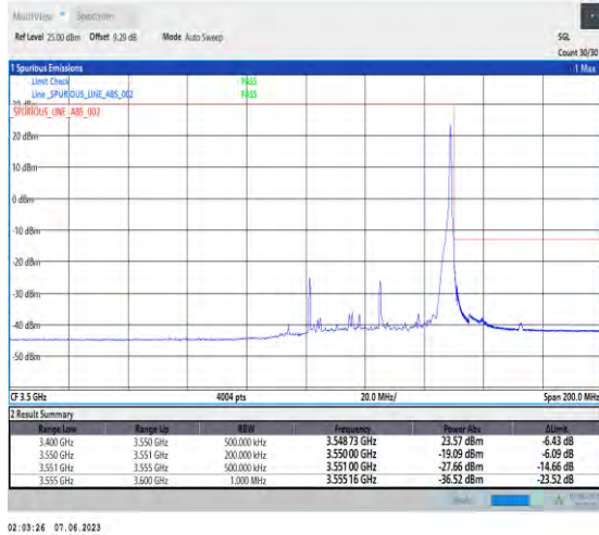
1-N78-3450-3550-PC3-30-50-H-2-DFT-PI2BPSK-Edge_1RB_Right-1@132-Ant1-1--PASS-see graph
