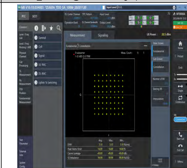
1-N78-3700-3800-PC3-30-100-M-8-CP-64QAM-Outer_Full-273@0-Ant1-see graph-PASS
