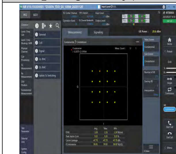
1-N78-3700-3800-PC3-30-100-M-7-CP-16QAM-Outer_Full-273@0-Ant1-see graph-PASS
