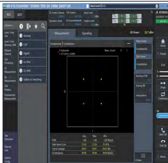
1-N78-3700-3800-PC3-30-100-M-2-DFT-QPSK-Out_Full-270@0-Ant1-see graph-PASS
