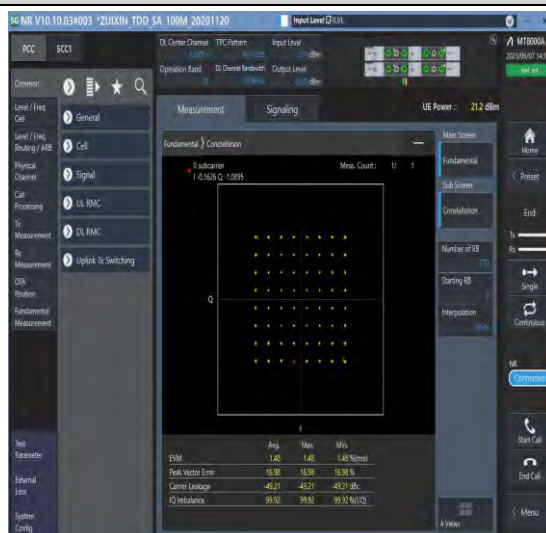
1-N78-3700-3800-PC3-30-100-M-4-DFT-64QAM-Out_Full-270@0-Ant1-see graph-PASS
