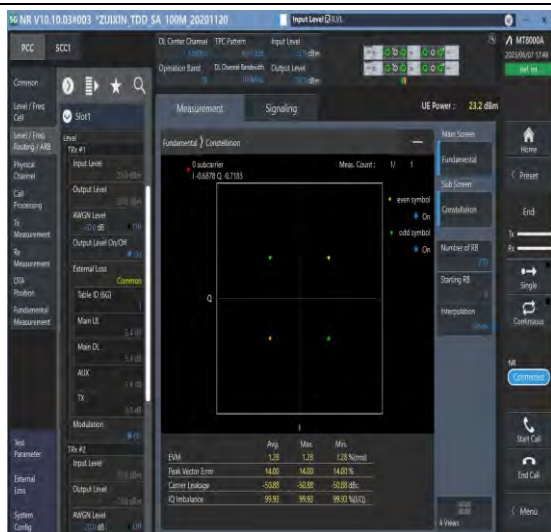
1-N78-3700-3800-PC3-30-100-M-1-DFT-PI2BPSK-Out_Full-270@0-Ant1-see graph-PASS
