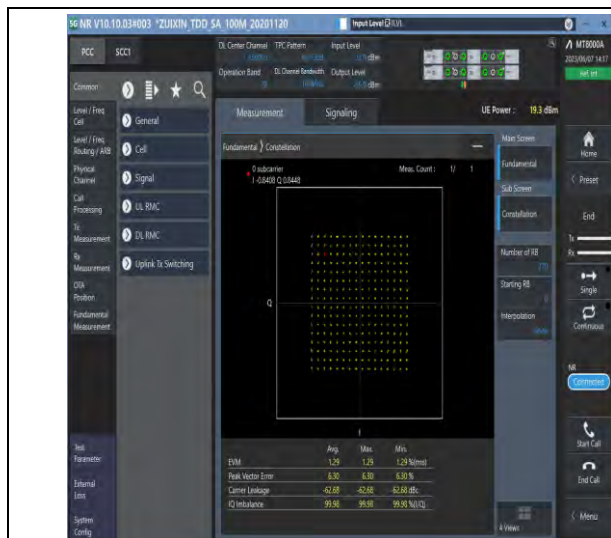
1-N78-3700-3800-PC3-30-100-M-5-DFT-256QAM-Outer_Full-270@0-Ant1-see graph-PASS
