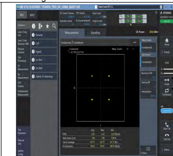
1-N78-3700-3800-PC3-30-100-M-6-CP-QPSK-Outer_Full-273@0-Ant1-see graph-PASS
