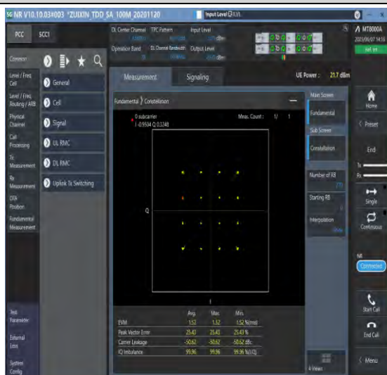
1-N78-3700-3800-PC3-30-100-M-3-DFT-16QAM-Out_Full-270@0-Ant1-see graph-PASS
