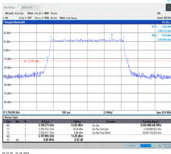
1-N78-3700-3800-PC3-30-10-L-3-DFT-16QAM-Out_Full-24@0-Ant1-8.565-9.460-≤10-PASS
