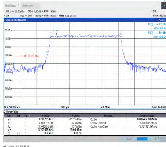
1-N78-3700-3800-PC3-30-10-L-2-DFT-PI2BPSK-Out_Full-24@0-Ant1-8.607-9.400-≤10-PASS
