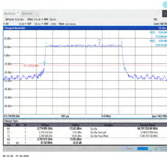
1-N78-3700-3800-PC3-30-70-M-1-DFT-QPSK-Outer_Full-180@0-Ant1-64.192-67.340-≤70-PASS
