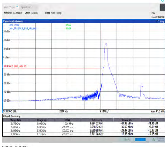
1-N78-3700-3800-PC3-30-20-L-1-DFT-PI2BPSK-Edge_1RB_Left-1@0-Ant1-1--PASS-see graph
