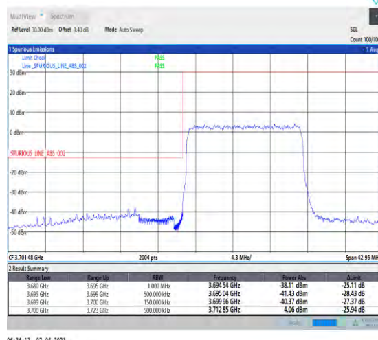
1-N78-3700-3800-PC3-30-15-L-3-DFT-PI2BPSK-Outer_Full-36@0-Ant1-1--PASS-see graph
