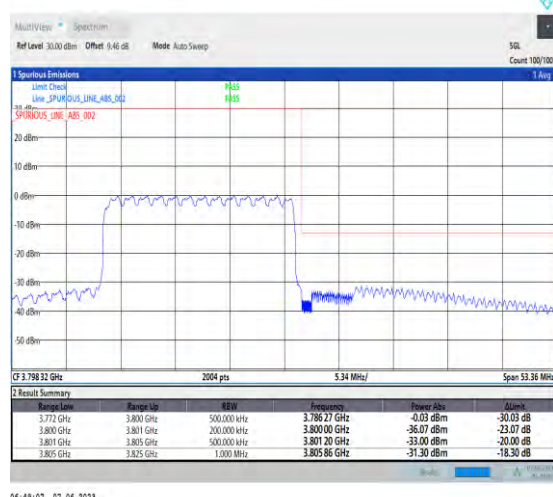
1-N78-3700-3800-PC3-30-20-H-6-CP-QPSK-Outer_Full-51@0-Ant1-1--PASS-see graph
