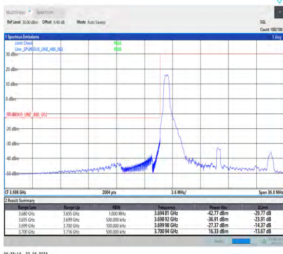
1-N78-3700-3800-PC3-30-15-L-1-DFT-PI2BPSK-Edge_1RB_Left-1@0-Ant1-1--PASS-see graph
