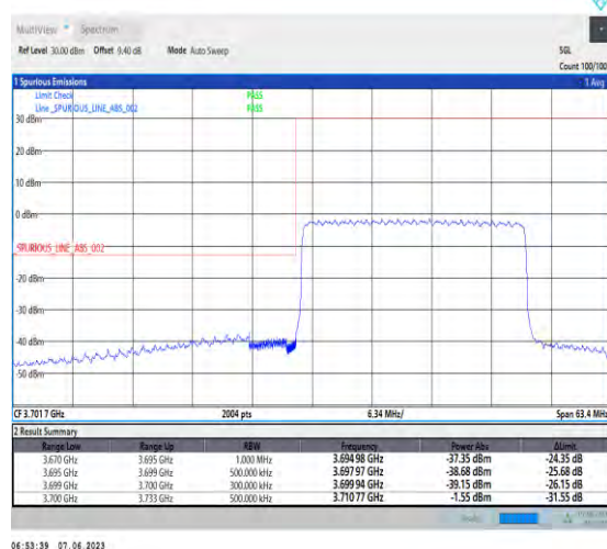
1-N78-3700-3800-PC3-30-25-L-6-CP-QPSK-Outer_Full-65@0-Ant1-1--PASS-see graph
