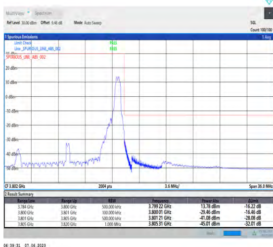
1-N78-3700-3800-PC3-30-15-H-5-CP-QPSK-Edge_1RB_Right-1@37-Ant1-1--PASS-see graph
