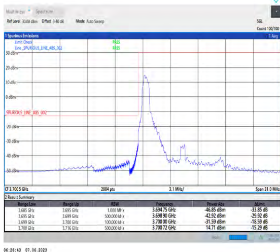
1-N78-3700-3800-PC3-30-10-L-4-CP-QPSK-Edge_1RB_Left-1@0-Ant1-1--PASS-see graph
