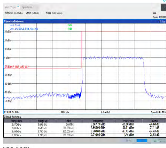
1-N78-3700-3800-PC3-30-25-L-3-DFT-PI2BPSK-Outer_Full-64@0-Ant1-1--PASS-see graph
