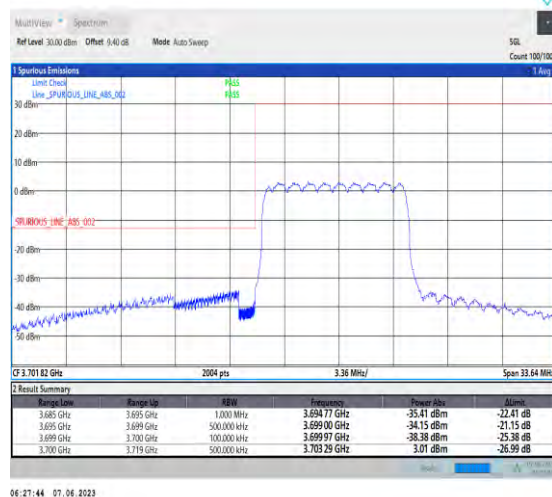
1-N78-3700-3800-PC3-30-10-L-6-CP-QPSK-Outer_Full-24@0-Ant1-1--PASS-see graph
