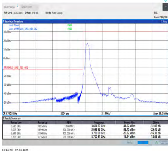
1-N78-3700-3800-PC3-30-10-L-1-DFT-PI2BPSK-Edge_1RB_Left-1@0-Ant1-1--PASS-see graph
