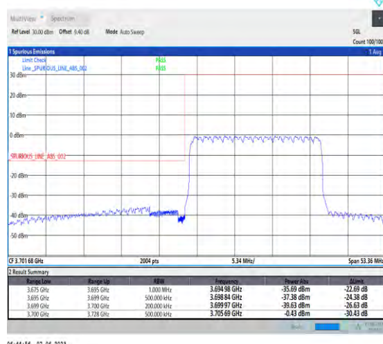
1-N78-3700-3800-PC3-30-20-L-6-CP-QPSK-Outer_Full-51@0-Ant1-1--PASS-see graph
