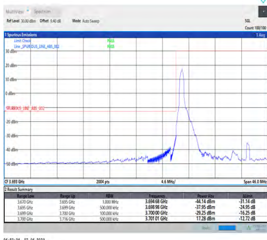
1-N78-3700-3800-PC3-30-25-L-1-DFT-PI2BPSK-Edge_1RB_Left-1@0-Ant1-1--PASS-see graph
