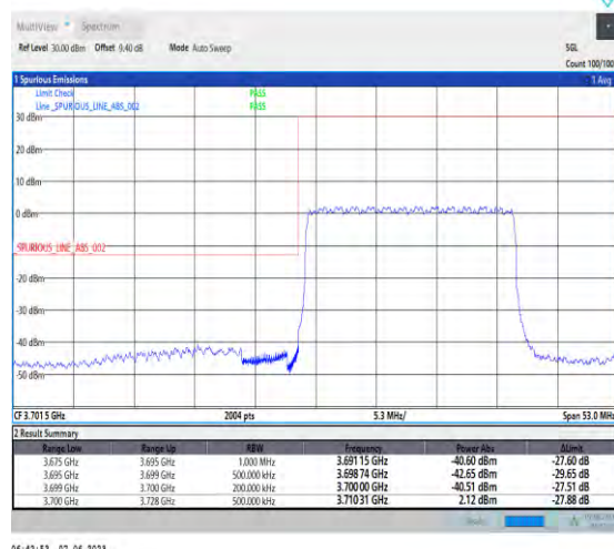
1-N78-3700-3800-PC3-30-20-L-3-DFT-PI2BPSK-Outer_Full-50@0-Ant1-1--PASS-see graph
