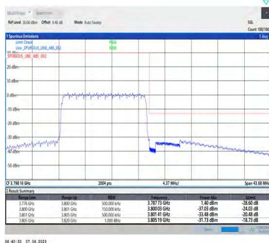
1-N78-3700-3800-PC3-30-15-H-6-CP-QPSK-Outer_Full-38@0-Ant1-1--PASS-see graph
