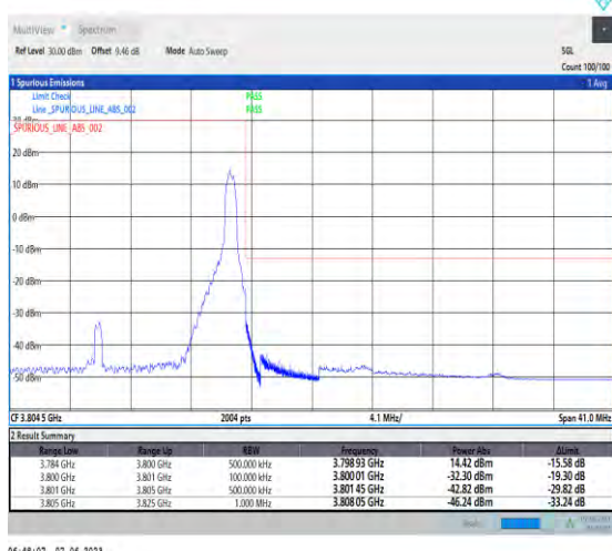
1-N78-3700-3800-PC3-30-20-H-5-CP-QPSK-Edge_1RB_Right-1@50-Ant1-1--PASS-see graph
