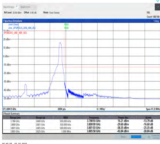
1-N78-3700-3800-PC3-30-20-H-2-DFT-PI2BPSK-Edge_1RB_Right-1@50-Ant1-1--PASS-see graph
