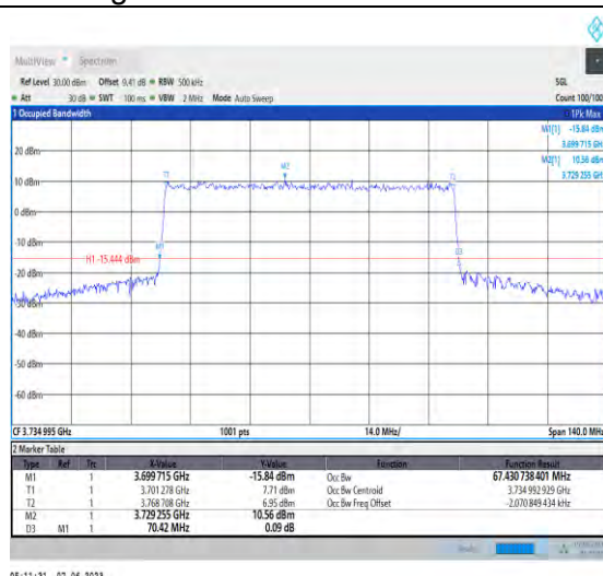
1-N78-3700-3800-PC3-30-70-L-8-CP-64QAM-Outer_Full-189@0-Ant1-67.431-70.420-≤70-PASS
