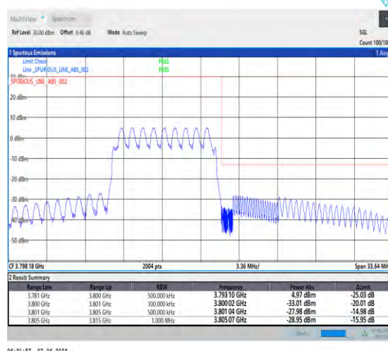
1-N78-3700-3800-PC3-30-10-H-6-CP-QPSK-Outer_Full-24@0-Ant1-1--PASS-see graph
