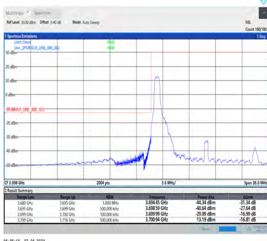
1-N78-3700-3800-PC3-30-15-L-4-CP-QPSK-Edge_1RB_Left-1@0-Ant1-1--PASS-see graph
