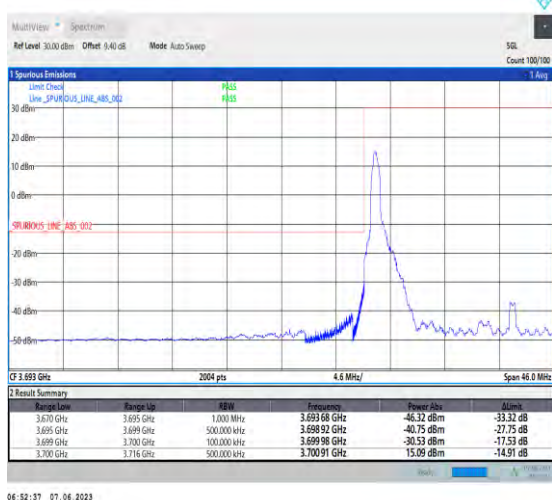
1-N78-3700-3800-PC3-30-25-L-4-CP-QPSK-Edge_1RB_Left-1@0-Ant1-1--PASS-see graph
