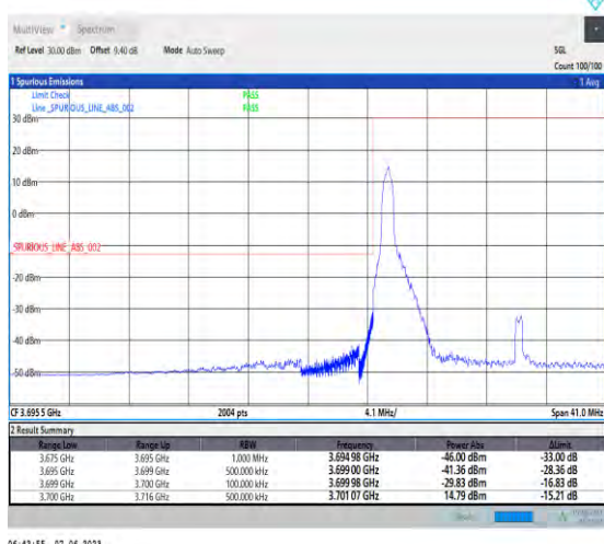
1-N78-3700-3800-PC3-30-20-L-4-CP-QPSK-Edge_1RB_Left-1@0-Ant1-1--PASS-see graph
