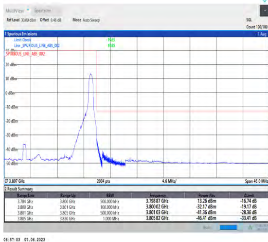
1-N78-3700-3800-PC3-30-25-H-5-CP-QPSK-Edge_1RB_Right-1@64-Ant1-1--PASS-see graph
