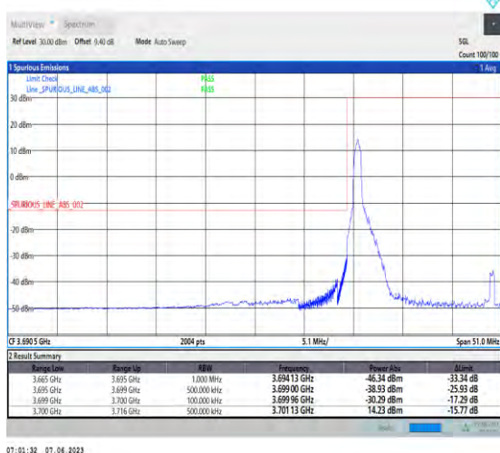
1-N78-3700-3800-PC3-30-30-L-4-CP-QPSK-Edge_1RB_Left-1@0-Ant1-1--PASS-see graph
