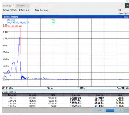
1-N78-3700-3800-PC3-30-90-H-5-CP-QPSK-Edge_1RB_Right-1@244-Ant1-1--PASS-see graph
