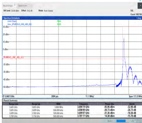
1-N78-3700-3800-PC3-30-90-L-4-CP-QPSK-Edge_1RB_Left-1@0-Ant1-1--PASS-see graph
