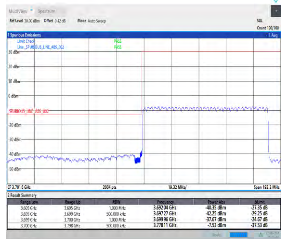
1-N78-3700-3800-PC3-30-90-L-6-CP-QPSK-Outer_Full-245@0-Ant1-1--PASS-see graph
