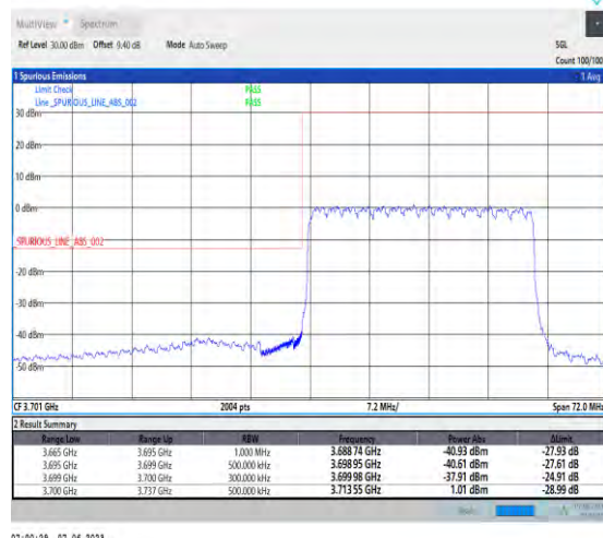
1-N78-3700-3800-PC3-30-30-L-3-DFT-PI2BPSK-Outer_Full-75@0-Ant1-1--PASS-see graph
