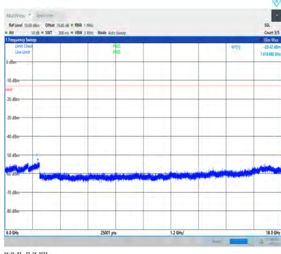
1-N78-3700-3800-PC3-30-100-M-1-N/A-DFT-PI2BP SK-Inner_1RB_Left-1@1-6000-18000-Ant1-7418.88 --53.42--13-PASS
