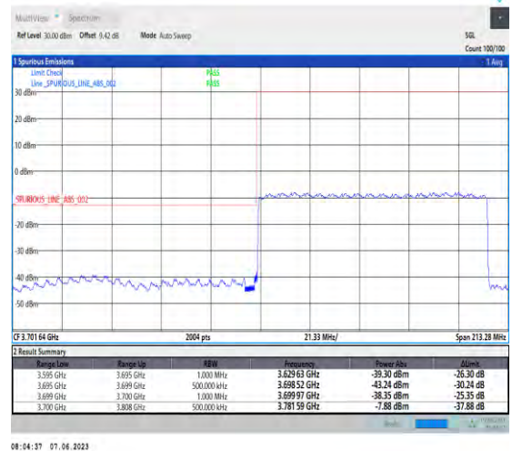
1-N78-3700-3800-PC3-30-100-L-6-CP-QPSK-Outer_Full-273@0-Ant1-1--PASS-see graph
