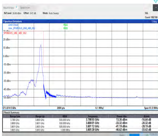
1-N78-3700-3800-PC3-30-40-H-5-CP-QPSK-Edge_1RB_Right-1@105-Ant1-1--PASS-see graph
