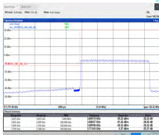
1-N78-3700-3800-PC3-30-60-L-6-CP-QPSK-Outer_Full-162@0-Ant1-1--PASS-see graph
