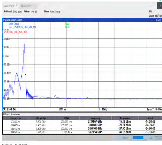
1-N78-3700-3800-PC3-30-90-H-2-DFT-PI2BPSK-Edge_1RB_Right-1@244-Ant1-1--PASS-see graph
