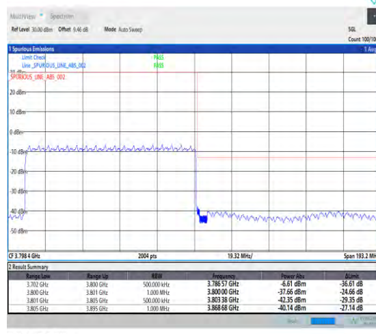
1-N78-3700-3800-PC3-30-90-H-6-CP-QPSK-Outer_Full-245@0-Ant1-1--PASS-see graph
