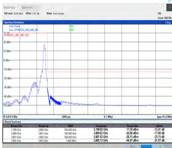
1-N78-3700-3800-PC3-30-40-H-2-DFT-PI2BPSK-Edge_1RB_Right-1@105-Ant1-1--PASS-see graph
