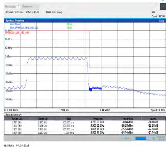
1-N78-3700-3800-PC3-30-25-H-6-CP-QPSK-Outer_Full-65@0-Ant1-1--PASS-see graph
