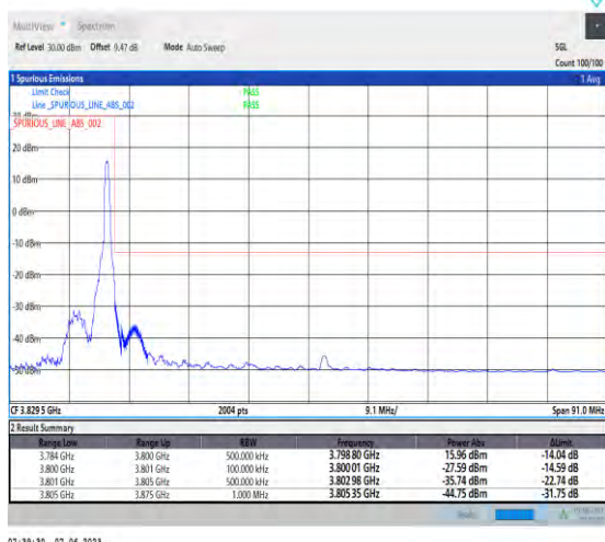
1-N78-3700-3800-PC3-30-70-H-2-DFT-PI2BPSK-Edge_1RB_Right-1@188-Ant1-1--PASS-see graph
