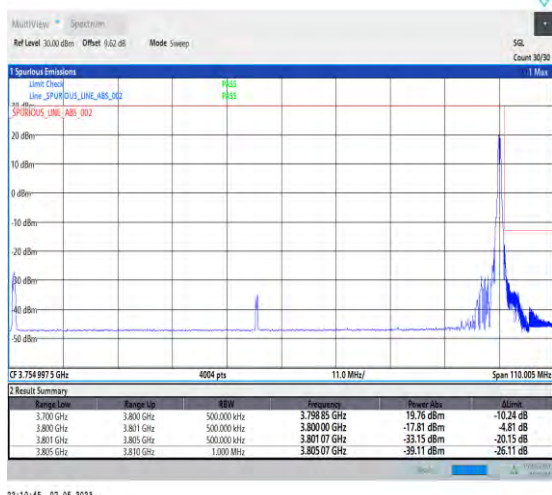
1-N78-3700-3800-PC3-30-100-H-1-DFT-PI2BPSK-Edge_1RB_Right-1@272-Ant1-1--PASS-see graph
