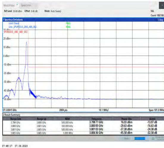
1-N78-3700-3800-PC3-30-80-H-2-DFT-PI2BPSK-Edge_1RB_Right-1@216-Ant1-1--PASS-see graph
