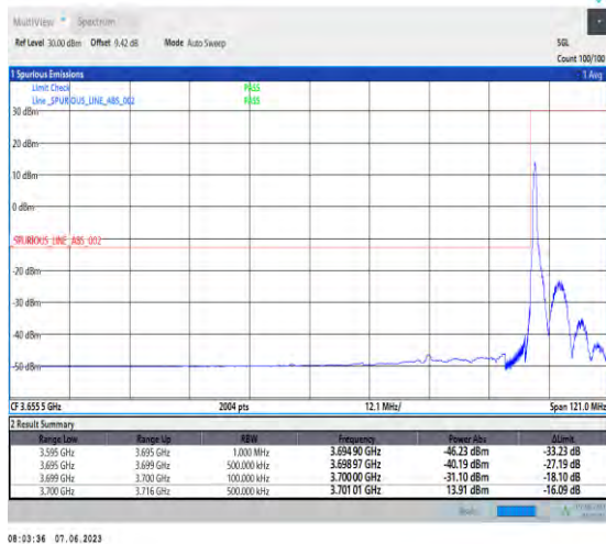
1-N78-3700-3800-PC3-30-100-L-4-CP-QPSK-Edge_1RB_Left-1@0-Ant1-1--PASS-see graph
