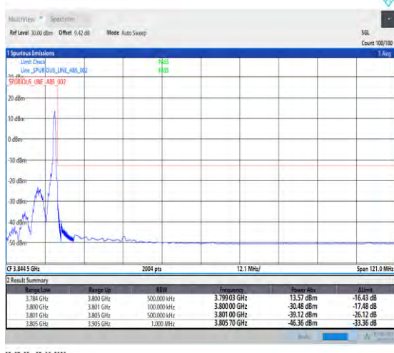
1-N78-3700-3800-PC3-30-100-H-5-CP-QPSK-Edge_1RB_Right-1@272-Ant1-1--PASS-see graph
