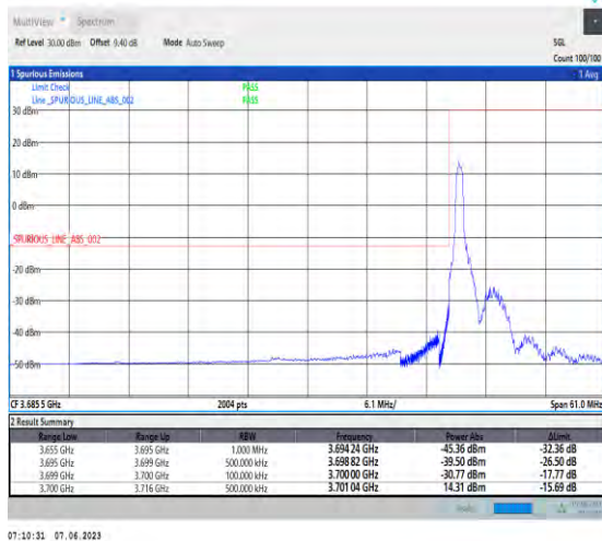
1-N78-3700-3800-PC3-30-40-L-4-CP-QPSK-Edge_1RB_Left-1@0-Ant1-1--PASS-see graph
