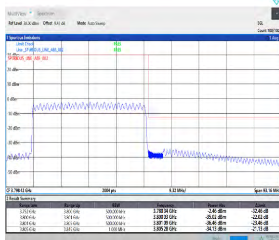
1-N78-3700-3800-PC3-30-40-H-6-CP-QPSK-Outer_Full-106@0-Ant1-1--PASS-see graph
