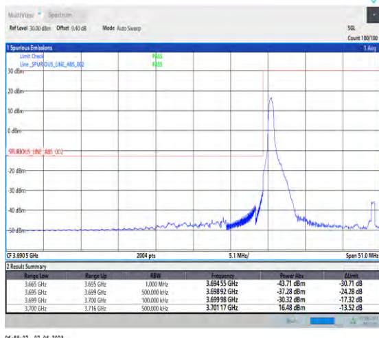
1-N78-3700-3800-PC3-30-30-L-1-DFT-PI2BPSK-Edge_1RB_Left-1@0-Ant1-1--PASS-see graph
