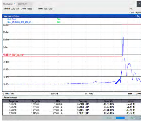
1-N78-3700-3800-PC3-30-90-L-1-DFT-PI2BPSK-Edge_1RB_Left-1@0-Ant1-1--PASS-see graph
