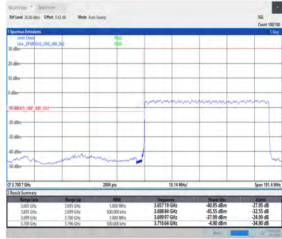
1-N78-3700-3800-PC3-30-90-L-3-DFT-PI2BPSK-Outer_Full-240@0-Ant1-1--PASS-see graph
