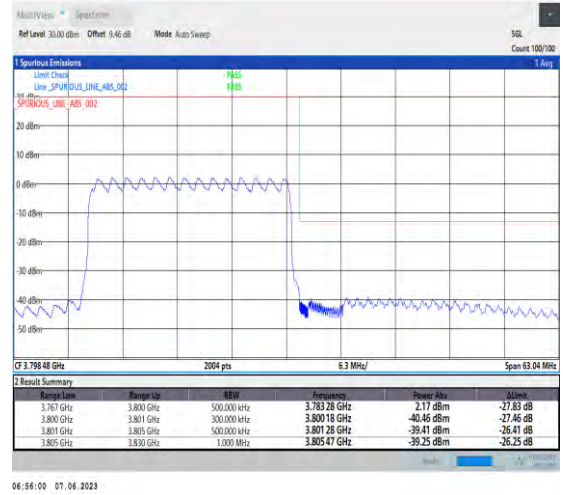
1-N78-3700-3800-PC3-30-25-H-3-DFT-PI2BPSK-Outer_Full-64@0-Ant1-1--PASS-see graph
