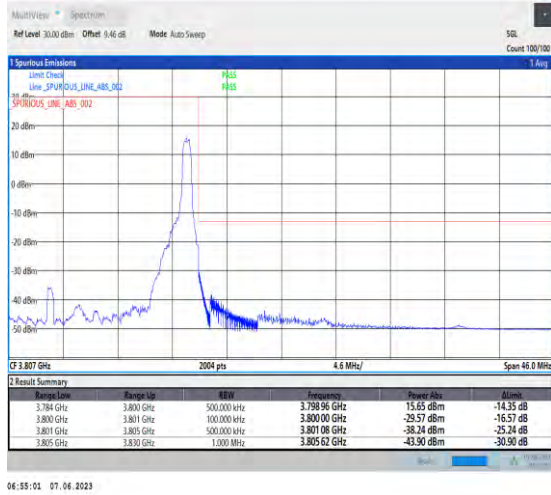
1-N78-3700-3800-PC3-30-25-H-2-DFT-PI2BPSK-Edge_1RB_Right-1@64-Ant1-1--PASS-see graph
