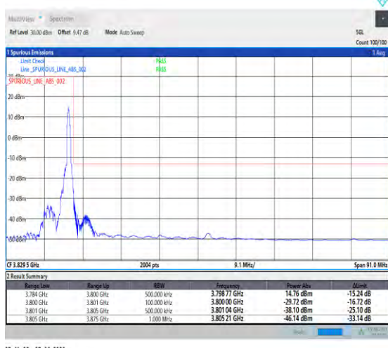
1-N78-3700-3800-PC3-30-70-H-5-CP-QPSK-Edge_1RB_Right-1@188-Ant1-1--PASS-see graph
