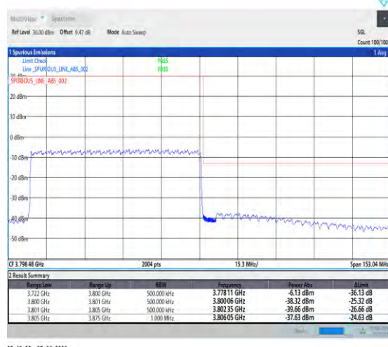
1-N78-3700-3800-PC3-30-70-H-6-CP-QPSK-Outer_Full-189@0-Ant1-1--PASS-see graph
