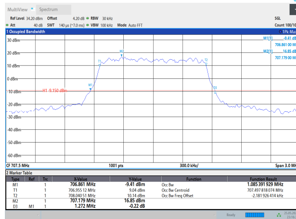
Band12-1.4MHz-QPSK-23095-6RB#0
