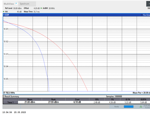
Band13-10MHz-16QAM-23230-50RB#0
