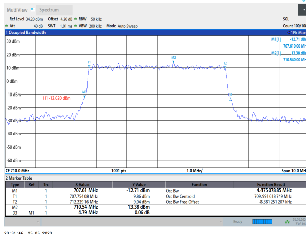
Band17-5MHz-QPSK-23790-25RB#0
