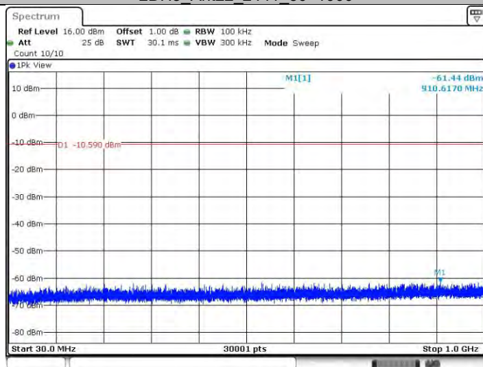
2DH5_Ant22_2441_30~1000
