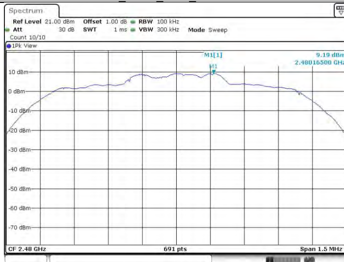
2DH5_Ant22_2480_0~Reference
