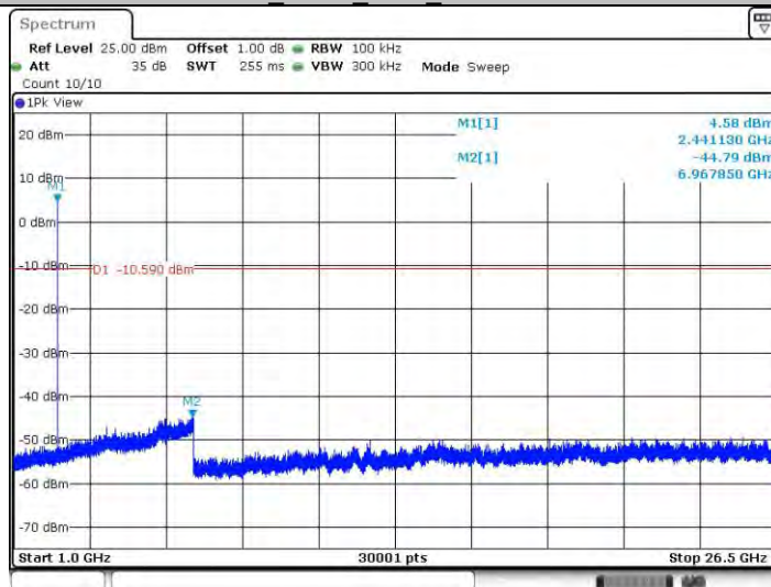
2DH5_Ant22_2441_1000~26500
