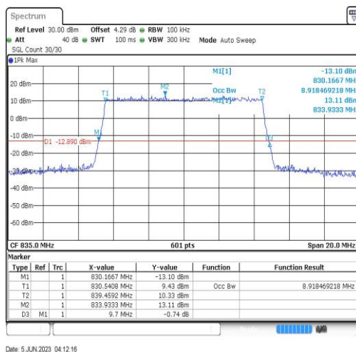
Band19-10MHz-64QAM-24050-50RB#0
