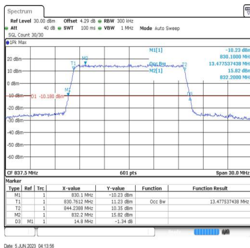
Band19-15MHz-64QAM-24075-75RB#0
