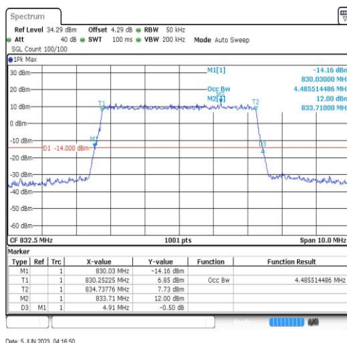
Band19-5MHz-256QAM-24025-25RB#0
