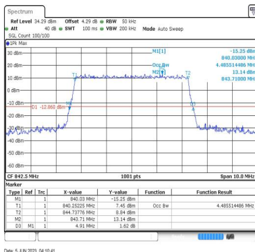
Band19-5MHz-64QAM-24125-25RB#0
