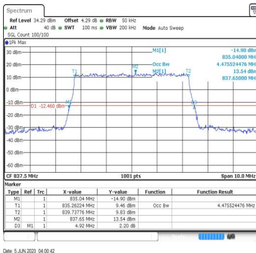
Band19-5MHz-16QAM-24075-25RB#0
