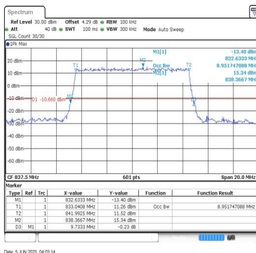
Band19-10MHz-QPSK-24075-50RB#0
