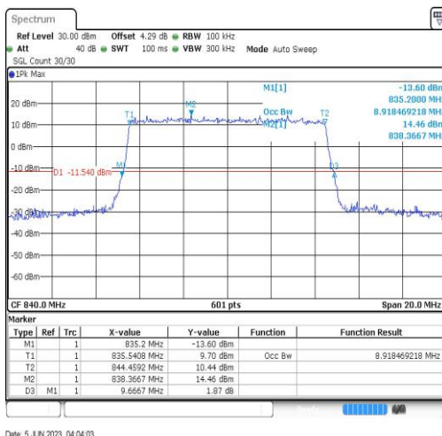
Band19-10MHz-16QAM-24100-50RB#0
