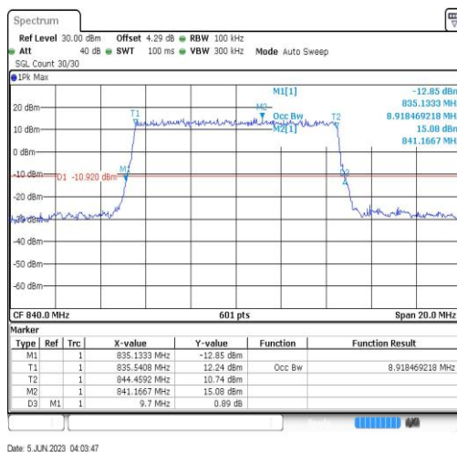
Band19-10MHz-QPSK-24100-50RB#0
