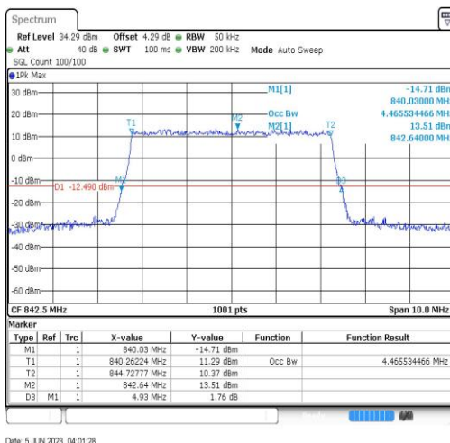
Band19-5MHz-16QAM-24125-25RB#0
