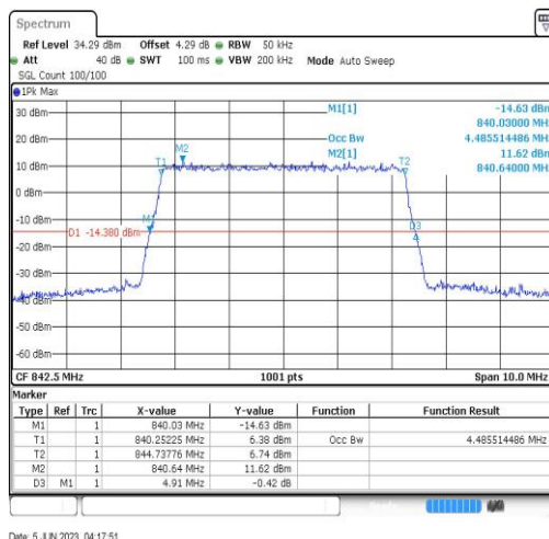
Band19-5MHz-256QAM-24125-25RB#0
