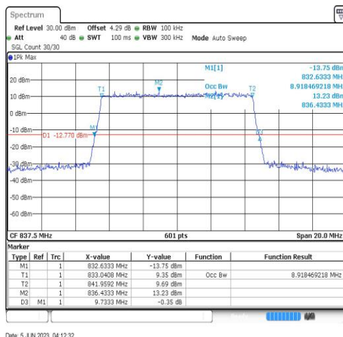
Band19-10MHz-64QAM-24075-50RB#0
