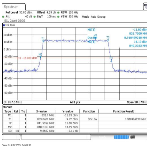
Band19-10MHz-16QAM-24075-50RB#0
