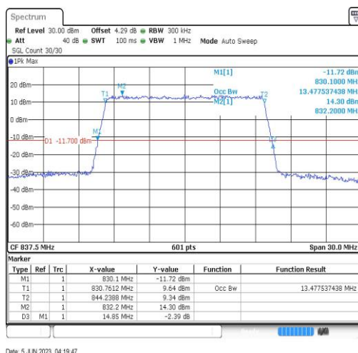
Band19-15MHz-256QAM-24075-75RB#0
