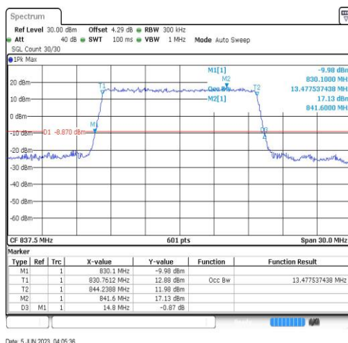
Band19-15MHz-16QAM-24075-75RB#0
