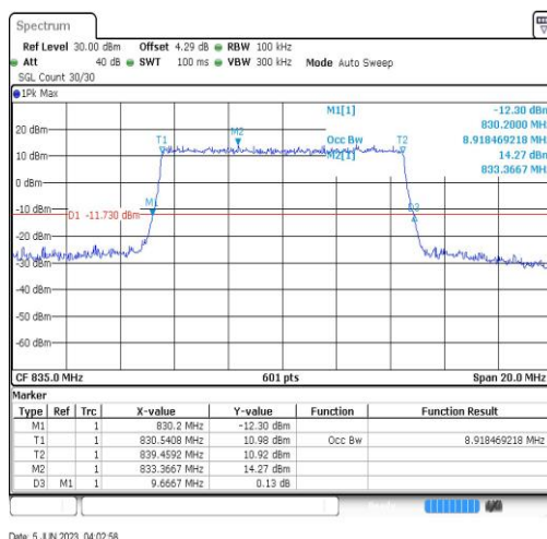
Band19-10MHz-16QAM-24050-50RB#0
