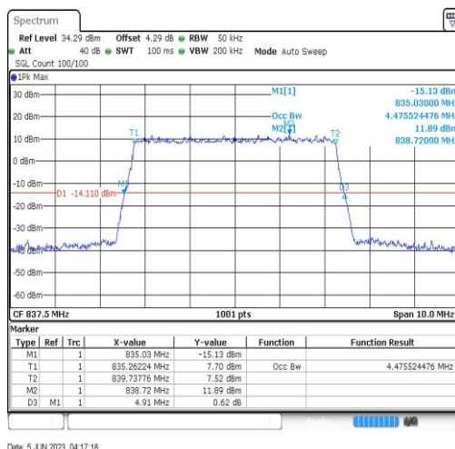
Band19-5MHz-256QAM-24075-25RB#0
