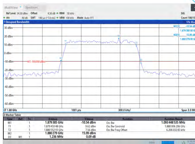
Band2-1.4MHz-QPSK-18900-6RB#0
