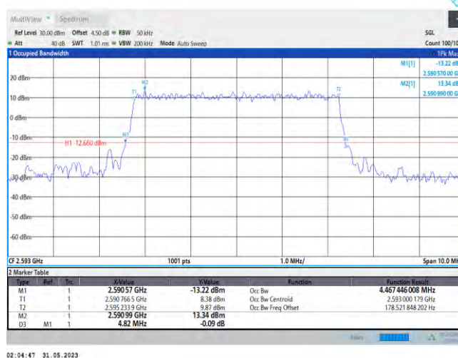
Band41-5MHz-QPSK-40620-25RB#0
