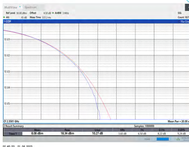
7-7-20MHz-20MHz-QPSK-QPSK-21152-21350-100RB#0-100RB#0
