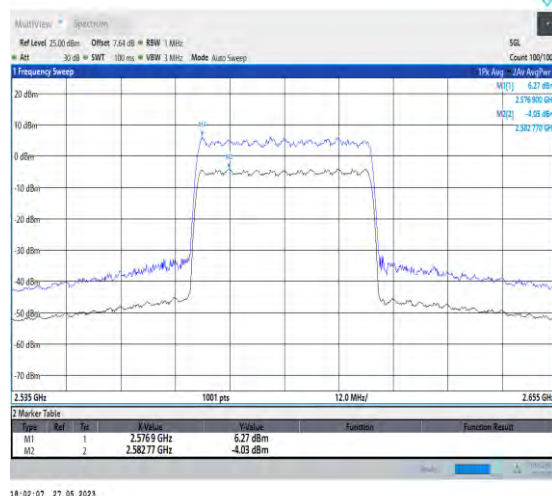
1-N38-PC3-30-40-M-2-CP-256QAM-Outer_Full-106 @0-10.30-100%-0.00-10.30-PASS≤13
