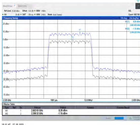
1-N38-PC3-30-40-M-1-DFT-256QAM-Outer_Full-10 0@0-9.55-100%-0.00-9.55-PASS≤13
