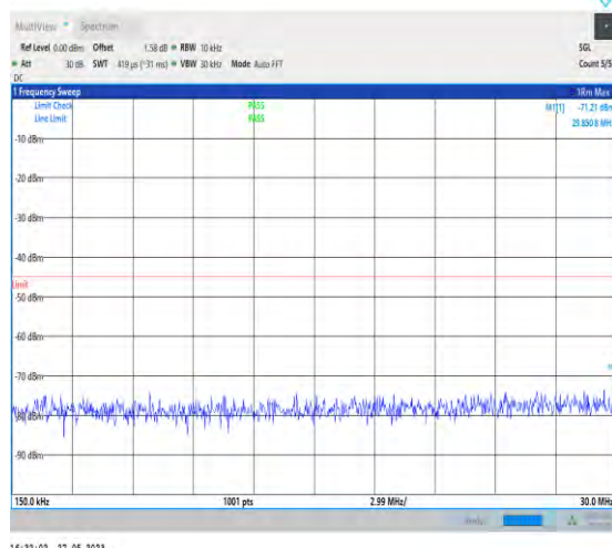
1-N38-PC3-30-40-H-1-N/A-DFT-PI2BPSK-Inner_1RB _Left-1@1-0.15-30-29.85--71.21--45-PASS
