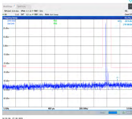
1-N38-PC3-30-40-H-1-N/A-DFT-PI2BPSK-Inner_1RB _Left-1@1-1000-3000-2761.00--39.76--25-PASS
