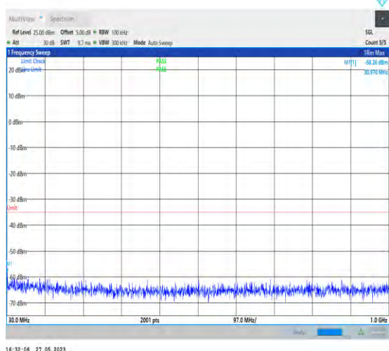
1-N38-PC3-30-40-H-1-N/A-DFT-PI2BPSK-Inner_1R B_Left-1@1-30-1000-30.97--58.26--35-PASS
