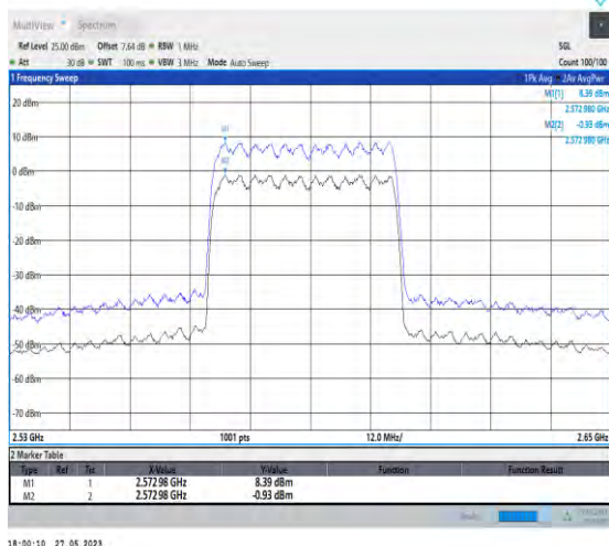
1-N38-PC3-30-40-L-1-DFT-256QAM-Outer_Full-100 @0-9.32-100%-0.00-9.32-PASS≤13
