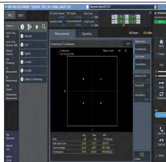
1-N41-PC3-30-100-M-2-DFT-QPSK-Outer_Full-270 @0-see graph-PASS
