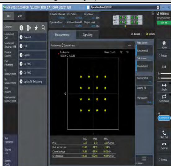
1-N41-PC3-30-100-M-7-CP-16QAM-Outer_Full-273 @0-see graph-PASS
