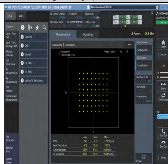
1-N41-PC3-30-100-M-8-CP-64QAM-Outer_Full-273 @0-see graph-PASS
