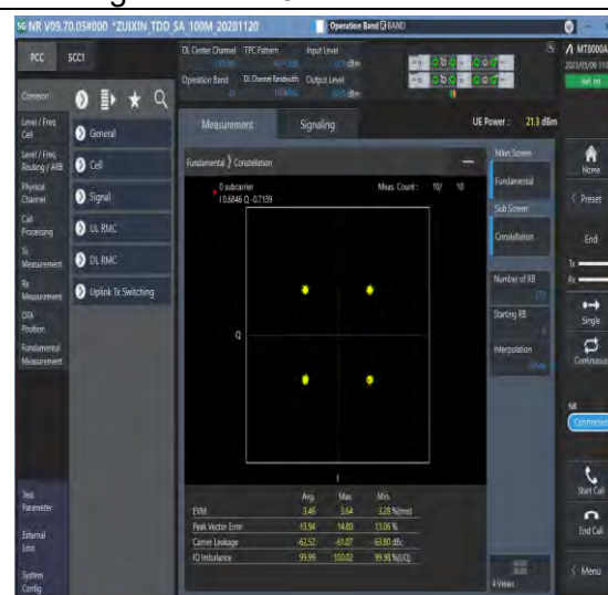
1-N41-PC3-30-100-M-6-CP-QPSK-Outer_Full-273 @0-see graph-PASS
