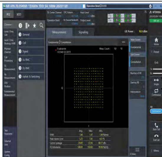
1-N41-PC3-30-100-M-9-CP-256QAM-Outer_Full-273@0-see graph-PASS
