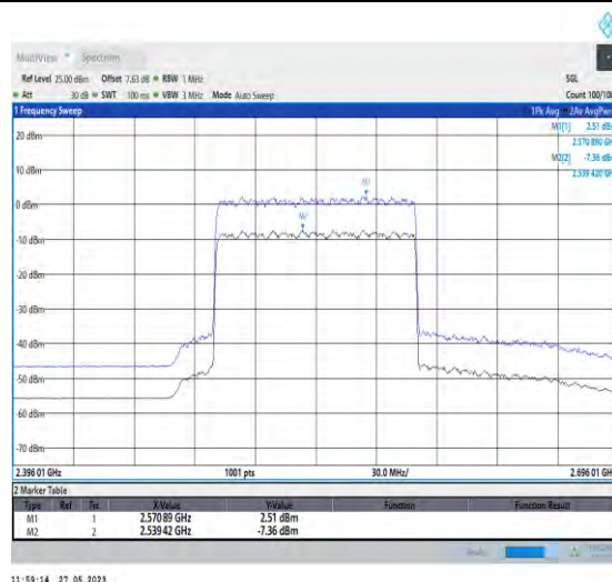
1-N41-PC3-30-100-L-2-CP-256QAM-Outer_Full-27 3@0-9.87-100%-0.00-9.87-PASS-≤13
