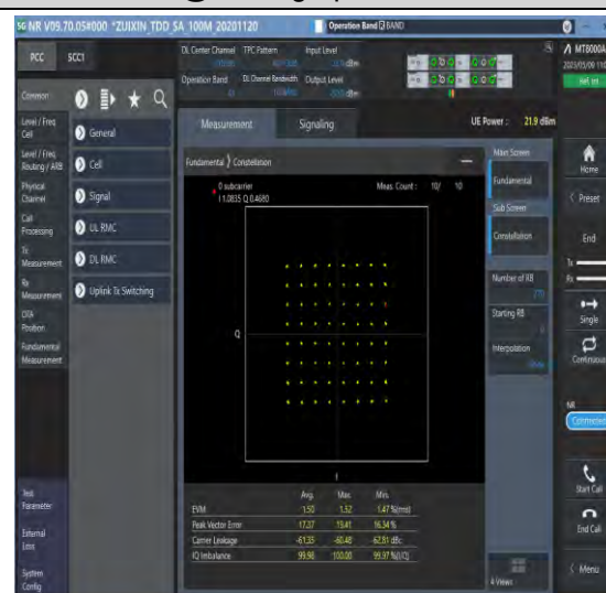
1-N41-PC3-30-100-M-4-DFT-64QAM-Outer_Full-27 0@0-see graph-PASS
