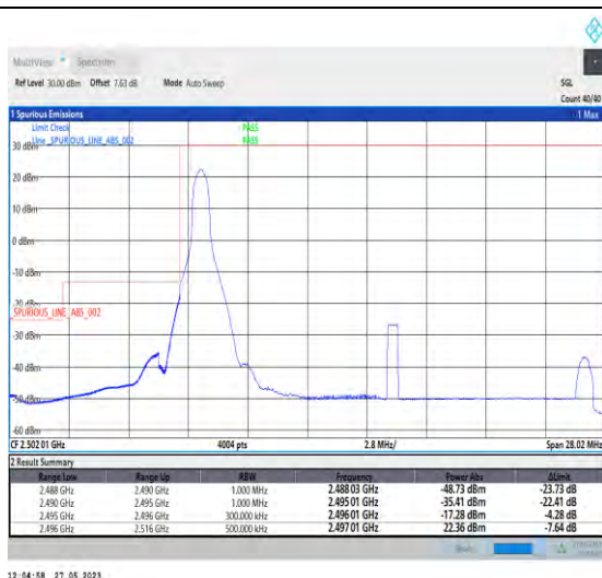
1-N41-PC3-30-20-L-1-DFT-PI2BPSK-Edge_1RB_Left-1@0-1--PASS-see graph
