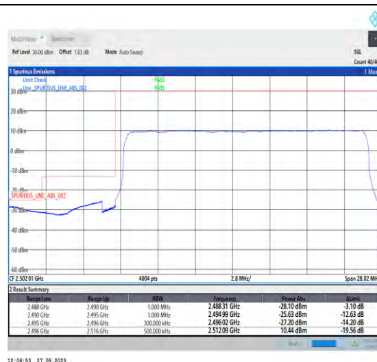
1-N41-PC3-30-20-L-3-DFT-PI2BPSK-Outer_Full-50@0-1--PASS-see graph
