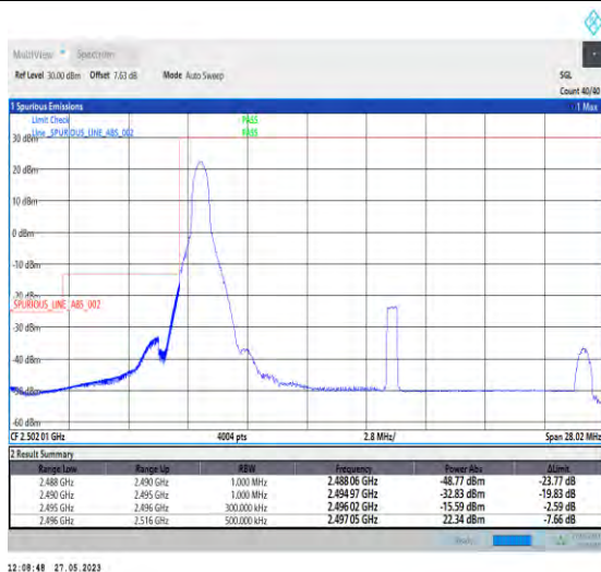
1-N41-PC3-30-20-L-4-CP-QPSK-Edge_1RB_Left-1@0-1--PASS-see graph
