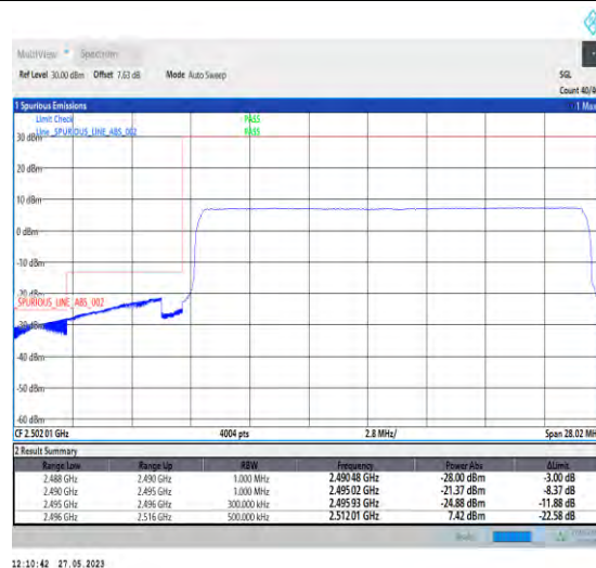
1-N41-PC3-30-20-L-6-CP-QPSK-Outer_Full-51@0-1--PASS-see graph
