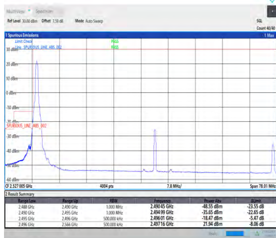
1-N41-PC3-30-70-L-1-DFT-PI2BPSK-Edge_1RB_Left -1@0-1--PASS-see graph
