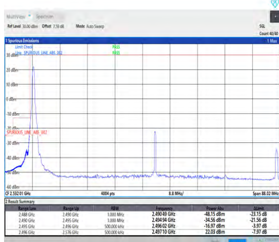
1-N41-PC3-30-80-L-4-CP-QPSK-Edge_1RB_Left-1@ 0-1--PASS-see graph
