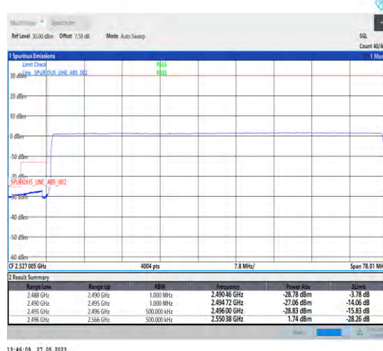
1-N41-PC3-30-70-L-6-CP-QPSK-Outer_Full-189@ 0-1--PASS-see graph
