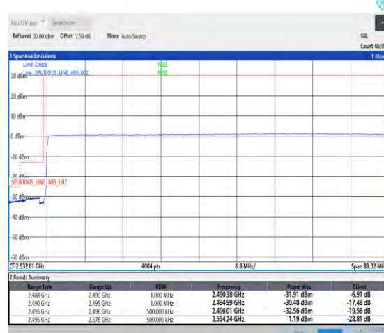
1-N41-PC3-30-80-L-6-CP-QPSK-Outer_Full-217@ 0-1--PASS-see graph
