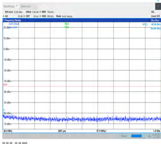
1-N41-PC3-30-100-M-1-N/A-DFT-PI2BPSK-Inner_1 RB_Left-1@1-30-1000-36.31--60.39--35-PASS
