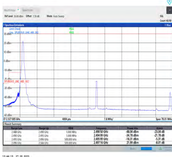
1-N41-PC3-30-70-L-4-CP-QPSK-Edge_1RB_Left-1@ 0-1--PASS-see graph
