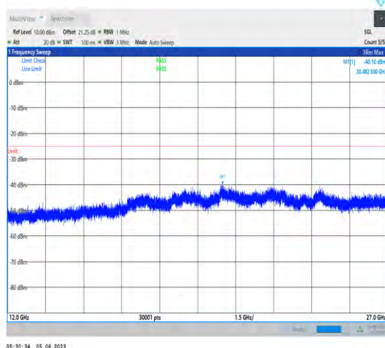
1-N41-PC3-30-100-M-1-N/A-DFT-PI2BPSK-Inner_1R B_Left-1@1-12000-27000-20482.50--40.10--25-PAS
