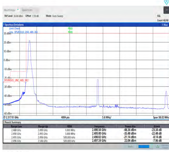
1-N41-PC3-30-50-L-4-CP-QPSK-Edge_1RB_Left-1@ 0-1--PASS-see graph
