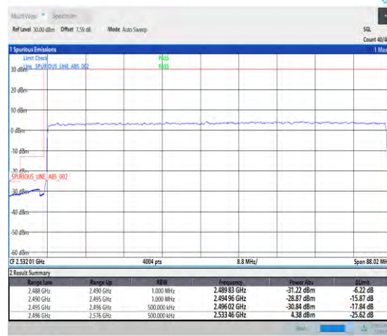
1-N41-PC3-30-80-L-3-DFT-PI2BPSK-Outer_Full-21 6@0-1--PASS-see graph
