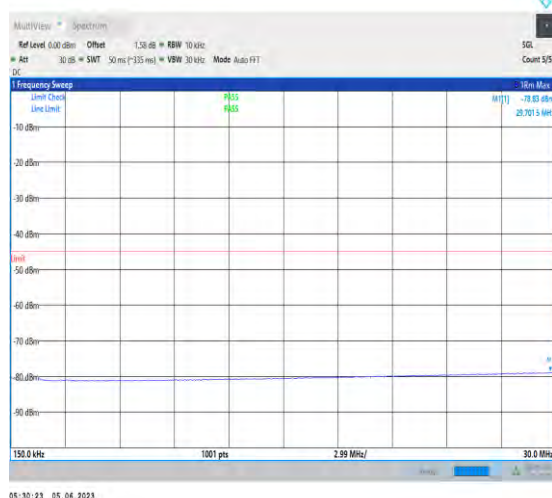
1-N41-PC3-30-100-M-1-N/A-DFT-PI2BPSK-Inner_1R B_Left-1@1-0.15-30-29.70--78.83--45-PASS
