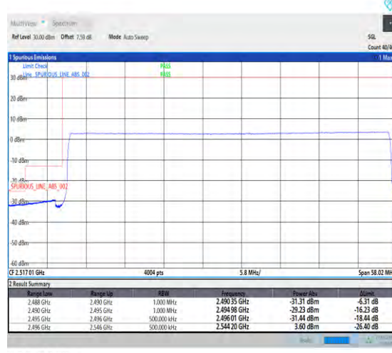
1-N41-PC3-30-50-L-6-CP-QPSK-Outer_Full-133@ 0-1--PASS-see graph
