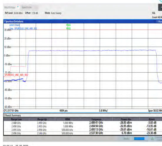
1-N41-PC3-30-50-L-3-DFT-PI2BPSK-Outer_Full-12 8@0-1--PASS-see graph
