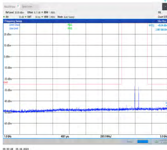
1-N41-PC3-30-100-M-1-N/A-DFT-PI2BPSK-Inner_1R B_Left-1@1-1000-3000-2981.50--45.04--25-PASS
