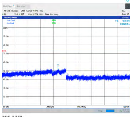
1-N41-PC3-30-100-M-1-N/A-DFT-PI2BPSK-Inner_1 RB_Left-1@1-3000-12000-6920.40--46.56--25-PAS
