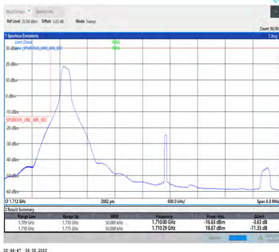
1-N66-PC3-15-5-L-1-DFT-PI2BPSK-Edge_1RB_Left-1 @0-1-seegraph-PASS-see graph
