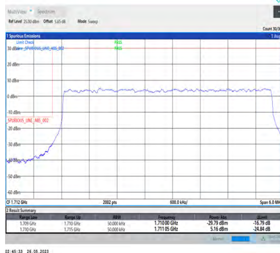
1-N66-PC3-15-5-L-3-DFT-PI2BPSK-Outer_Full-25 @0-1-seegraph-PASS-see graph
