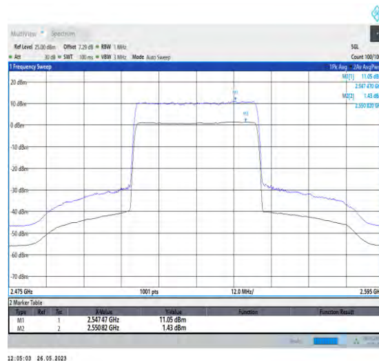
1-N7-PC3-15-40-M-2-CP-256QAM-Outer_Full-216 @0-9.62-100%-0.00-9.62-PASS-≤13
