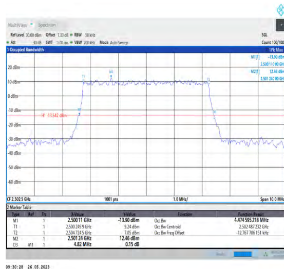
1-N7-PC3-15-5-L-4-DFT-64QAM-Outer_Full-25@0-4. .475-4.820-≤5-PASS
