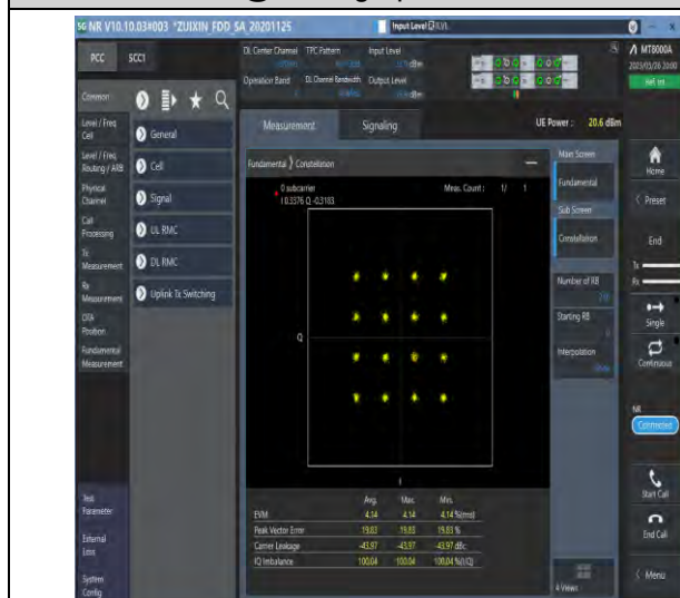
1-N7-PC3-15-40-M-7-CP-16QAM-Outer_Full-216@0- see graph-PASS
