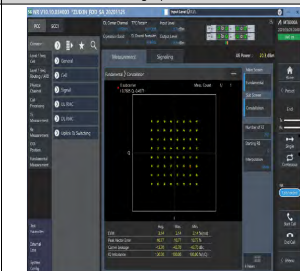
1-N7-PC3-15-40-M-8-CP-64QAM-Outer_Full-216@ 0-see graph-PASS
