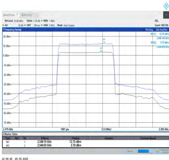
1-N7-PC3-15-40-M-1-DFT-256QAM-Outer_Full-216 @0-9.05-100%-0.00-9.05-PASS-≤13
