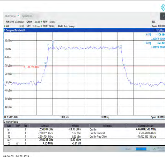
1-N7-PC3-15-5-L-2-DFT-PI2BPSK-Outer_Full-25@0-4. 469-4.850-≤5-PASS
