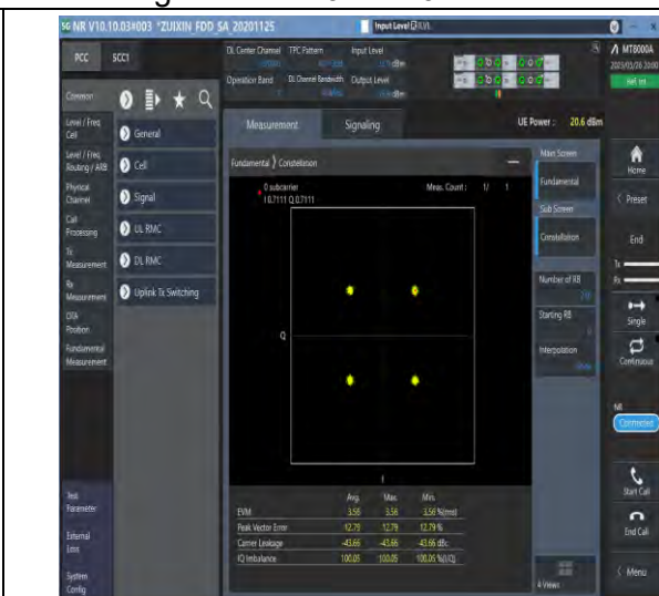
1-N7-PC3-15-40-M-6-CP-QPSK-Outer_Full-216@0- see graph-PASS
