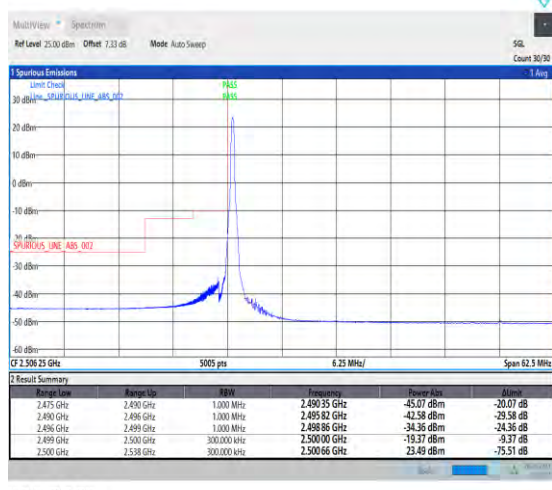
1-N7-PC3-15-25-L-1-DFT-PI2BPSK-Edge_1RB_Left-1@0-1--PASS-see graph
