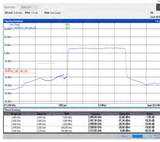
1-N7-PC3-15-20-L-3-DFT-PI2BPSK-Outer_Full-100@0-1--PASS-see graph
