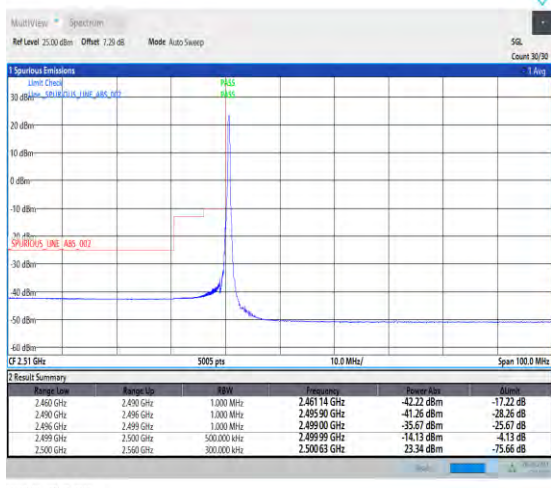
1-N7-PC3-15-40-L-1-DFT-PI2BPSK-Edge_1RB_Left-1@0-1--PASS-see graph
