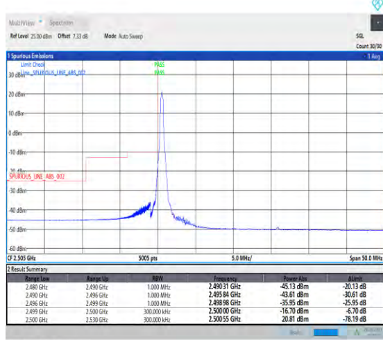
1-N7-PC3-15-20-L-4-CP-QPSK-Edge_1RB_Left-1@0-1--PASS-see graph
