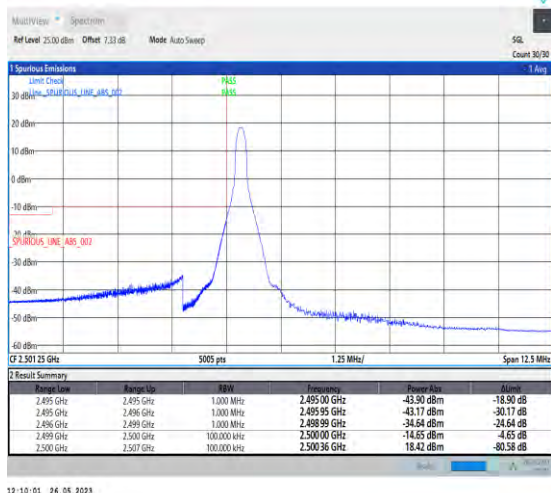
1-N7-PC3-15-5-L-4-CP-QPSK-Edge_1RB_Left-1@0-1--PASS-see graph
