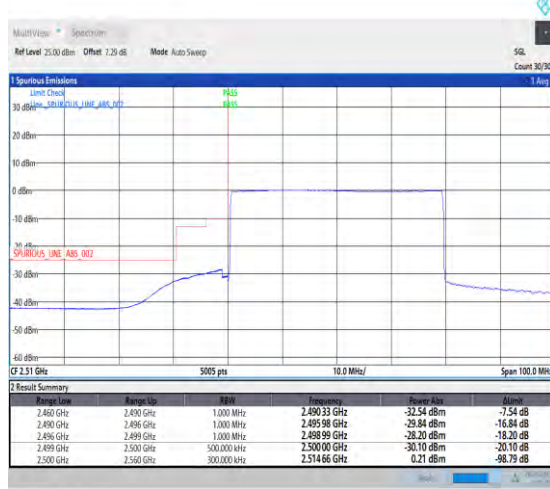
1-N7-PC3-15-40-L-6-CP-QPSK-Outer_Full-216@0-1--PASS-see graph
