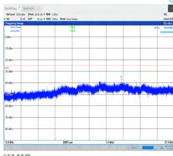
1-N7-PC3-15-40-M-1-N/A-DFT-PI2BPSK-Inner_1RB_ Left-1@1-12000-27000-22345.00--38.09--25-PASS
