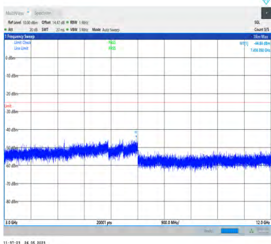
1-N7-PC3-15-40-M-1-N/A-DFT-PI2BPSK-Inner_1RB _Left-1@1-3000-12000-7456.35--44.84--25-PASS
