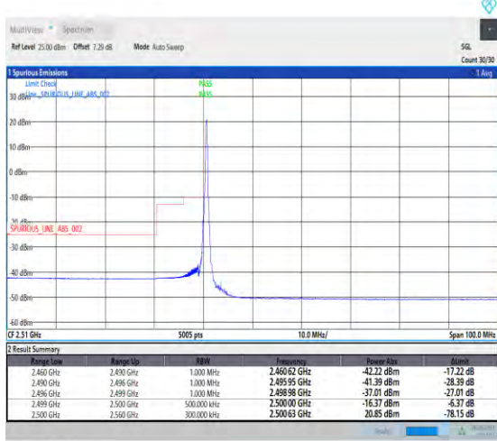
1-N7-PC3-15-40-L-4-CP-QPSK-Edge_1RB_Left-1@0-1--PASS-see graph
