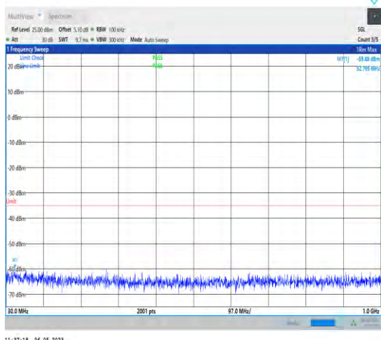
1-N7-PC3-15-40-M-1-N/A-DFT-PI2BPSK-Inner_1RB _Left-1@1-30-1000-52.80--59.88--35-PASS
