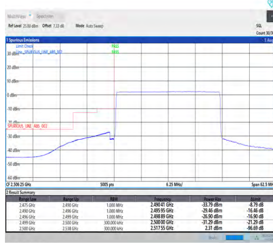
1-N7-PC3-15-25-L-6-CP-QPSK-Outer_Full-133@0-1--PASS-see graph
