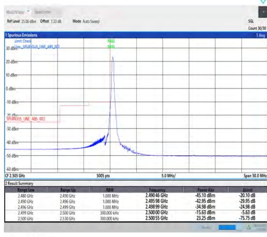
1-N7-PC3-15-20-L-1-DFT-PI2BPSK-Edge_1RB_Left-1@0-1--PASS-see graph
