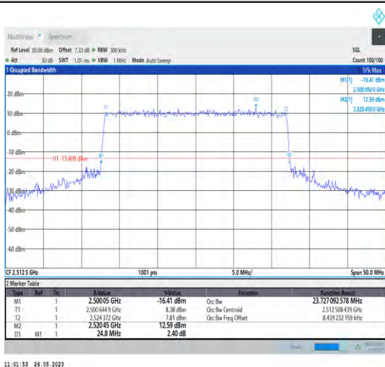
1-N7-PC3-15-25-L-7-CP-16QAM-Out_133@0-23.727-24.800-≤25-PASS
