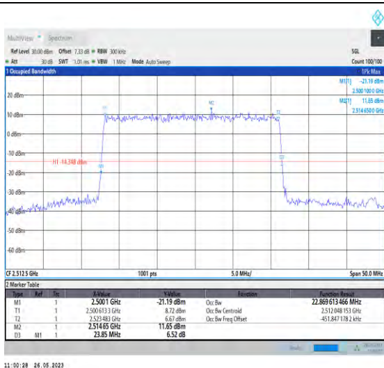
1-N7-PC3-15-25-L-5-DFT-256QAM-Out_128@0-22.87-23.850-≤25-PASS
