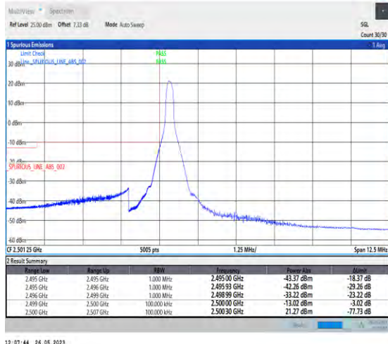
1-N7-PC3-15-5-L-1-DFT-PI2BPSK-Edge_1RB_Left-1@0-1--PASS-see graph
