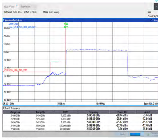
1-N7-PC3-15-40-L-3-DFT-PI2BPSK-Outer_Full-216@0-1--PASS-see graph
