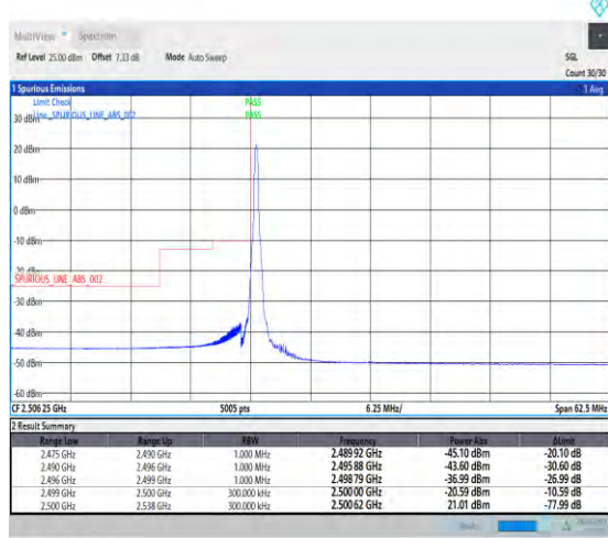
1-N7-PC3-15-25-L-4-CP-QPSK-Edge_1RB_Left-1@0-1--PASS-see graph
