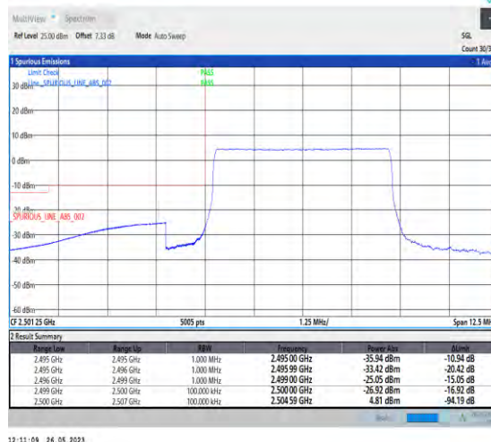
1-N7-PC3-15-5-L-6-CP-QPSK-Outer_Full-25@0-1--PASS-see graph
