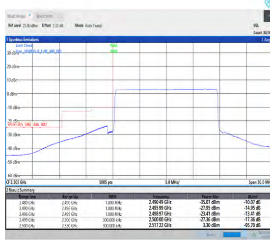
1-N7-PC3-15-20-L-6-CP-QPSK-Outer_Full-106@0-1--PASS-see graph
