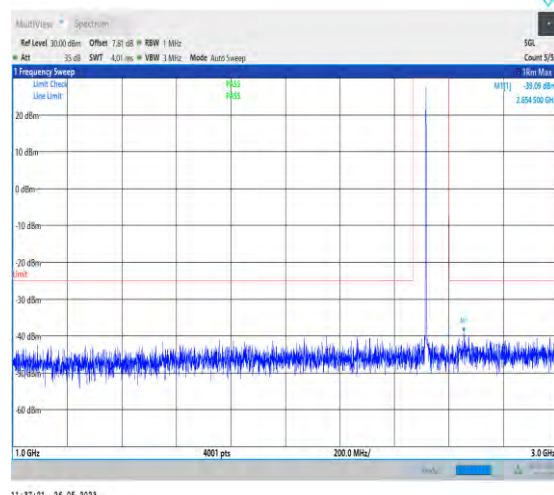
1-N7-PC3-15-40-M-1-N/A-DFT-PI2BPSK-Inner_1RB_ Left-1@1-1000-3000-2654.50--39.09--25-PASS
