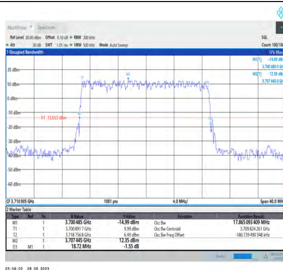
1-N77-3700-3980-PC3-30-20-L-2-DFT-PI2BPSK-Out_ Full-50@0-17.865-18.720-≤20-PASS
