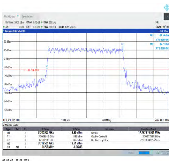
1-N77-3700-3980-PC3-30-20-L-1-DFT-QPSK-Out_ Full-50@0-17.768-18.560-≤20-PASS
