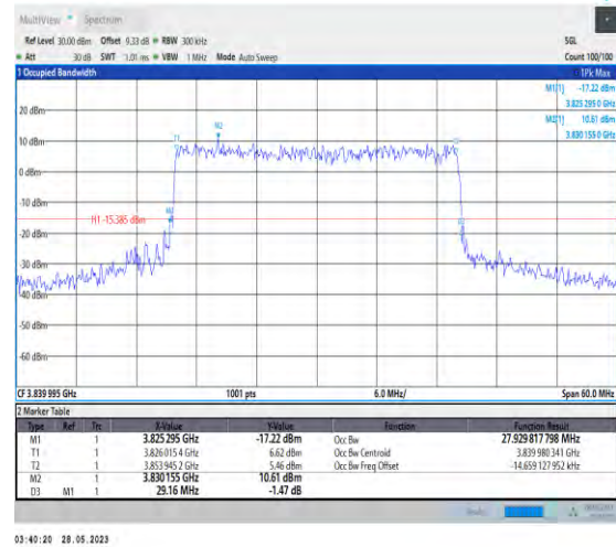
1-N77-3700-3980-PC3-30-30-M-8-CP-64QAM-Outer_Full-78@0-27.93-29.160-≤30-PASS
