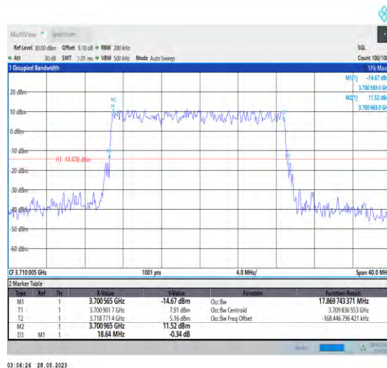
1-N77-3700-3980-PC3-30-20-L-4-DFT-64QAM-Out_ Full-50@0-17.87-18.640-≤20-PASS
