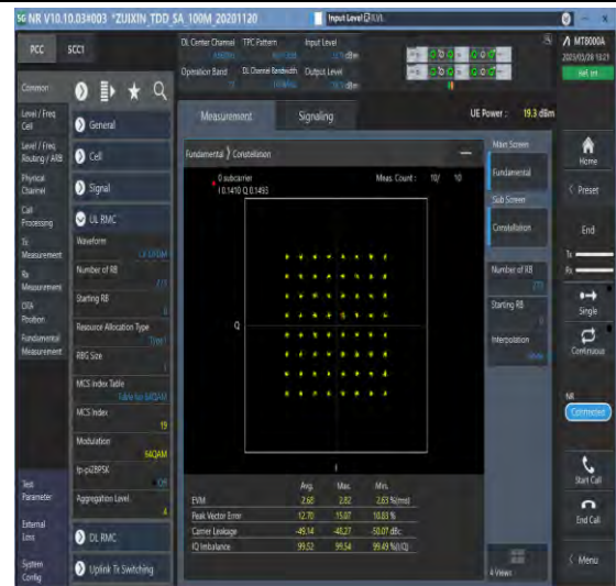
1-N77-3700-3980-PC3-30-100-M-8-CP-64QAM-Outer_Full-273@0-see graph-PASS
