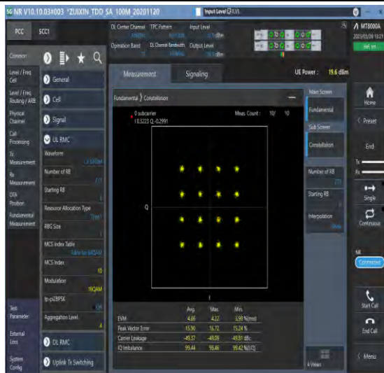
1-N77-3700-3980-PC3-30-100-M-7-CP-16QAM-Outer_Full-273@0-see graph-PASS
