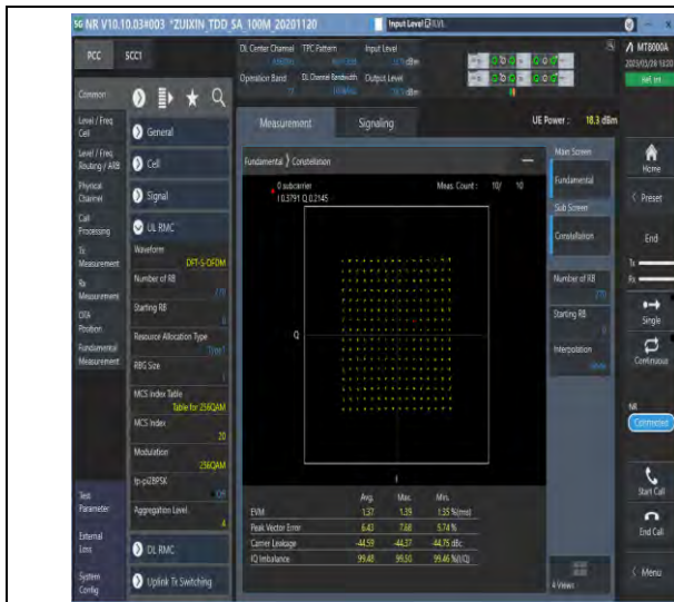
1-N77-3700-3980-PC3-30-100-M-5-DFT-256QAM-Outer_Full-270@0-see graph-PASS
