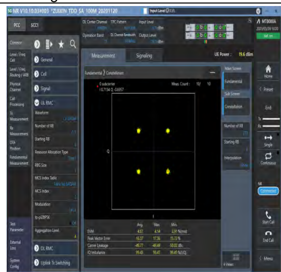
1-N77-3700-3980-PC3-30-100-M-6-CP-QPSK-Outer_Full-273@0-see graph-PASS
