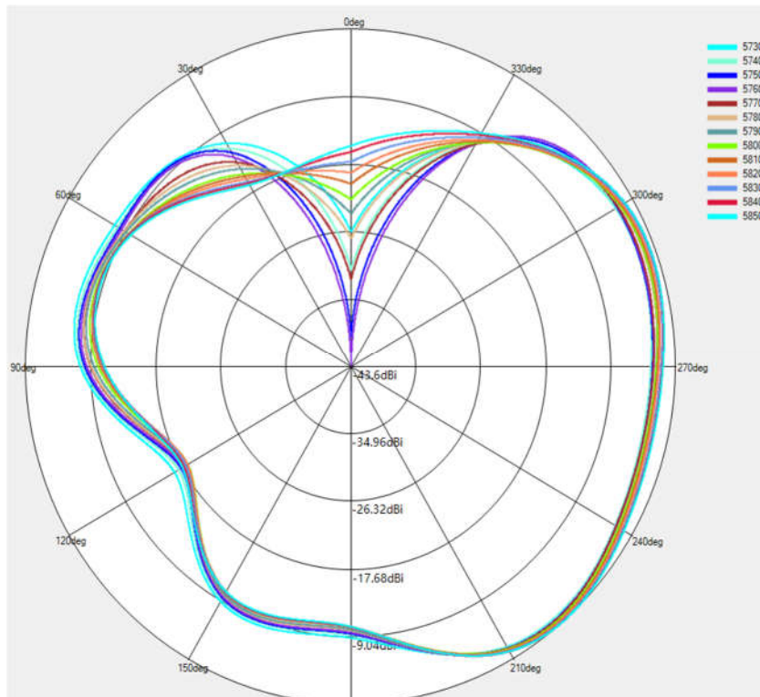
(18) X-Z Plane(unit:dBi):
