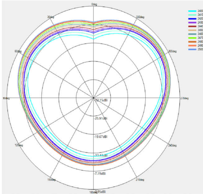
(2) X-Z Plane(unit:dBi):
