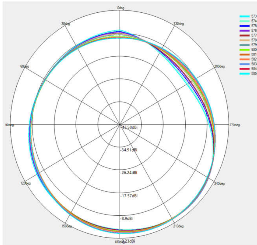
(18) X-Z Plane(unit:dBi):
