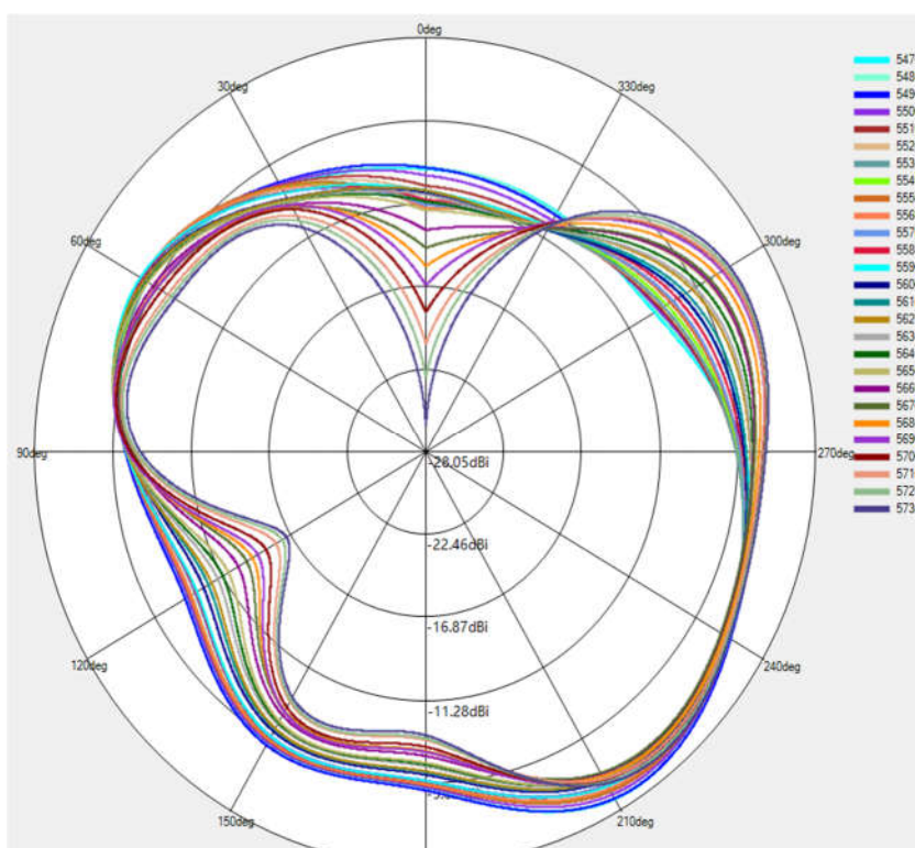
(14) X-Z Plane(unit:dBi):
