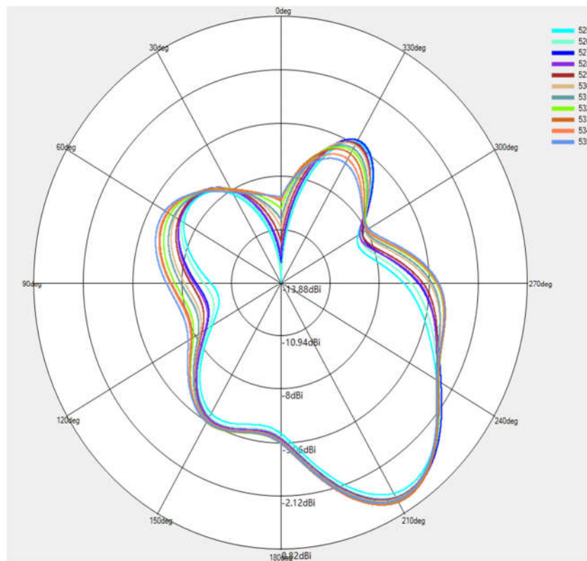
(10) X-Z Plane(unit:dBi):
