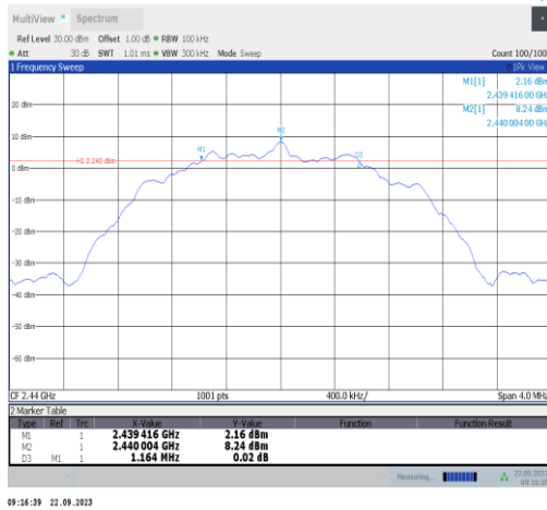
BLE_2M-Ant22-2440-PASS
