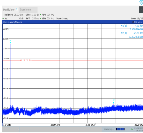
BLE_2M-Ant22-2440-1000~26500-PASS
