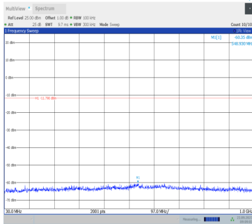
BLE_1M-Ant22-2440-30~1000-PASS
