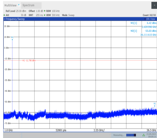
BLE_1M-Ant22-2440-1000~26500-PASS
