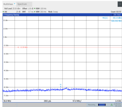
BLE_1M-Ant22-2480-30~1000-PASS
