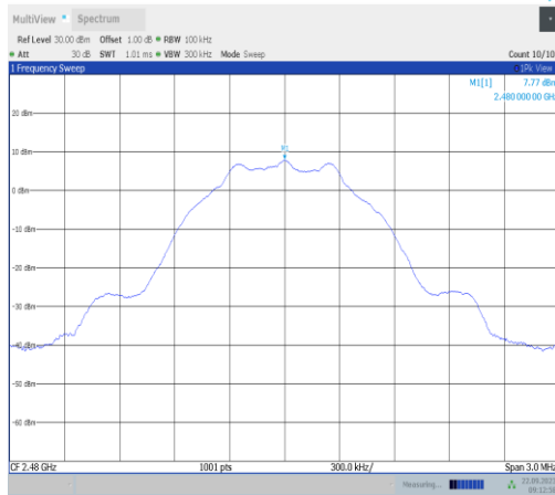
BLE_1M-Ant22-2480-0~Reference-PASS
