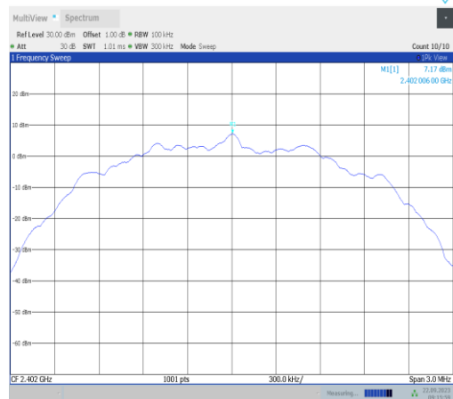
BLE_2M-Ant22-2402-0~Reference-PASS
