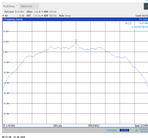
BLE_2M-Ant22-2440-0~Reference-PASS
