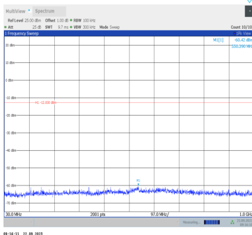
BLE_2M-Ant22-2402-30~1000-PASS
