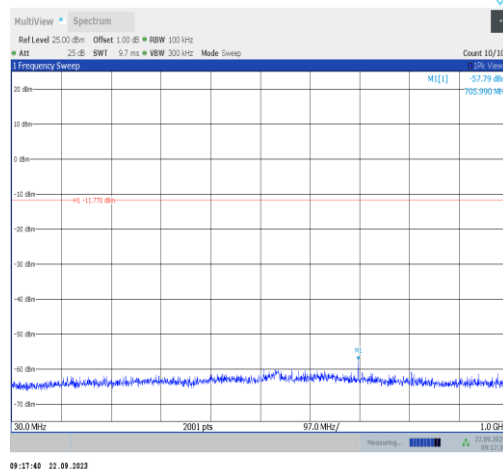
BLE_2M-Ant22-2440-30~1000-PASS
