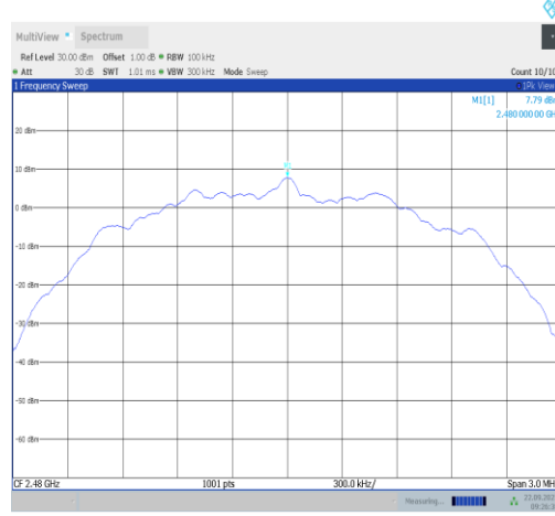
BLE_2M-Ant22-2480-0~Reference-PASS
