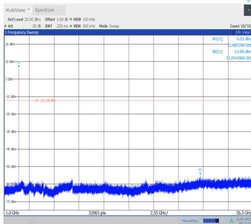
BLE_1M-Ant22-2480-1000~26500-PASS
