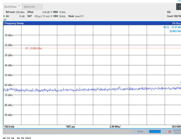
Band17-10MHz-QPSK-23780-1RB#0-Range2:0.15~30MHz
