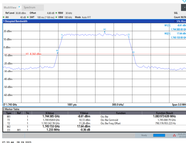
Band66-1.4MHz-16QAM-132322-6RB#0
