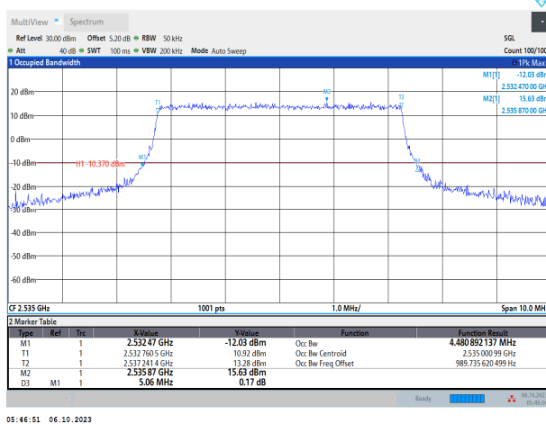
Band7-5MHz-16QAM-21100-25RB#0
