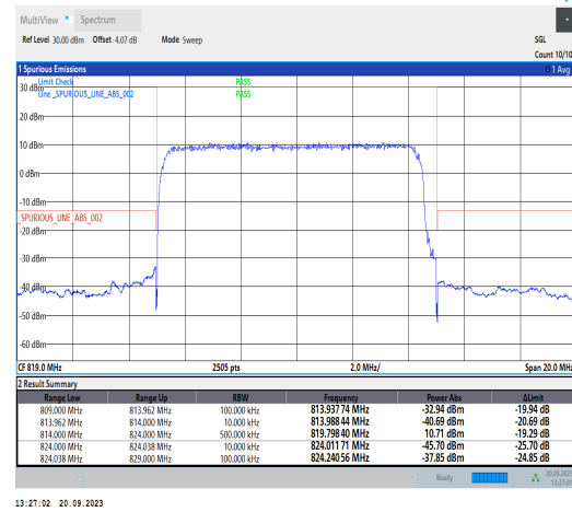
1-N26-814-824-PC3-15-10-H-3-DFT-PI2BPSK-Out er_Full-50@0-Ant41-1--PASS-see graph
