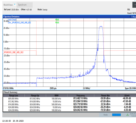
1-N26-814-824-PC3-15-10-H-2-DFT-PI2BPSK-Edge_1 RB_Right-1@51-Ant41-1--PASS-see graph
