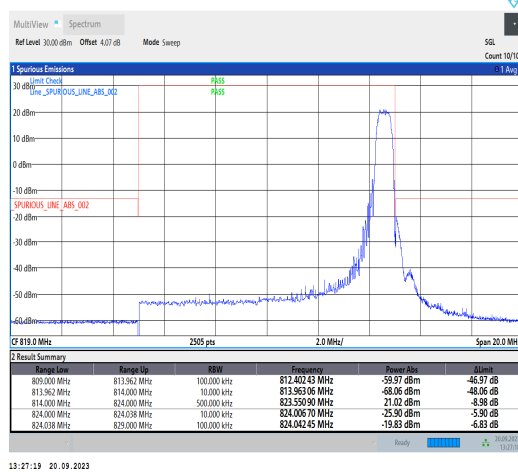
1-N26-814-824-PC3-15-10-H-5-CP-QPSK-Edge_1RB_1 Right-1@51-Ant41-1--PASS-see graph
