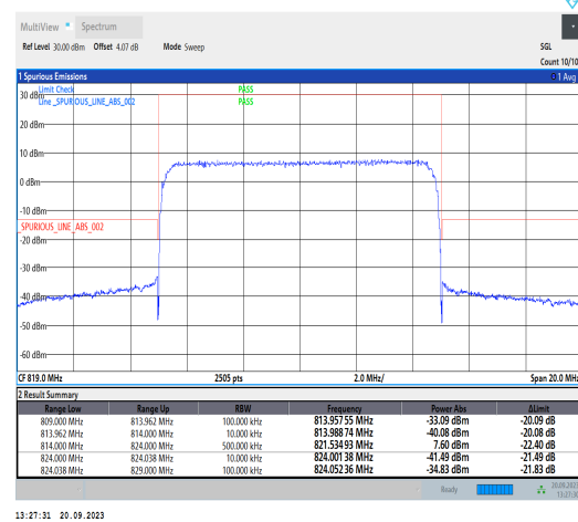
1-N26-814-824-PC3-15-10-H-6-CP-QPSK-Outer_1 Full-52@0-Ant41-1--PASS-see graph
