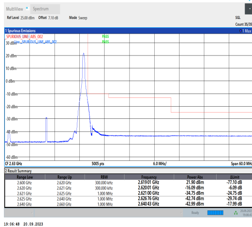
1-N38-PC3-30-20-H-2-DFT-PI2BPSK-Edge_1RB_Righ t1@50-Ant11-1--PASS-see graph
