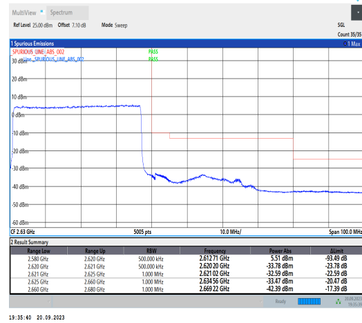
1-N38-PC3-30-40-H-3-DFT-PI2BPSK-Outer_Full-1 00@0-Ant11-1--PASS-see graph
