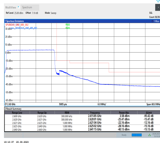
1-N38-PC3-30-20-H-6-CP-QPSK-Outer_Full-51@ 0-Ant11-1--PASS-see graph
