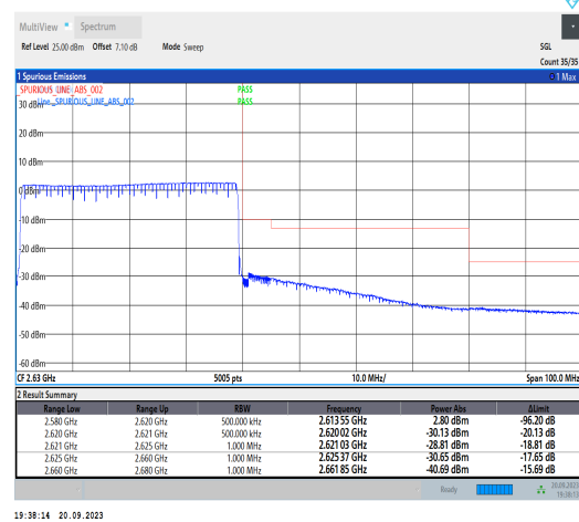
1-N38-PC3-30-40-H-6-CP-QPSK-Outer_Full-106 @0-Ant11-1--PASS-see graph
