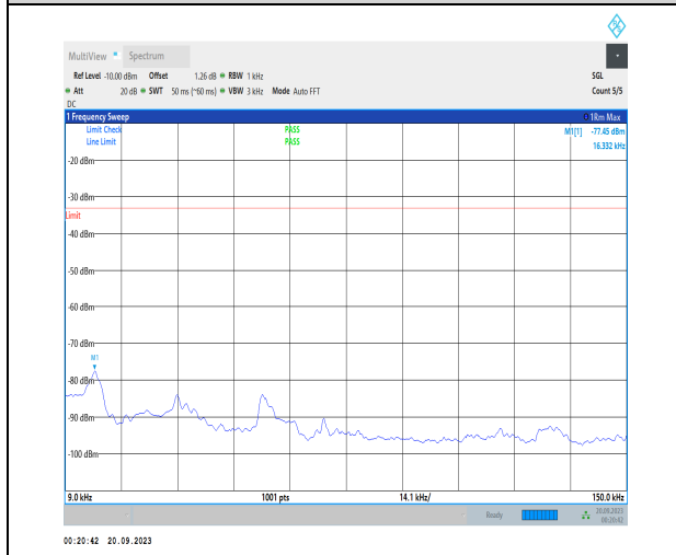
1-N5-PC3-15-20-H-1-DFT-PI2BPSK-Inner_1RB_Left -1@1-0.009-0.15-Ant41-0.16--77.45--33-PASS
