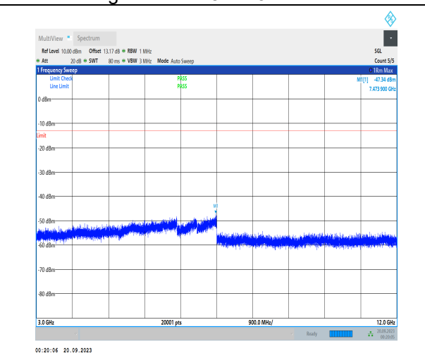
1-N5-PC3-15-20-M-1-DFT-PI2BPSK-Inner_1RB_Left -1@1-3000-12000-Ant41-7473.90--47.34--13-PASS
