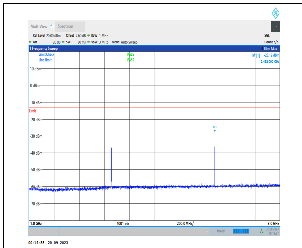
1-N5-PC3-15-20-M-1-DFT-PI2BPSK-Inner_1RB_Left -1@1-1000-3000-Ant41-2482.00--28.12--13-PASS
