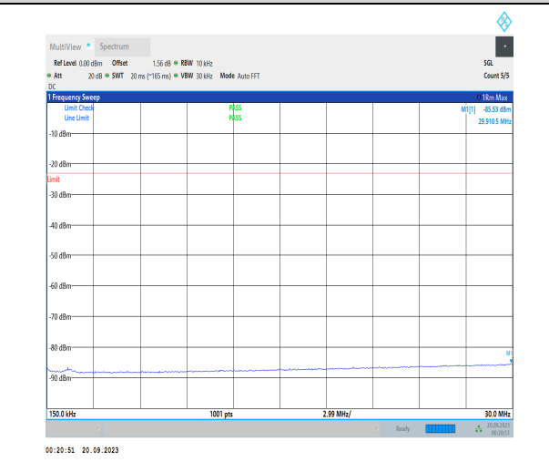
1-N5-PC3-15-20-H-1-DFT-PI2BPSK-Inner_1RB_Left -1@1-0.15-30-Ant41-29.91--85.53--23-PASS
