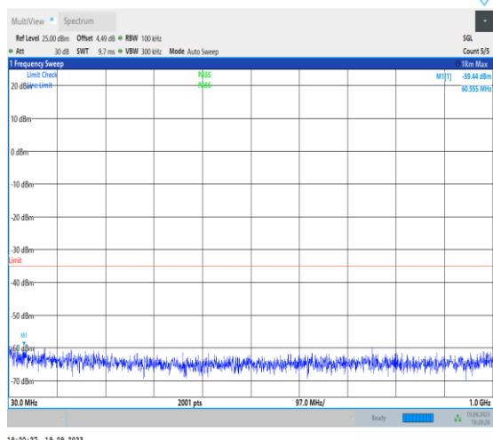
1-N7-PC3-15-40-M-1-DFT-PI2BPSK-Inner_1RB_Lef t-1@1-30-1000-Ant31-60.56--59.44--35-PASS
