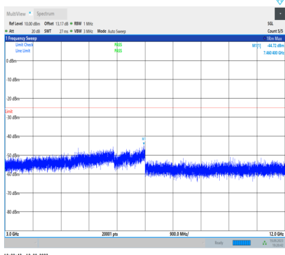
1-N7-PC3-15-40-M-1-DFT-PI2BPSK-Inner_1RB_Lef t-1@1-3000-12000-Ant317460.40--44.72--25-PASS
