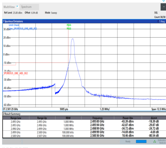
1-N7-PC3-15-5-L-4-CP-QPSK-Edge_1RB_Left-1@0-A nt31-1--PASS-see graph
