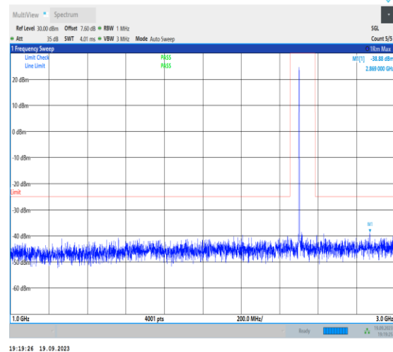
1-N7-PC3-15-40-L-1-DFT-PI2BPSK-Inner_1RB_Left- 1@1-1000-3000-Ant31-2889.00--38.88--25-PASS
