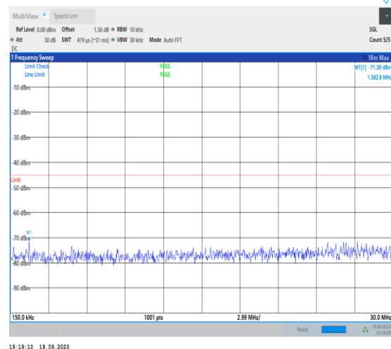
1-N7-PC3-15-40-L-1-DFT-PI2BPSK-Inner_1RB_Left- 1@1-0.15-30-Ant31-1.58--71.39--45-PASS
