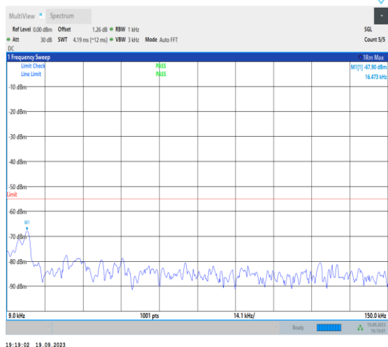
1-N7-PC3-15-40-L-1-DFT-PI2BPSK-Inner_1RB_Left -1@1-0.009-0.15-Ant31-0.16--67.90--55-PASS
