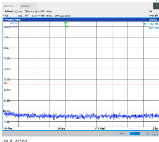
1-N7-PC3-15-40-L-1-DFT-PI2BPSK-Inner_1RB_Left -1@1-30-1000-Ant31-31.98--58.24--35-PASS
