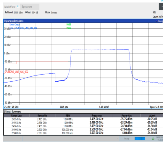
1-N7-PC3-15-5-L-6-CP-QPSK-Outer_Full-25@0-A nt31-1--PASS-see graph
