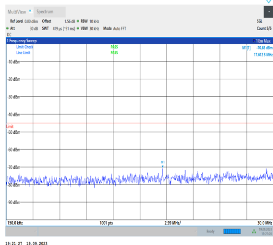
1-N7-PC3-15-40-H-1-DFT-PI2BPSK-Inner_1RB_Left- 1@1-0.15-30-Ant31-17.61--70.63--45-PASS
