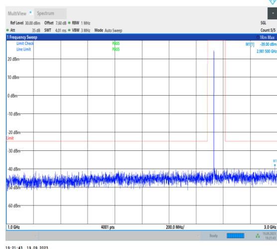
1-N7-PC3-15-40-H-1-DFT-PI2BPSK-Inner_1RB_Left- 1@1-1000-3000-Ant31-2981.50--39.00--25-PASS
