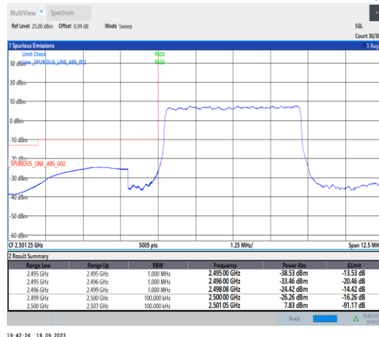
1-N7-PC3-15-5-L-3-DFT-PI2BPSK-Outer_Full-25 @0-Ant31-1--PASS-see graph
