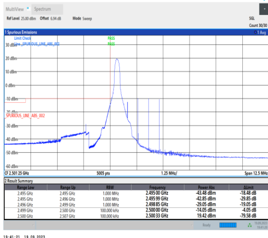
1-N7-PC3-15-5-L-1-DFT-PI2BPSK-Edge_1RB_Left-1 @0-Ant31-1--PASS-see graph
