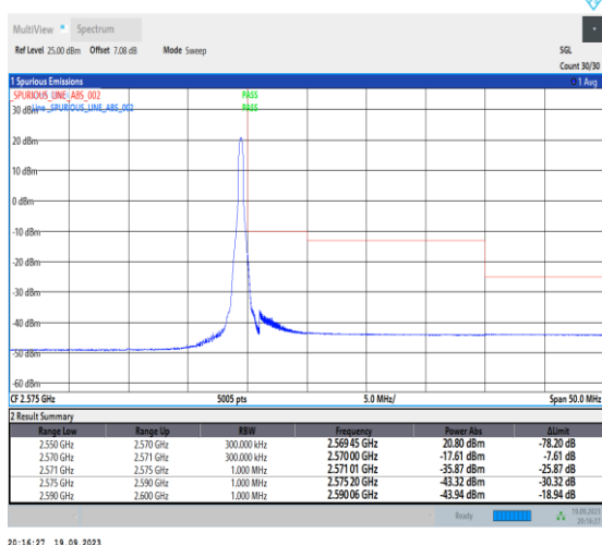
1-N7-PC3-15-20-H-5-CP-QPSK-Edge_1RB_Right-1@105-Ant31-1--PASS-see graph
