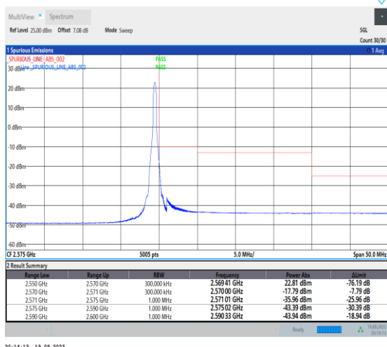
1-N7-PC3-15-20-H-2-DFT-PI2BPSK-Edge_1RB_Right-1@105-Ant31-1--PASS-see graph
