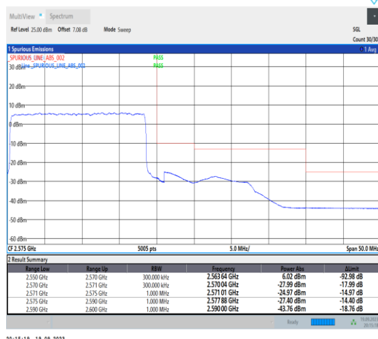
1-N7-PC3-15-20-H-3-DFT-PI2BPSK-Outer_Full-100@0-Ant31-1--PASS-see graph
