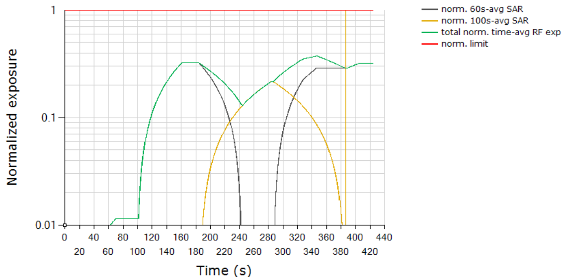
Total Normalized Time-averaged RF Exposure Tech: NR5G SUB6, Band 78 / Tech: NR5G SUB6, Band 41
