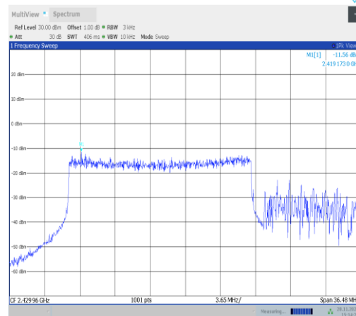
11ax40MIMO-Ant25-2437-242Tone-RU61-PASS
