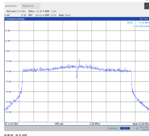
11ax20MIMO-Ant25-2412-PASS
