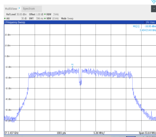
11VHT40MIMO-Ant25-2437-PASS
