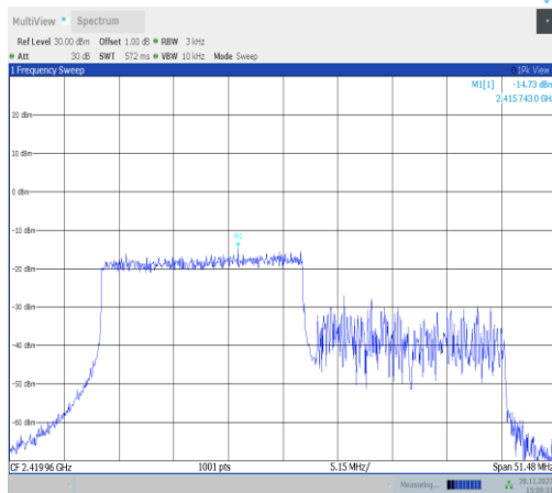
11ax40MIMO-Ant22-2422-242Tone-RU61-PASS
