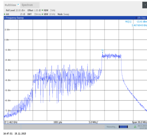
11ax20MIMO-Ant22-2462-52Tone-RU40-PASS
