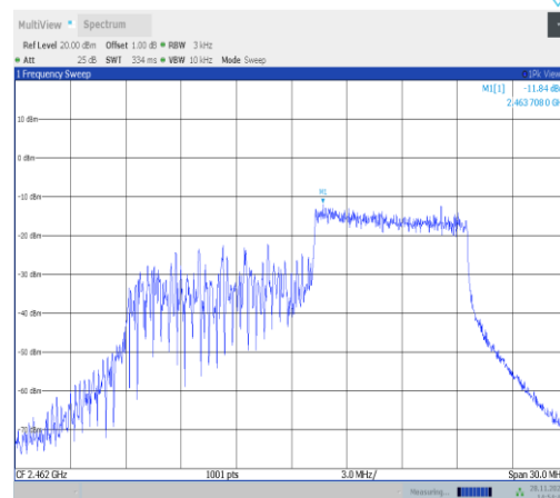
11ax20MIMO-Ant25-2462-106Tone-RU54-PASS
