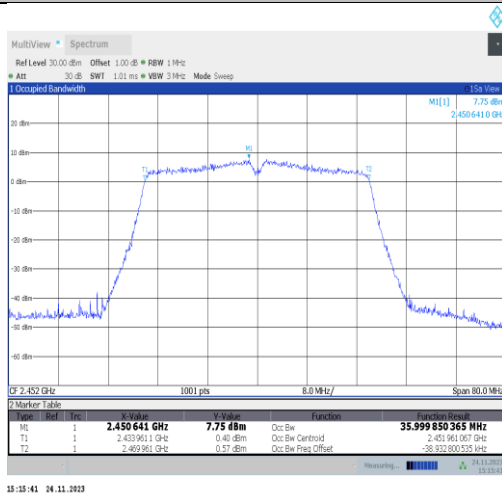
11VHT40MIMO-Ant22-2452
