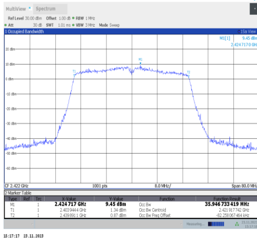
11VHT40MIMO-Ant22-2422
