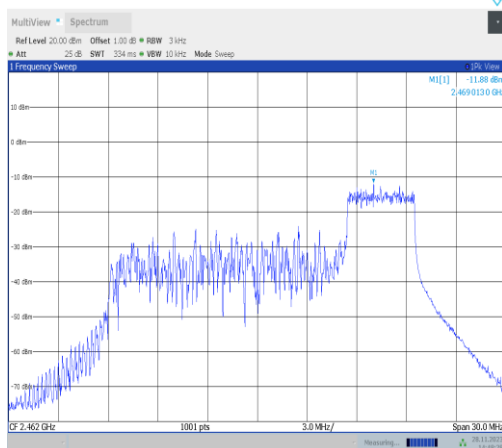
11ax20MIMO-Ant25-2462-52Tone-RU40-PASS
