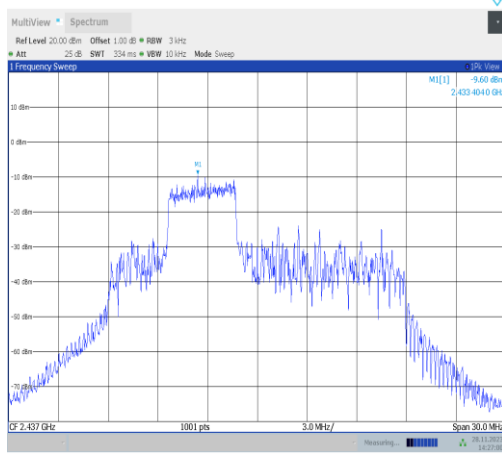
11ax20MIMO-Ant25-2437-52Tone-RU38-PASS
