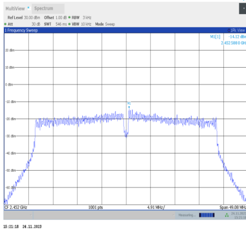
11VHT40MIMO-Ant22-2452-PASS
