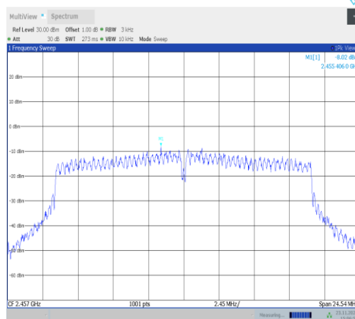
11VHT20MIMO-Ant25-2457-PASS
