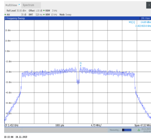
11VHT40MIMO-Ant25-2452-PASS
