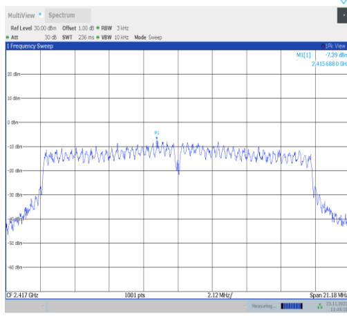
11g-CDD-Ant22-2417-PASS
