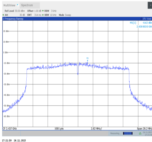
11ax20MIMO-Ant22-2437-PASS
