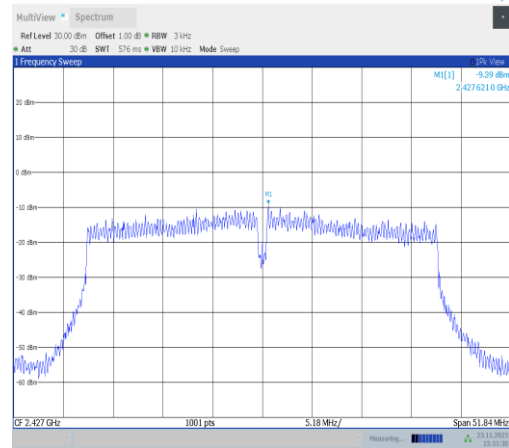
11VHT40MIMO-Ant25-2427-PASS
