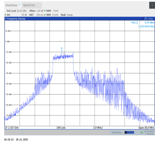
11ax20MIMO-Ant22-2437-52Tone-RU38-PASS
