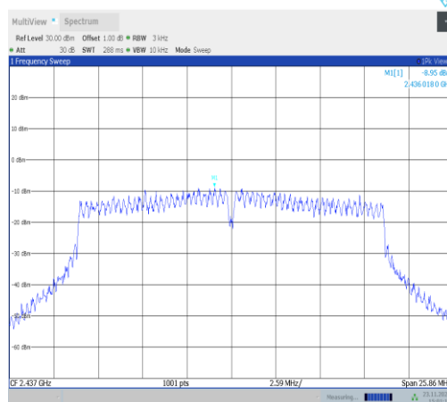
11VHT20MIMO-Ant25-2437-PASS
