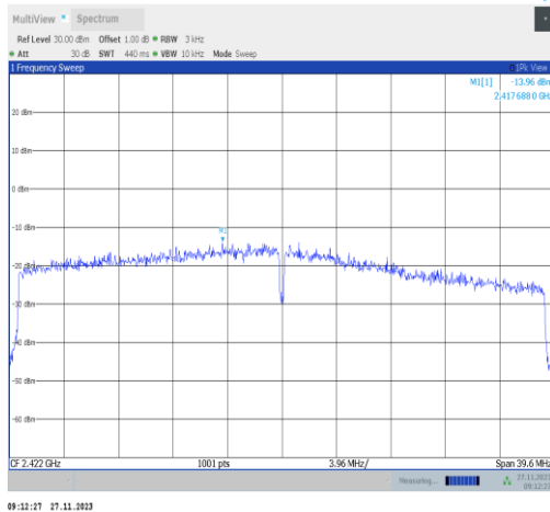
11ax40MIMO-Ant22-2422-PASS
