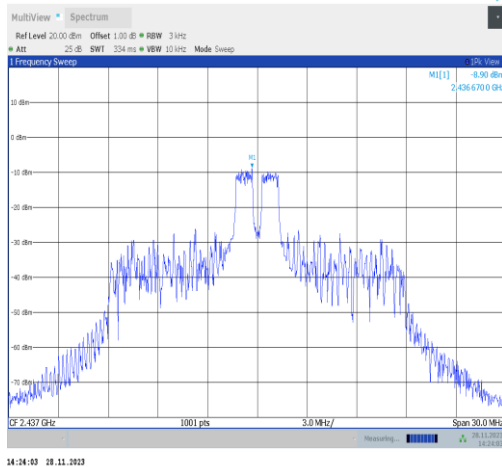
11ax20MIMO-Ant22-2437-26Tone-RU4-PASS
