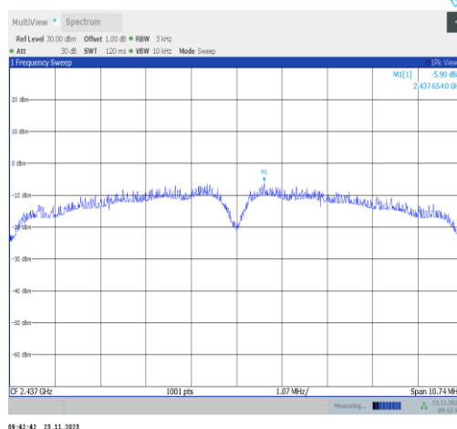
11b-CDD-Ant25-2437-PASS
