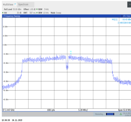
11VHT40MIMO-Ant22-2447-PASS
