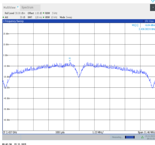
11b-CDD-Ant22-2437-PASS
