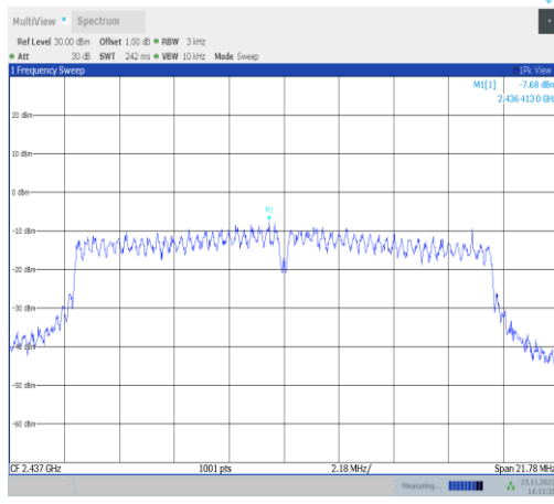
11g-CDD-Ant22-2437-PASS
