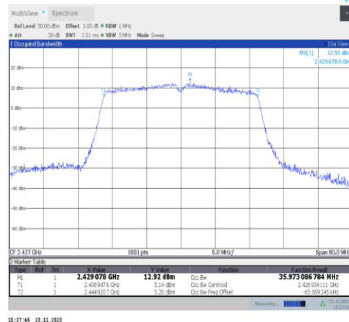
11VHT40MIMO-Ant25-2427
