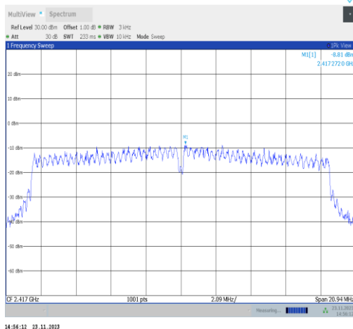
11VHT20MIMO-Ant22-2417-PASS
