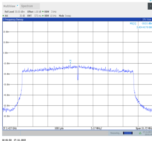
11ax40MIMO-Ant22-2427-PASS
