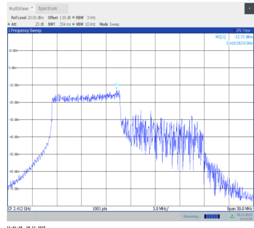
11ax20MIMO-Ant25-2412-106Tone-RU53-PASS
