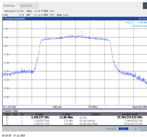
11ax40MIMO-Ant22-2447
