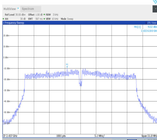
11VHT40MIMO-Ant22-2437-PASS
