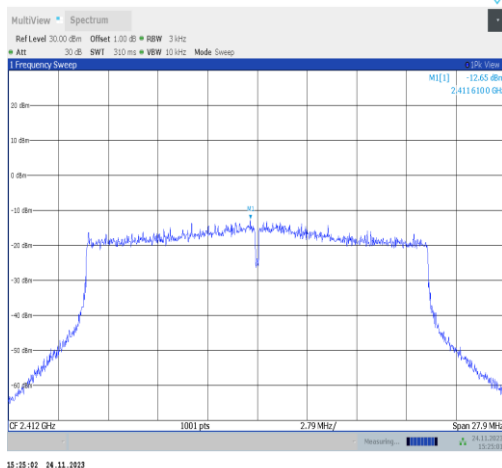
11ax20MIMO-Ant22-2412-PASS
