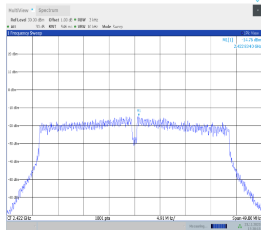
11VHT40MIMO-Ant25-2422-PASS
