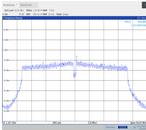
11VHT40MIMO-Ant22-2427-PASS
