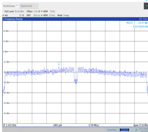
11VHT40MIMO-Ant22-2422-PASS
