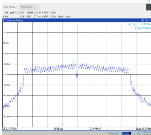
11VHT20MIMO-Ant22-2457-PASS
