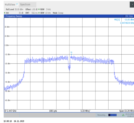
11VHT40MIMO-Ant25-2447-PASS
