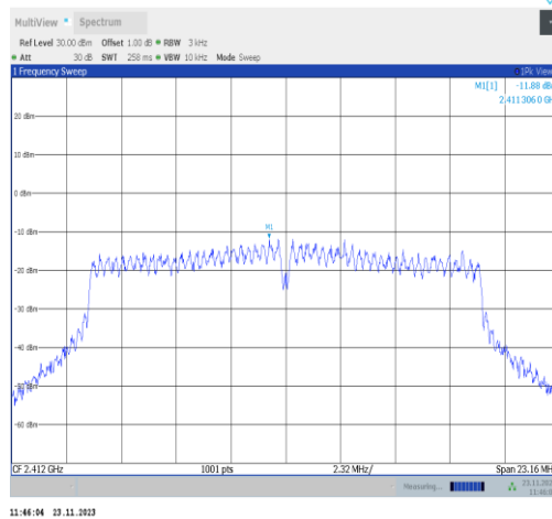
11g-CDD-Ant25-2412-PASS
