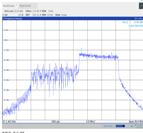
11ax20MIMO-Ant22-2462-106Tone-RU54-PASS
