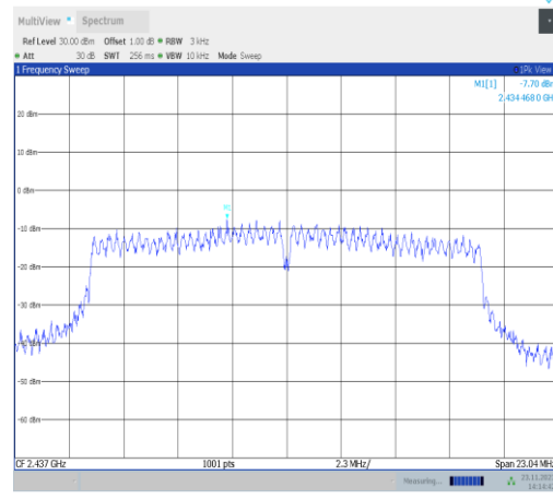
11g-CDD-Ant25-2437-PASS
