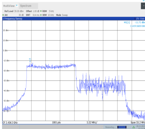
11ax40MIMO-Ant22-2437-242Tone-RU61-PASS
