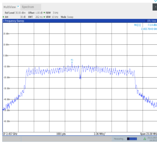
11g-CDD-Ant22-2457-PASS
