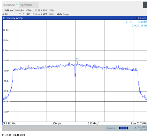
11ax20MIMO-Ant22-2462-PASS
