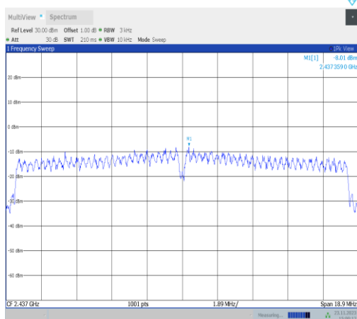
11VHT20MIMO-Ant22-2437-PASS
