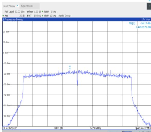
11ax40MIMO-Ant22-2452-PASS
