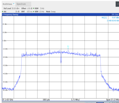
11ax40MIMO-Ant22-2437-PASS
