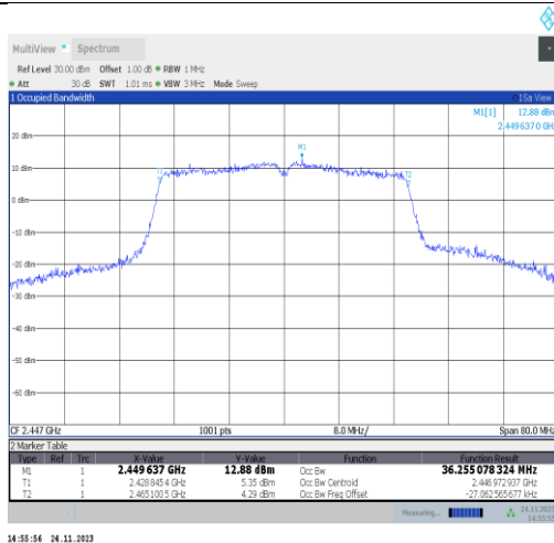
11VHT40MIMO-Ant22-2447
