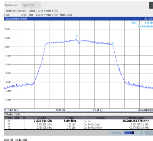
11VHT40MIMO-Ant25-2422
