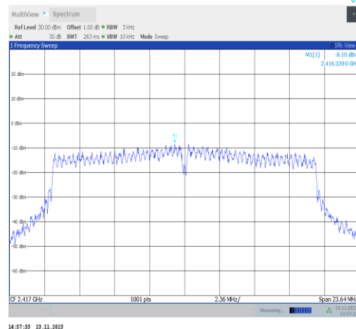
11VHT20MIMO-Ant25-2417-PASS
