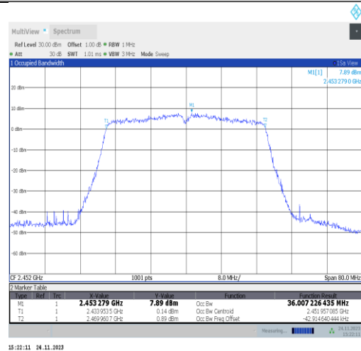
11VHT40MIMO-Ant25-2452
