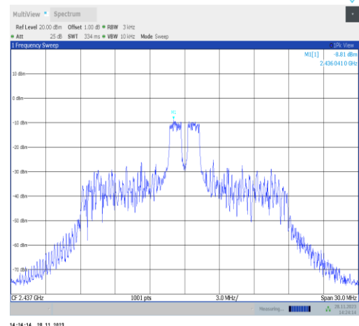
11ax20MIMO-Ant25-2437-26Tone-RU4-PASS
