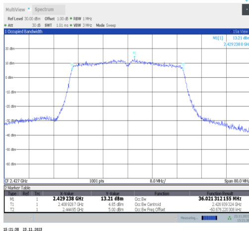
11VHT40MIMO-Ant22-2427
