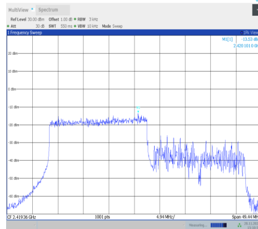
11ax40MIMO-Ant25-2422-242Tone-RU61-PASS
