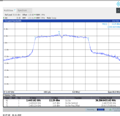
11VHT40MIMO-Ant25-2447
