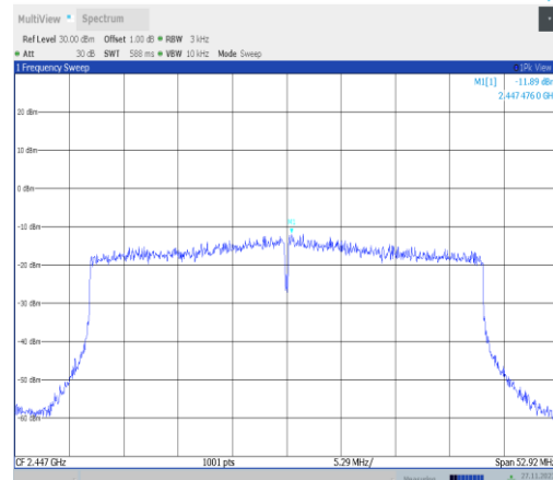
11ax40MIMO-Ant25-2447-PASS
