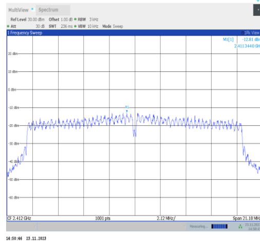
11VHT20MIMO-Ant25-2412-PASS
