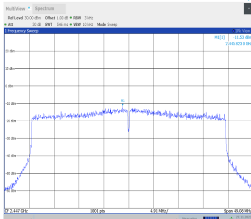
11ax40MIMO-Ant22-2447-PASS
