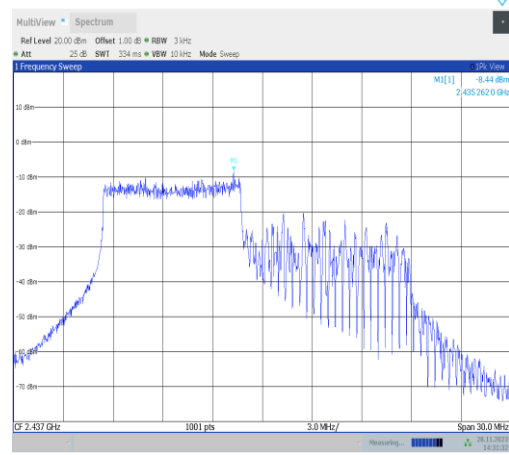
11ax20MIMO-Ant25-2437-106Tone-RU53-PASS
