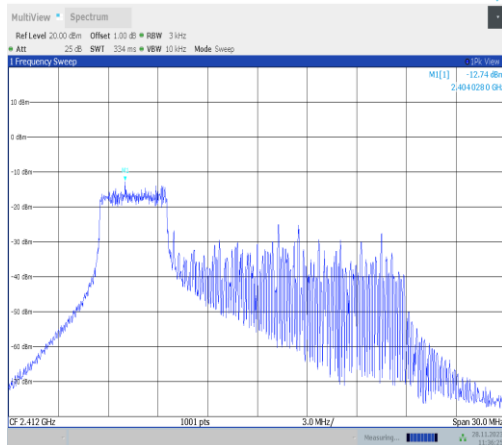
11ax20MIMO-Ant25-2412-52Tone-RU37-PASS
