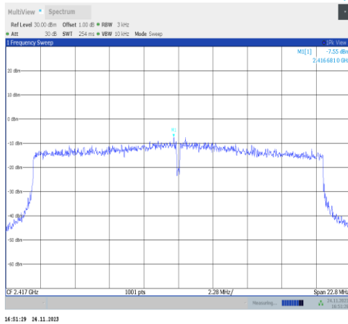
11ax20MIMO-Ant22-2417-PASS
