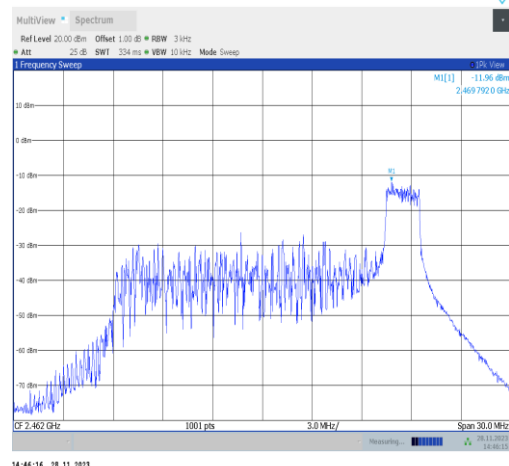
11ax20MIMO-Ant25-2462-26Tone-RU8-PASS
