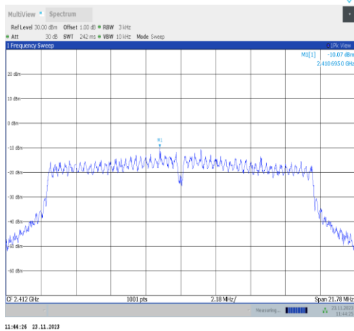
11g-CDD-Ant22-2412-PASS
