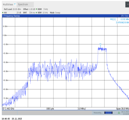
11ax20MIMO-Ant22-2462-26Tone-RU8-PASS
