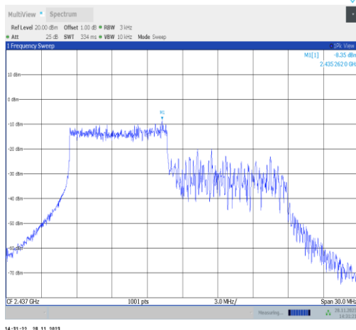
11ax20MIMO-Ant22-2437-106Tone-RU53-PASS
