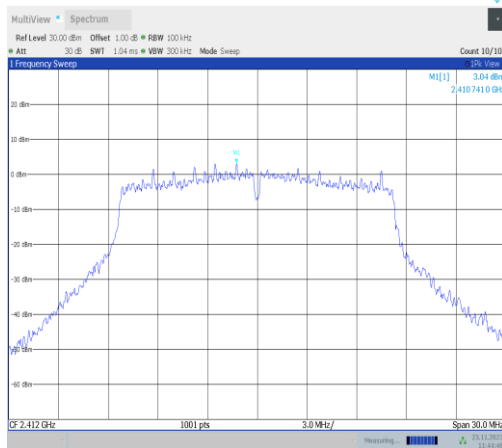
11g-CDD-Ant22-2412-0~Reference-PASS
