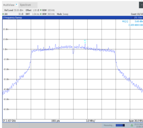
11VHT20MIMO-Ant22-2437-0~Reference-PASS
