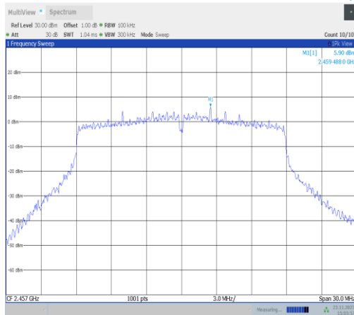
11VHT20MIMO-Ant22-2457-0~Reference-PASS
