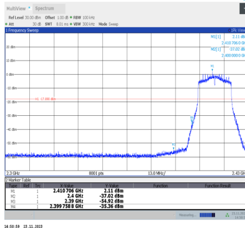
11VHT20MIMO-Ant25-2412-PASS
