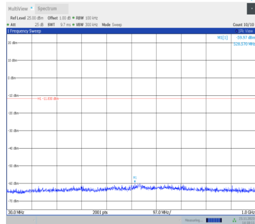
11g-CDD-Ant22-2437-30~1000-PASS
