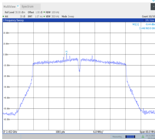
11VHT40MIMO-Ant22-2452-0~Reference-PASS
