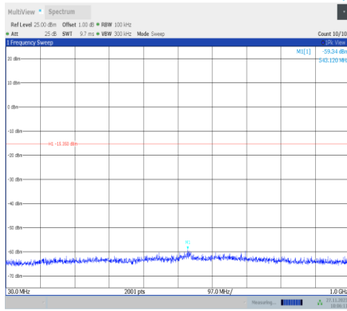
11ax40MIMO-Ant25-2427-30~1000-PASS
