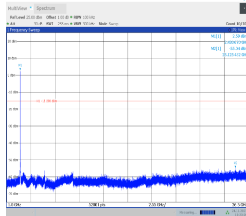
11ax20MIMO-Ant25-2437-1000~26500-PASS
