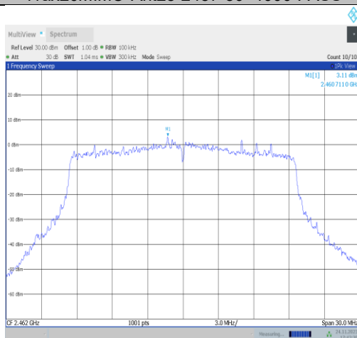
11ax20MIMO-Ant22-2462-0~Reference-PASS
