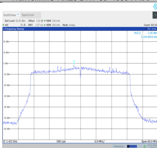
11ax40MIMO-Ant22-2452-0~Reference-PASS
