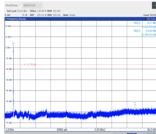
11VHT40MIMO-Ant25-2427-1000~26500-PASS
