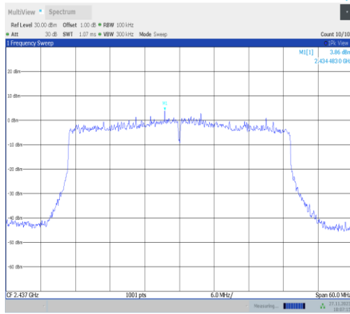
11ax40MIMO-Ant22-2437-0~Reference-PASS
