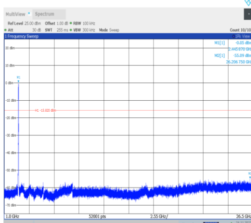
11VHT40MIMO-Ant22-2447-1000~26500-PASS
