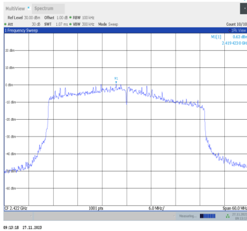
11ax40MIMO-Ant22-2422-0~Reference-PASS
