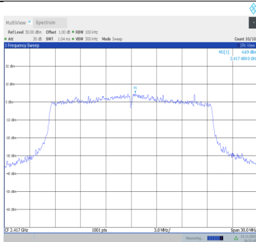
11ax20MIMO-Ant22-2417-0~Reference-PASS
