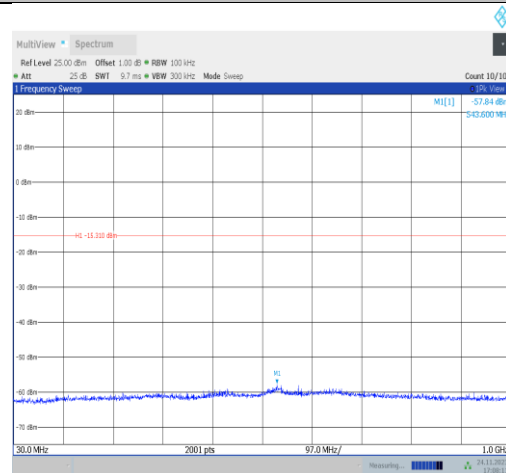
11ax20MIMO-Ant22-2417-30~1000-PASS
