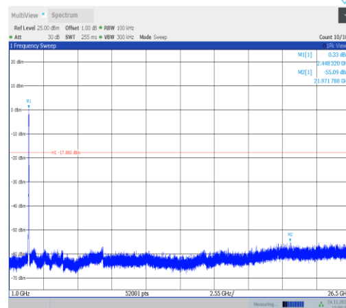
11VHT40MIMO-Ant25-2447-1000~26500-PASS
