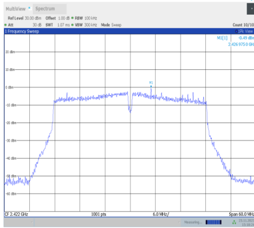
11VHT40MIMO-Ant22-2422-0~Reference-PASS
