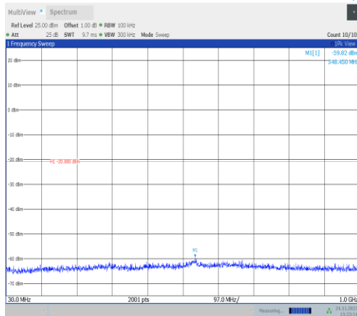
11VHT40MIMO-Ant25-2452-30~1000-PASS
