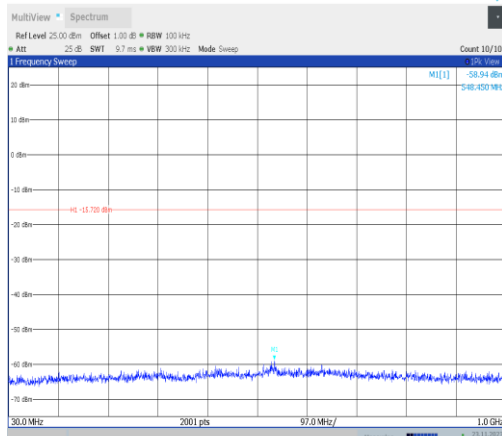
11VHT40MIMO-Ant25-2427-30~1000-PASS
