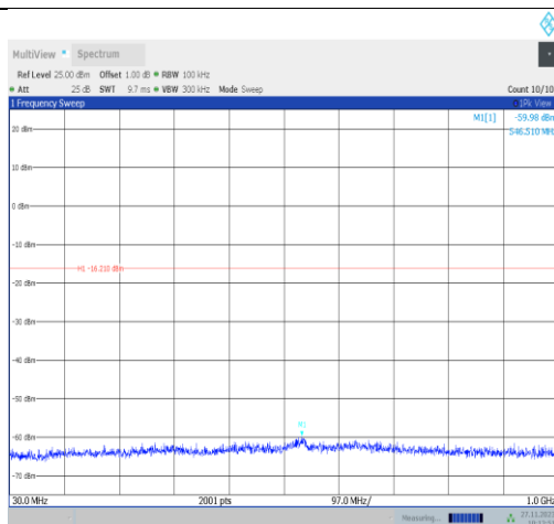
11ax40MIMO-Ant25-2447-30~1000-PASS
