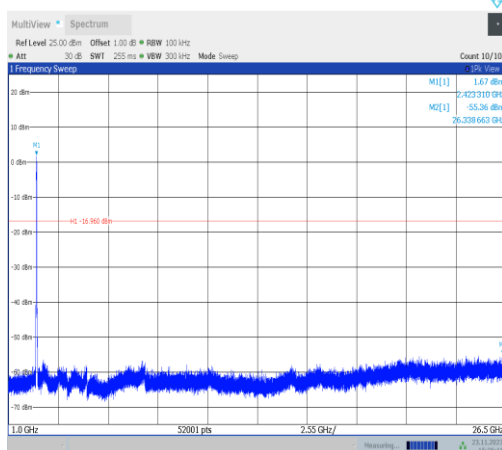
11VHT40MIMO-Ant22-2427-1000~26500-PASS
