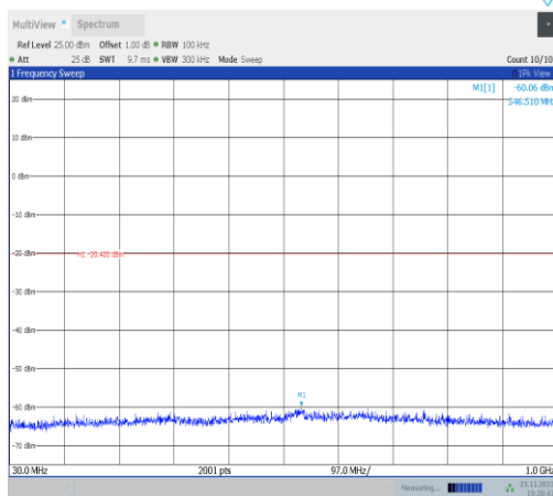
11VHT40MIMO-Ant25-2422-30~1000-PASS
