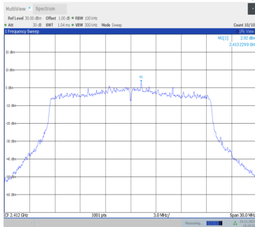
11ax20MIMO-Ant22-2412-0~Reference-PASS
