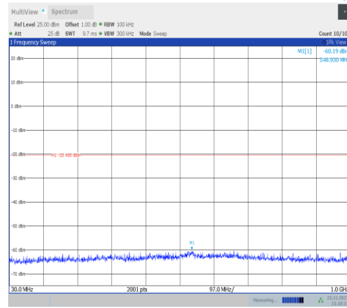
11VHT40MIMO-Ant22-2422-30~1000-PASS
