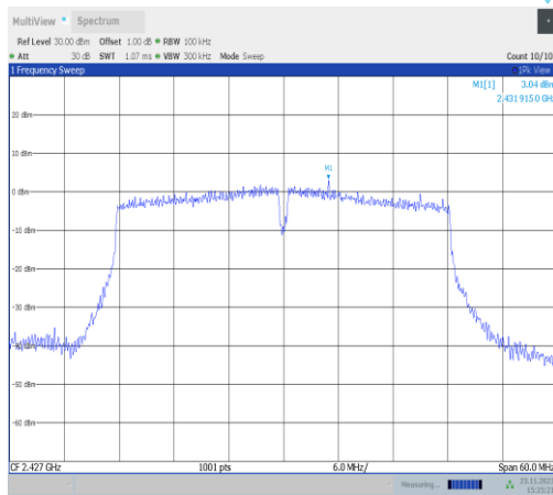
11VHT40MIMO-Ant22-2427-0~Reference-PASS
