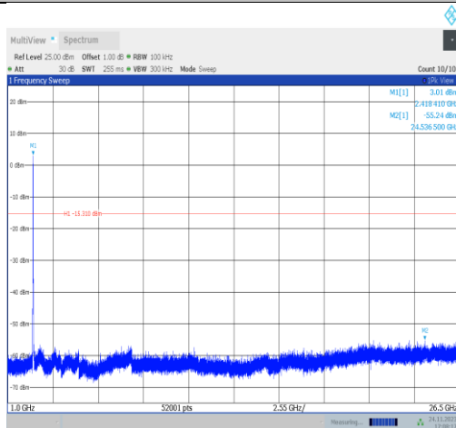
11ax20MIMO-Ant22-2417-1000~26500-PASS
