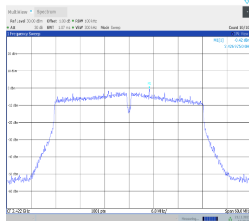
11VHT40MIMO-Ant25-2422-0~Reference-PASS
