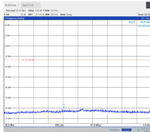
11ax20MIMO-Ant22-2457-30~1000-PASS
