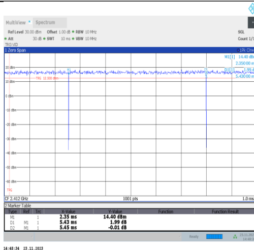
NTVN-11VHT20MIMO-Ant22-2412
