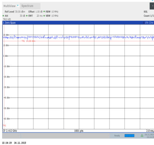
NTVN-11ax20MIMO-Ant22-2412
