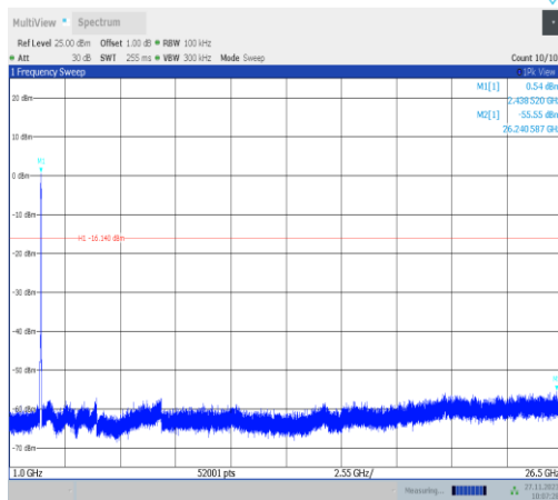
11ax40MIMO-Ant22-2437-1000~26500-PASS
