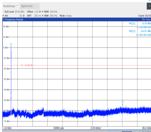
11VHT40MIMO-Ant22-2437-1000~26500-PASS
