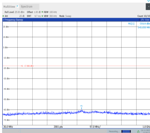
11VHT40MIMO-Ant25-2447-30~1000-PASS
