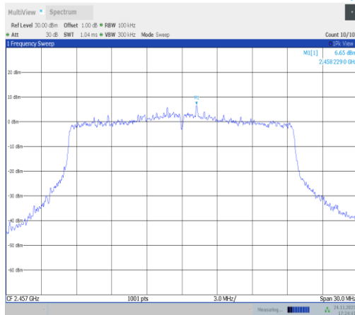
11ax20MIMO-Ant22-2457-0~Reference-PASS
