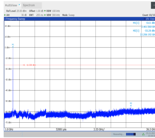
11VHT20MIMO-Ant25-2462-1000~26500-PASS
