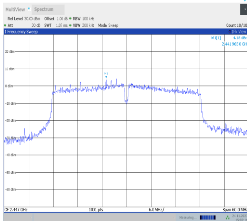
11VHT40MIMO-Ant22-2447-0~Reference-PASS
