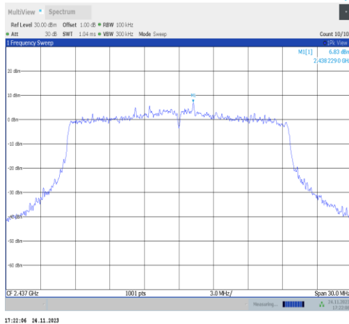
11ax20MIMO-Ant22-2437-0~Reference-PASS
