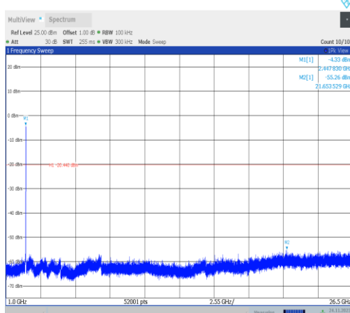
11VHT40MIMO-Ant22-2452-1000~26500-PASS
