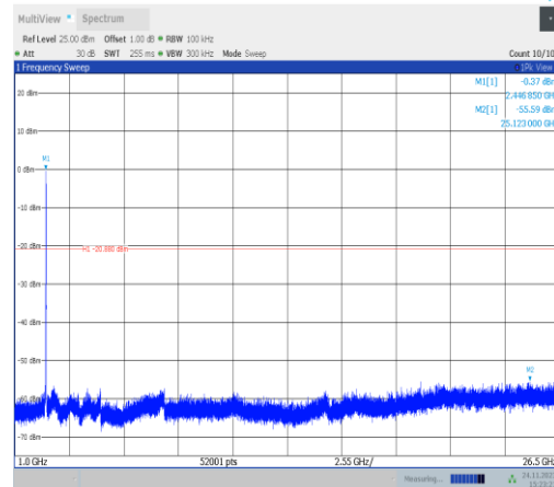
11VHT40MIMO-Ant25-2452-1000~26500-PASS
