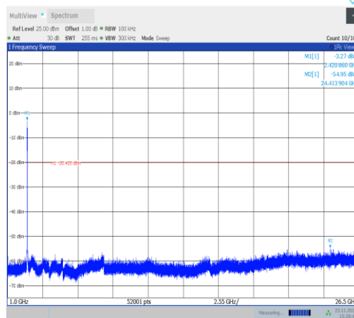
11VHT40MIMO-Ant25-2422-1000~26500-PASS
