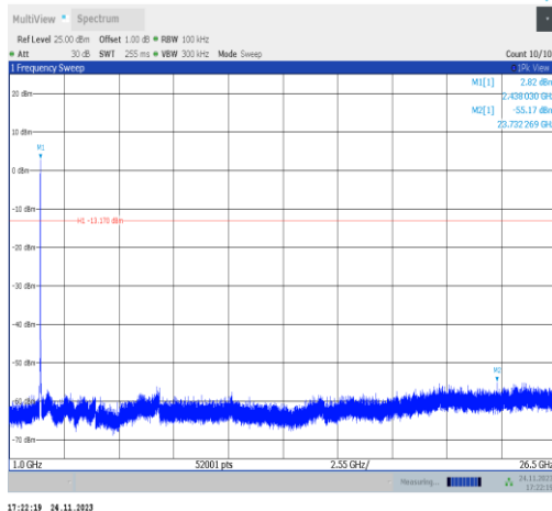
11ax20MIMO-Ant22-2437-1000~26500-PASS
