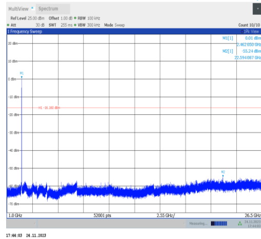
11ax20MIMO-Ant25-2462-1000~26500-PASS
