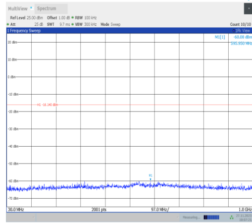
11ax40MIMO-Ant22-2437-30~1000-PASS
