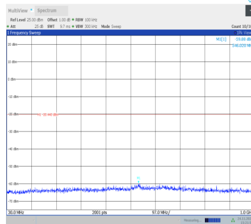
11VHT40MIMO-Ant22-2452-30~1000-PASS
