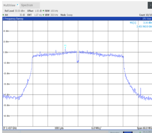
11VHT40MIMO-Ant22-2437-0~Reference-PASS
