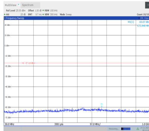
11ax40MIMO-Ant22-2447-30~1000-PASS
