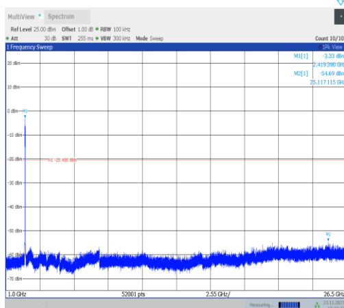
11VHT40MIMO-Ant22-2422-1000~26500-PASS
