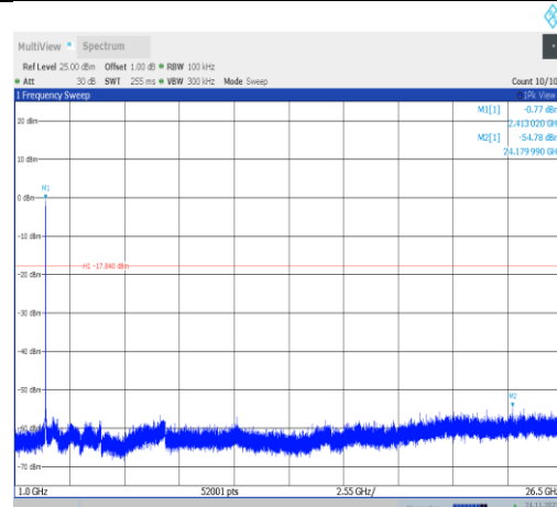
11ax20MIMO-Ant25-2412-1000~26500-PASS
