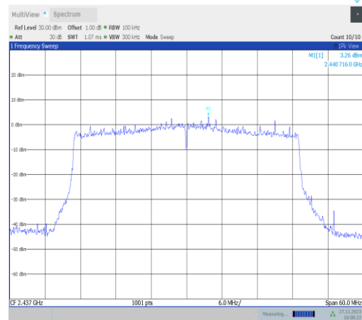
11ax40MIMO-Ant25-2437-0~Reference-PASS
