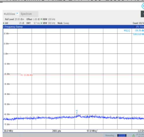
11ax40MIMO-Ant22-2452-30~1000-PASS
