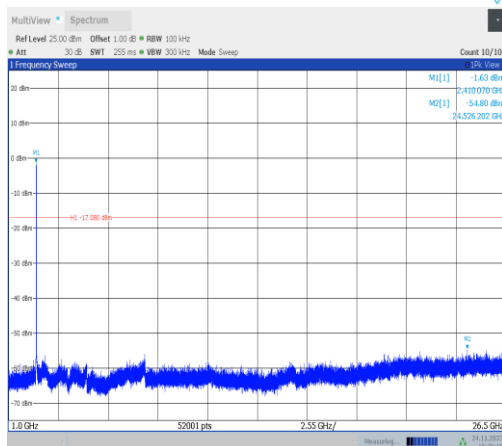
11ax20MIMO-Ant22-2412-1000~26500-PASS
