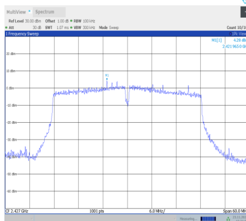
11VHT40MIMO-Ant25-2427-0~Reference-PASS
