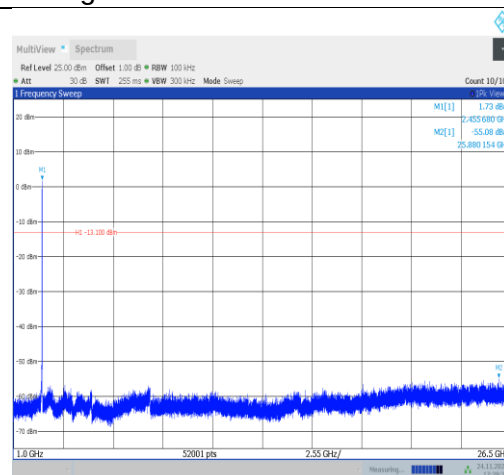
11ax20MIMO-Ant25-2457-1000~26500-PASS
