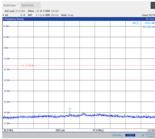
11VHT20MIMO-Ant25-2462-30~1000-PASS
