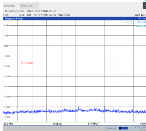
11VHT40MIMO-Ant22-2427-30~1000-PASS
