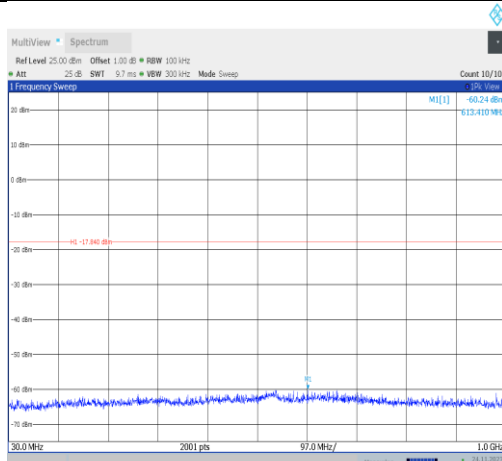
11ax20MIMO-Ant25-2412-30~1000-PASS
