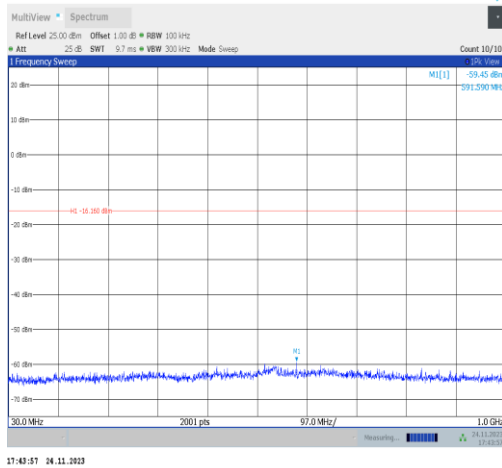
11ax20MIMO-Ant25-2462-30~1000-PASS
