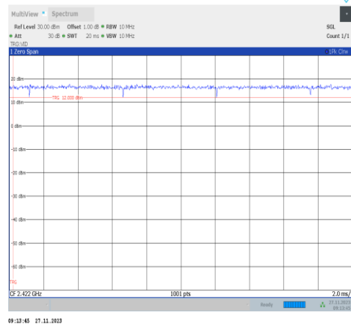
NTVN-11ax40MIMO-Ant25-2422
