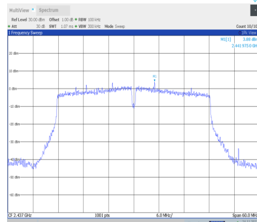
11VHT40MIMO-Ant25-2437-0~Reference-PASS
