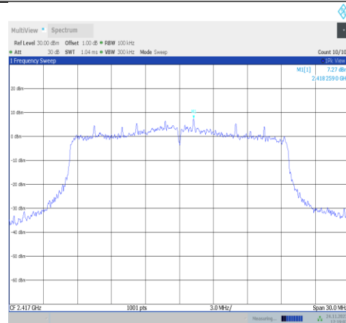
11ax20MIMO-Ant25-2417-0~Reference-PASS
