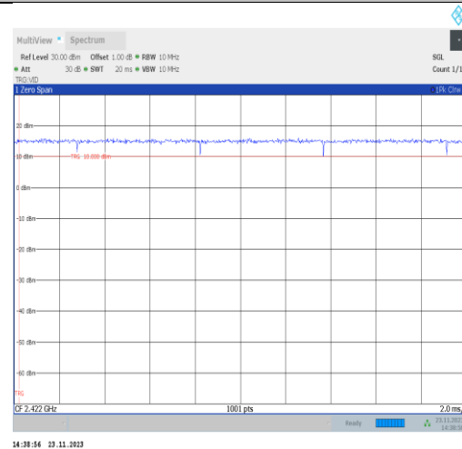
NTVN-11n40MIMO-Ant25-2422
