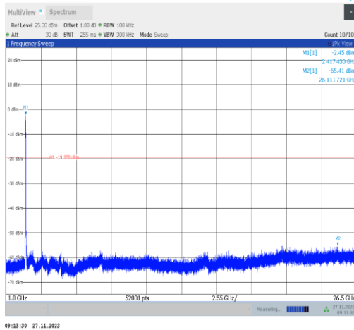
11ax40MIMO-Ant22-2422-1000~26500-PASS
