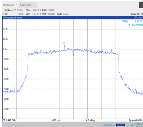
11ax40MIMO-Ant22-2447-0~Reference-PASS
