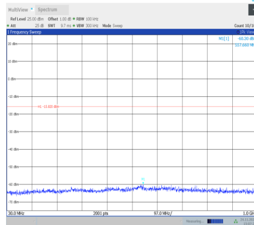
11VHT40MIMO-Ant22-2447-30~1000-PASS
