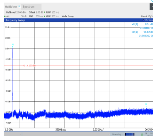
11VHT40MIMO-Ant25-2437-1000~26500-PASS
