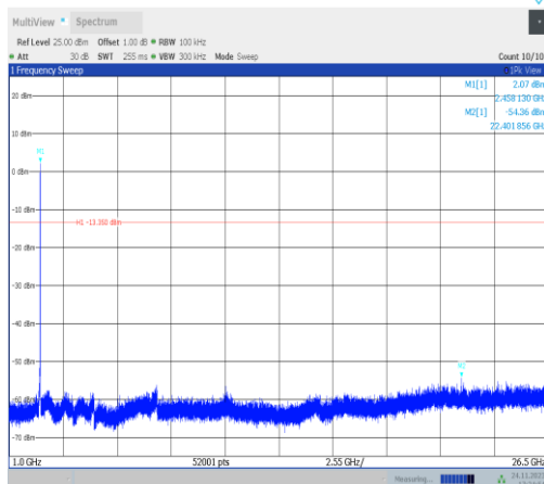
11ax20MIMO-Ant22-2457-1000~26500-PASS
