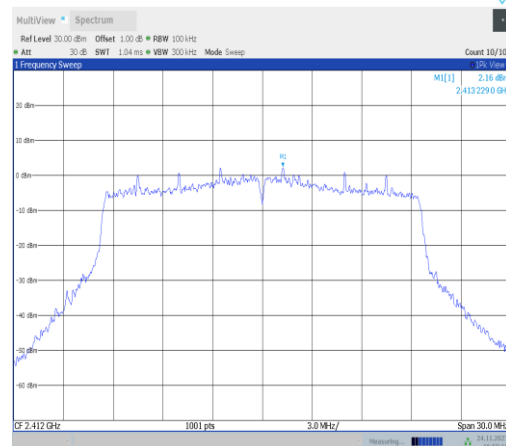
11ax20MIMO-Ant25-2412-0~Reference-PASS
