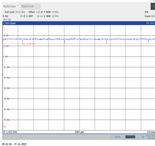
NTVN-11ax40MIMO-Ant22-2422
