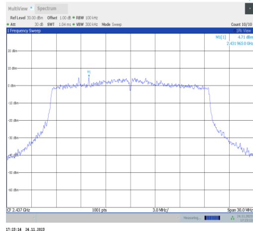
11ax20MIMO-Ant25-2437-0~Reference-PASS
