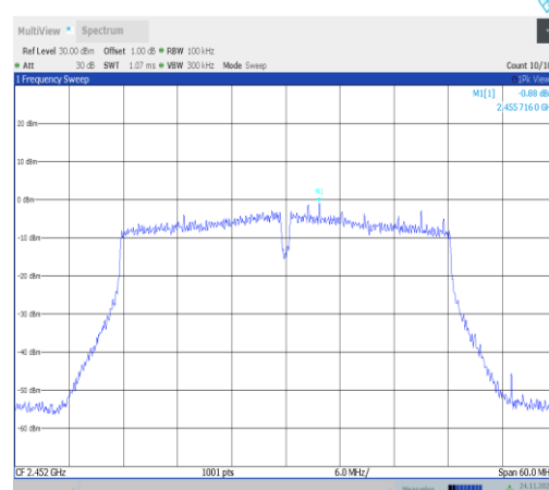
11VHT40MIMO-Ant25-2452-0~Reference-PASS
