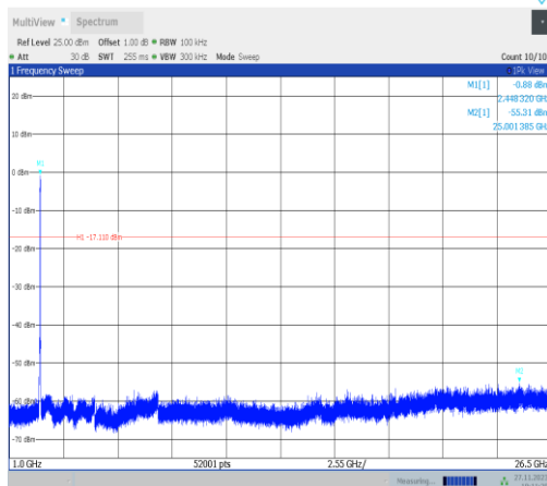
11ax40MIMO-Ant22-2447-1000~26500-PASS
