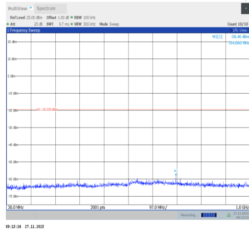
11ax40MIMO-Ant22-2422-30~1000-PASS
