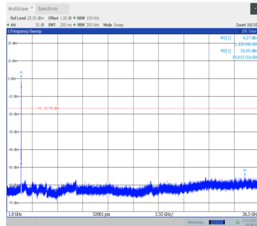
11ax40MIMO-Ant25-2437-1000~26500-PASS
