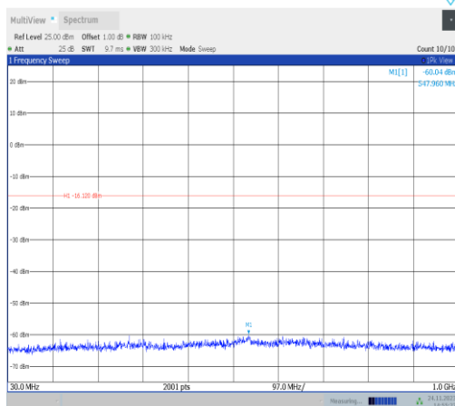
11VHT40MIMO-Ant25-2437-30~1000-PASS
