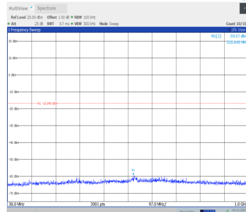
11VHT40MIMO-Ant22-2437-30~1000-PASS
