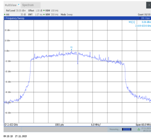
11ax40MIMO-Ant25-2422-0~Reference-PASS
