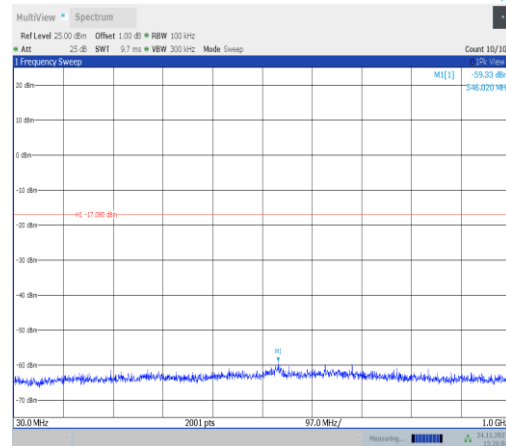
11ax20MIMO-Ant22-2412-30~1000-PASS
