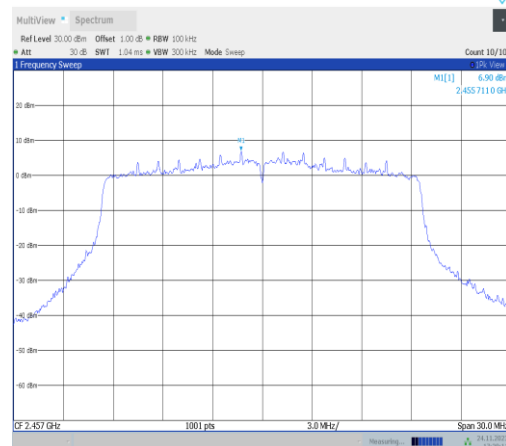
11ax20MIMO-Ant25-2457-0~Reference-PASS
