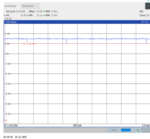
NTVN-11VHT40MIMO-Ant25-2422
