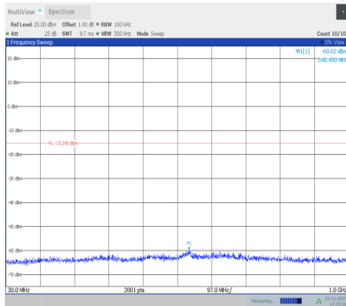
11ax20MIMO-Ant25-2437-30~1000-PASS
