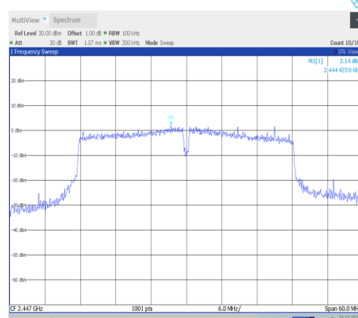
11VHT40MIMO-Ant25-2447-0~Reference-PASS
