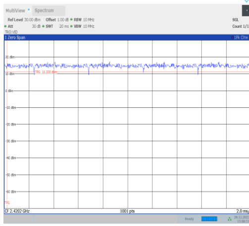
NTVN-11ax40MIMO-Ant22-2422-242Tone-RU61
