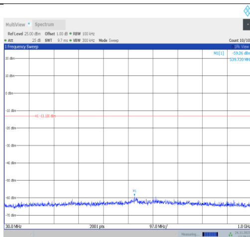
11ax20MIMO-Ant25-2457-30~1000-PASS
