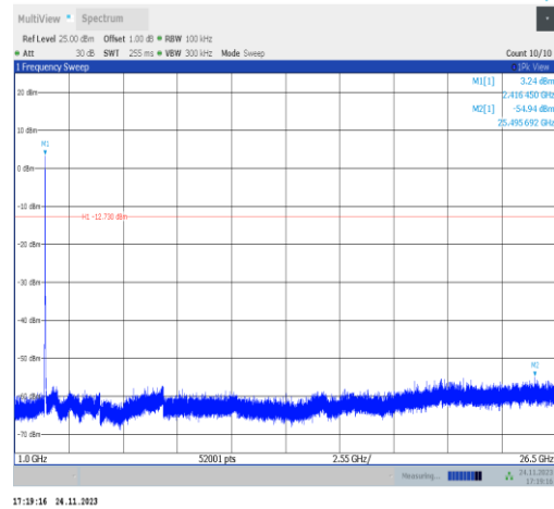
11ax20MIMO-Ant25-2417-1000~26500-PASS
