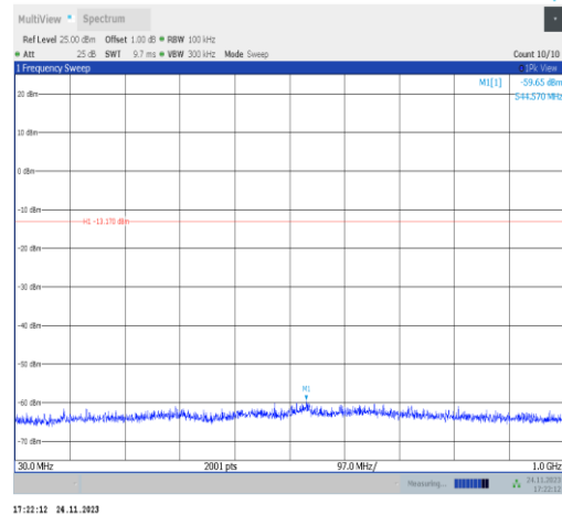
11ax20MIMO-Ant22-2437-30~1000-PASS
