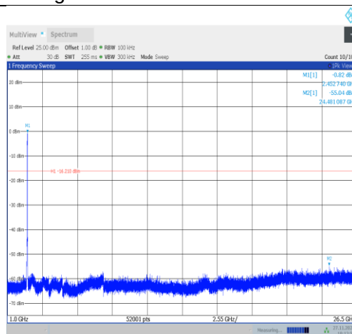
11ax40MIMO-Ant25-2447-1000~26500-PASS
