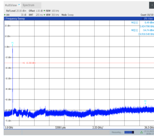
11ax40MIMO-Ant25-2427-1000~26500-PASS
