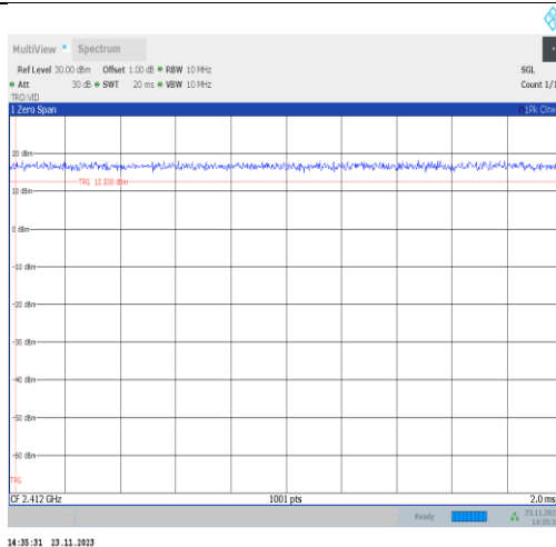
NTVN-11n20MIMO-Ant22-2412
