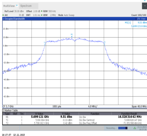
11a-CDD-Ant22-5700
