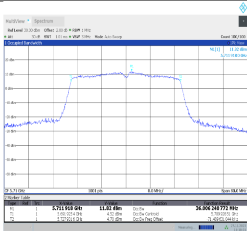
11n40MIMO-Ant22-5710
