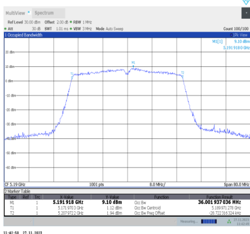
11n40MIMO-Ant22-5190
