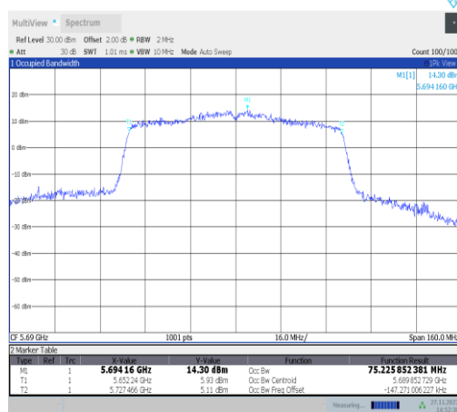
11ac80MIMO-Ant25-5690
