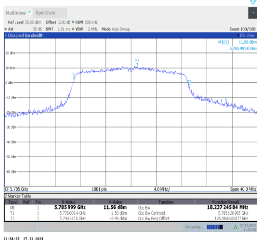
11n20MIMO-Ant22-5785
