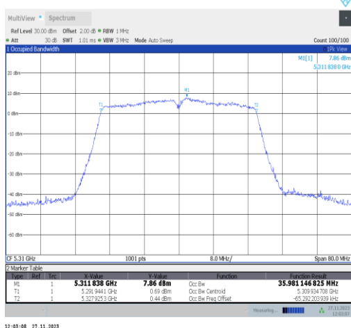
11n40MIMO-Ant22-5310
