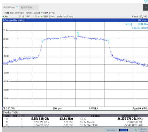
11n40MIMO-Ant22-5550
