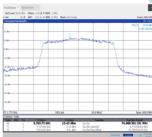
11ac80MIMO-Ant25-5775
