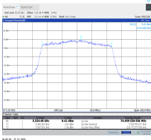
11ac80MIMO-Ant22-5530
