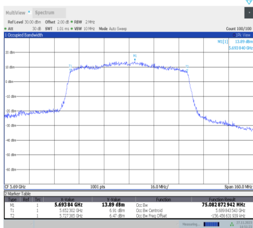
11ac80MIMO-Ant22-5690
