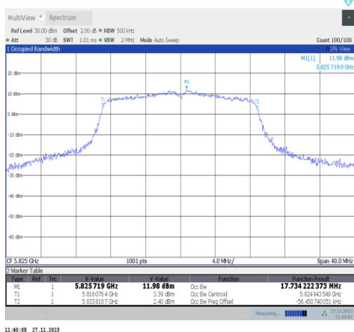
11n20MIMO-Ant22-5825
