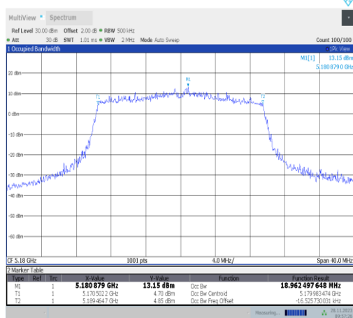
11ax20MIMO-Ant25-5180
