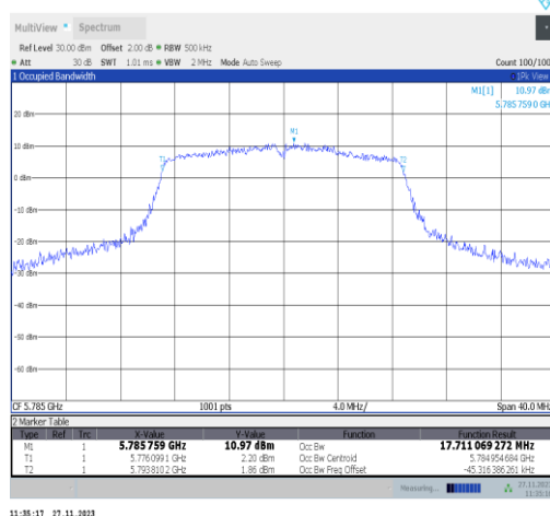
11n20MIMO-Ant25-5785
