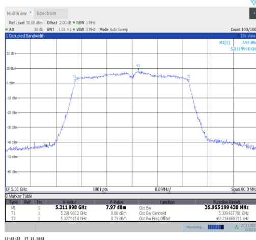
11n40MIMO-Ant25-5310
