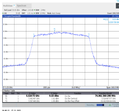
11ac80MIMO-Ant25-5530
