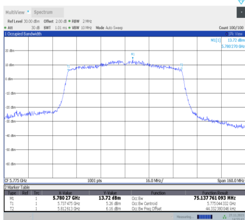
11ac80MIMO-Ant22-5775
