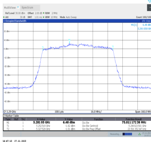
11ac80MIMO-Ant25-5290
