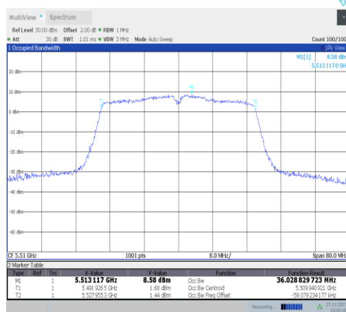
11n40MIMO-Ant25-5510
