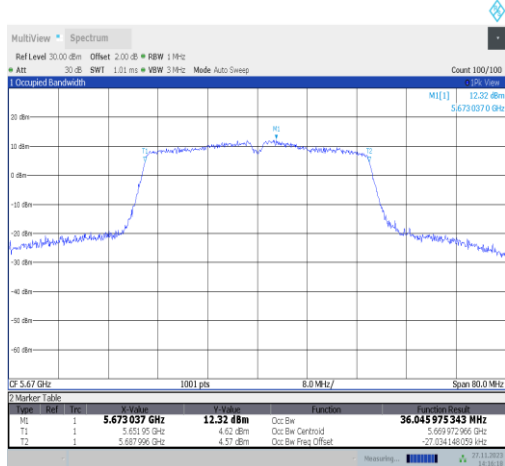
11n40MIMO-Ant22-5670
