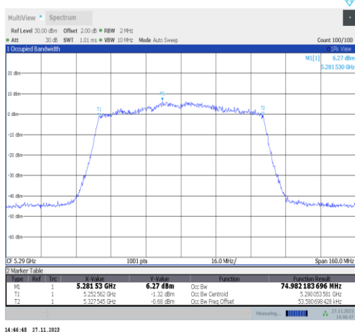
11ac80MIMO-Ant22-5290
