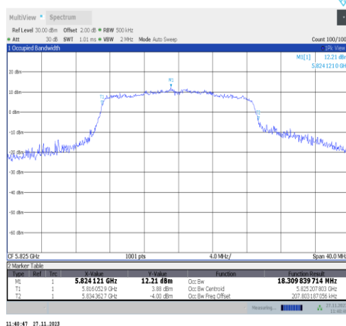
11n20MIMO-Ant25-5825
