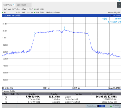
11n40MIMO-Ant22-5755
