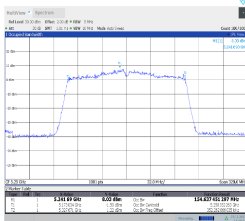
11ac160MIMO-Ant25-5250
