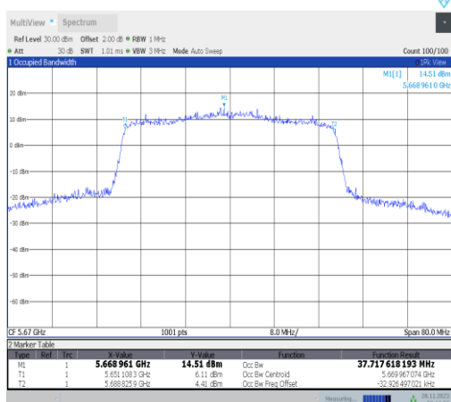
11ax40MIMO-Ant22-5670
