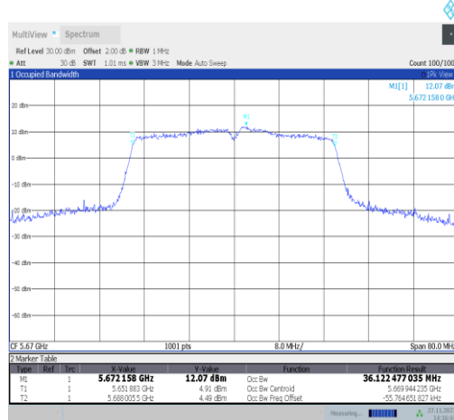
11n40MIMO-Ant25-5670
