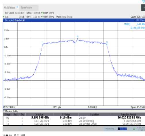
11n40MIMO-Ant25-5190
