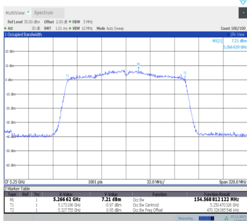
11ac160MIMO-Ant22-5250
