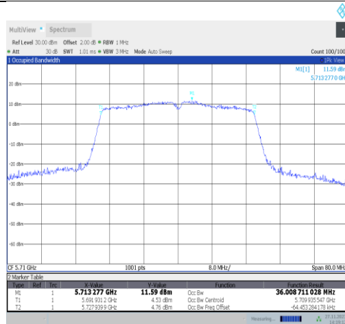
11n40MIMO-Ant25-5710
