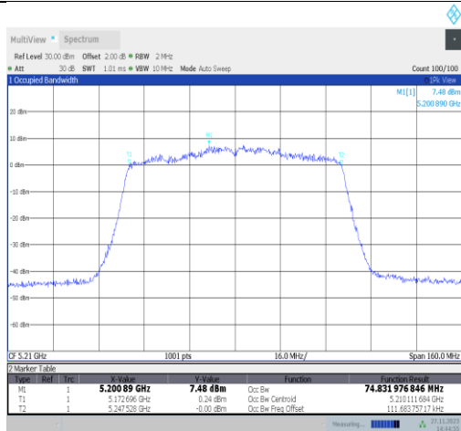
11ac80MIMO-Ant22-5210
