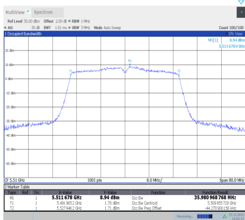
11n40MIMO-Ant22-5510
