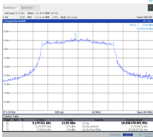
11ax20MIMO-Ant22-5180
