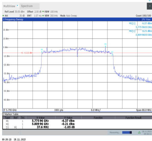
11ax40MIMO-Ant22-5795-PASS
