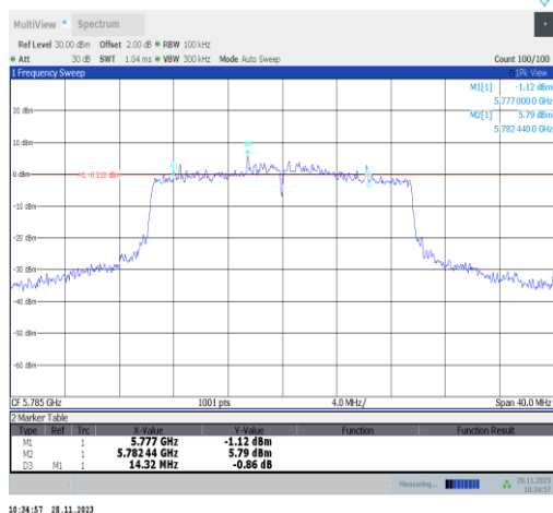
11ax20MIMO-Ant22-5785-PASS
