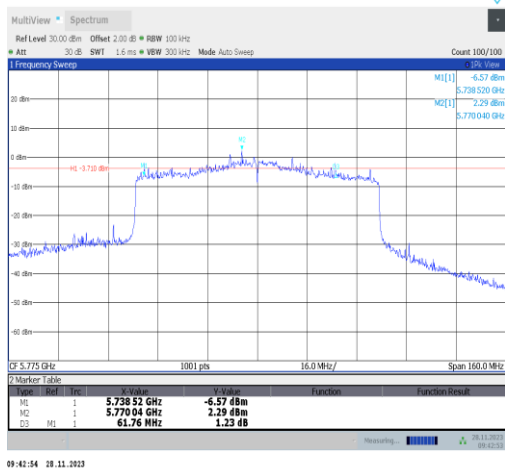
11ax80MIMO-Ant22-5775-PASS
