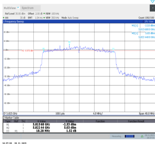
11ax20MIMO-Ant22-5825-PASS
