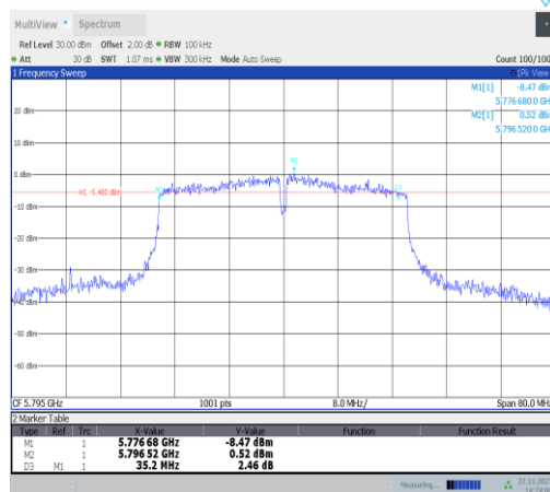
11n40MIMO-Ant25-5795-PASS
