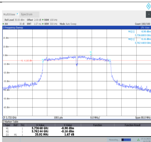
11n40MIMO-Ant22-5755-PASS
