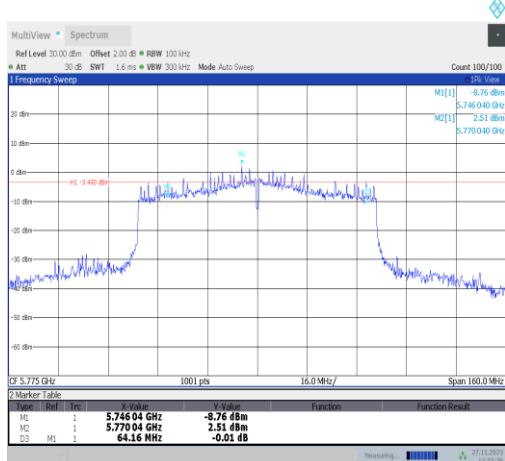
11ac80MIMO-Ant22-5775-PASS
