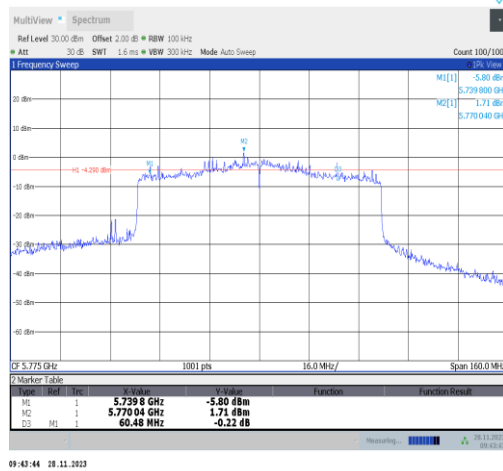
11ax80MIMO-Ant25-5775-PASS
