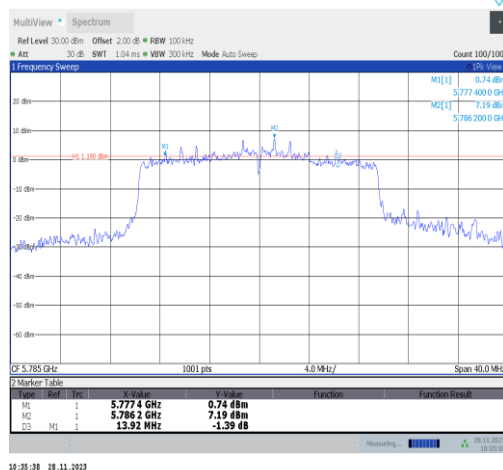
11ax20MIMO-Ant25-5785-PASS
