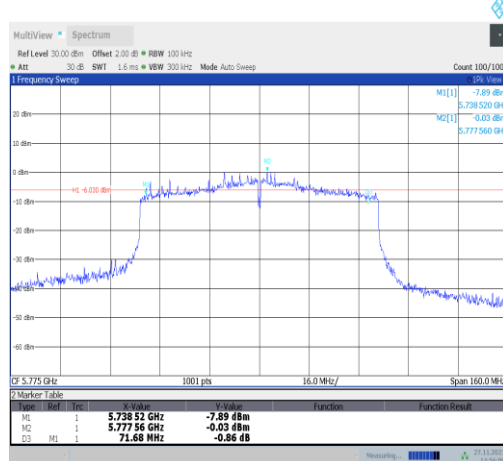
11ac80MIMO-Ant25-5775-PASS
