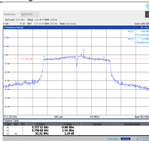
11n40MIMO-Ant25-5755-PASS
