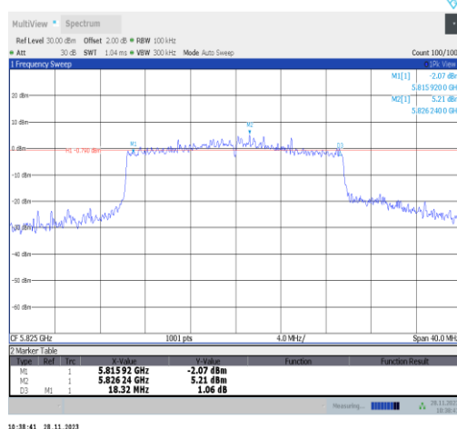
11ax20MIMO-Ant25-5825-PASS
