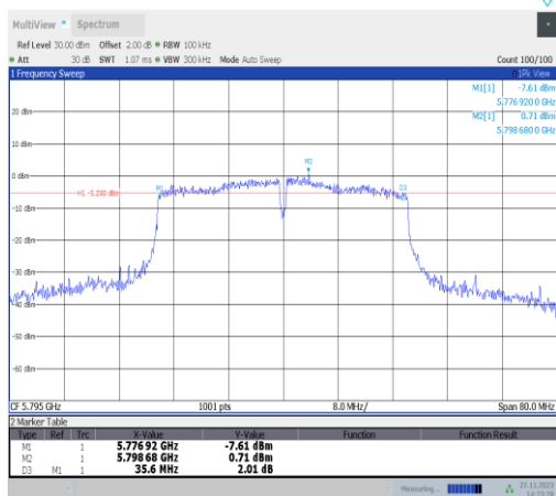
11n40MIMO-Ant22-5795-PASS
