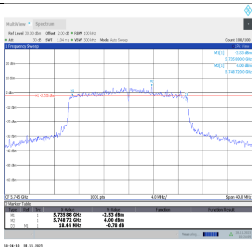
11ax20MIMO-Ant22-5745-PASS
