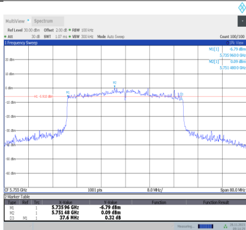
11ax40MIMO-Ant22-5755-PASS
