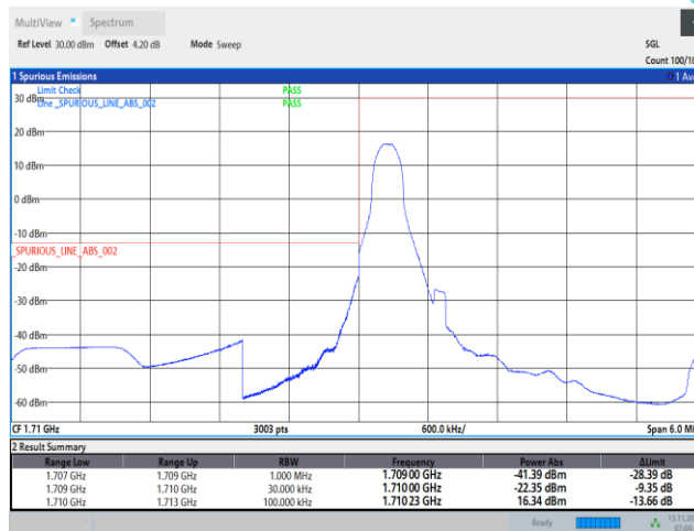
Band4-1.4MHz-QPSK-19957-6RB#0
