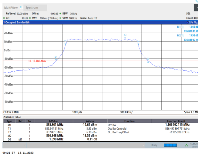
Band5-1.4MHz-16QAM-20525-6RB#0
