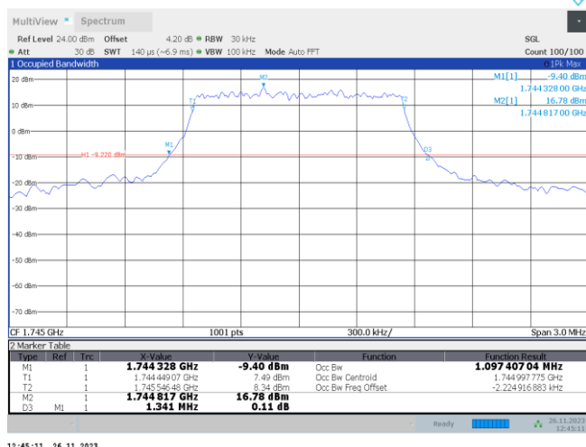
Band66-1.4MHz-16QAM-132322-6RB#0
