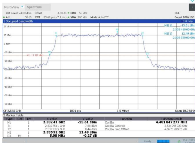
Band7-5MHz-16QAM-21100-25RB#0
