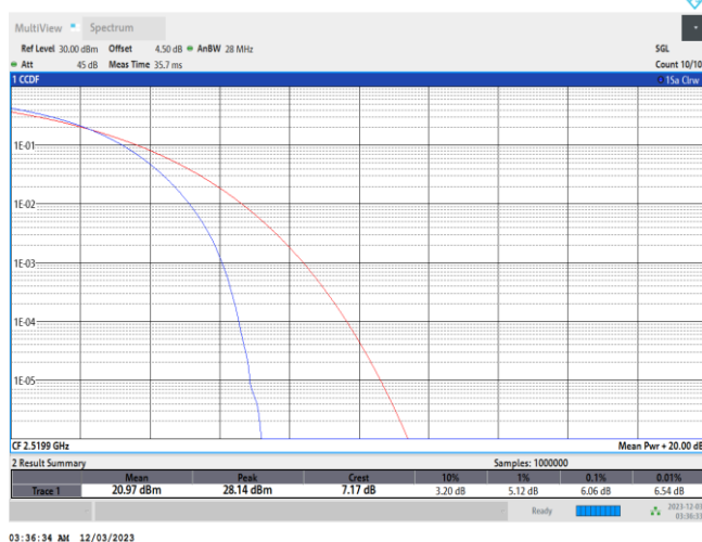
7-7-20MHz-20MHz-QPSK-QPSK-21001-21199-100RB#0-100RB#0
