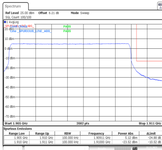
1-N2-PC3-15-5-H-6-CP-QPSK-Outer_Full-25@0-A nt14-1-seegraph-PASS-see graph
