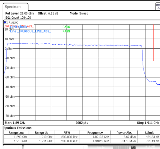
1-N2-PC3-15-20-H-3-DFT-PI2BPSK-Outer_Full-100@0-Ant14-1-seegraph-PASS-see graph
