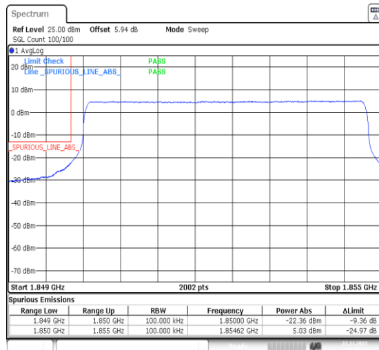
1-N2-PC3-15-5-L-6-CP-QPSK-Outer_Full-25@0-A nt14-1-seegraph-PASS-see graph
