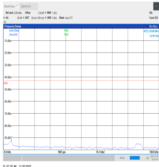
NTNV_N2_PC3_15_20_L_TID1_0.009_0.15_#1
