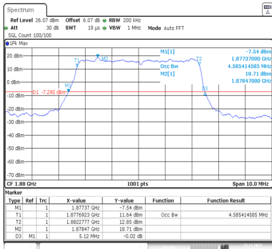
1-N2-PC3-15-5-M-1-DFT-QPSK-Outer_Full-25@0-A nt14-4.585-5.120-≤5-PASS
