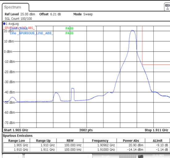
1-N2-PC3-15-5-H-2-DFT-PI2BPSK-Edge_1RB_Right-1 @24-Ant14-1-seegraph-PASS-see graph
