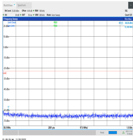
NTNV_N2_PC3_15_20_L_TID1_30_1000_#1
