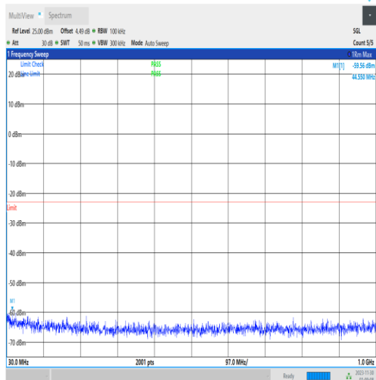
NTVN_N2_PC3_15_20_M_TID1_30_1000_#1
