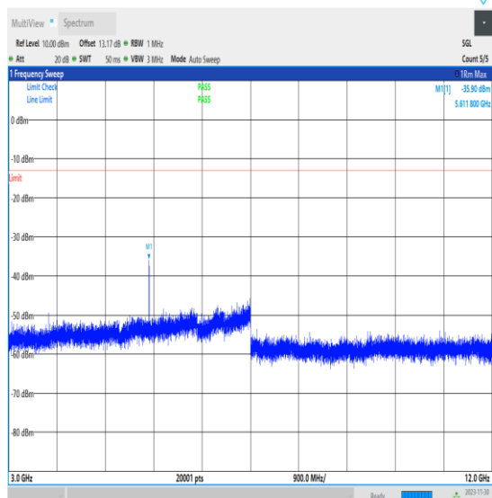
NTVN_N2_PC3_15_20_M_TID1_3000_12000_#1
