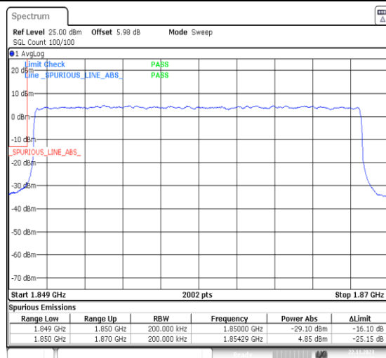
1-N2-PC3-15-20-L-3-DFT-PI2BPSK-Outer_Full-10 0@0-Ant14-1-seegraph-PASS-see graph
