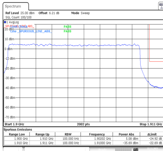
1-N2-PC3-15-10-H-3-DFT-PI2BPSK-Outer_Full-50@0-Ant14-1-seegraph-PASS-see graph
