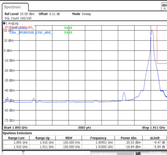
1-N2-PC3-15-15-H-5-CP-QPSK-Edge_1RB_Right-1@78-Ant14-1-seegraph-PASS-see graph
