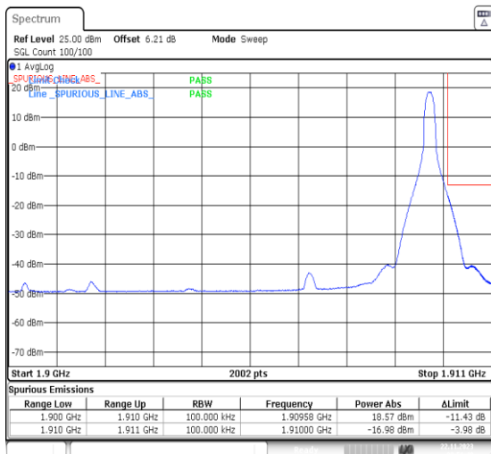
1-N2-PC3-15-10-H-5-CP-QPSK-Edge_1RB_Right-1@51-Ant14-1-seegraph-PASS-see graph
