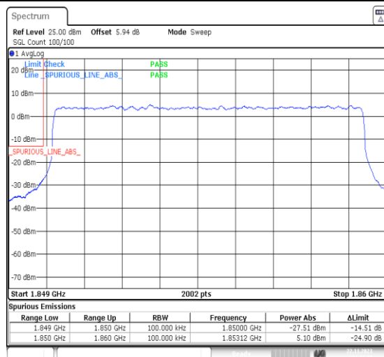
1-N2-PC3-15-10-L-3-DFT-PI2BPSK-Outer_Full-50 @0-Ant14-1-seegraph-PASS-see graph
