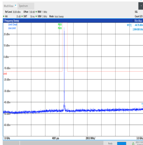
NTVN_N2_PC3_15_20_M_TID1_1000_3000_#1
