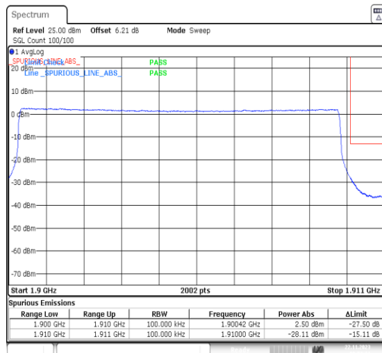
1-N2-PC3-15-10-H-6-CP-QPSK-Outer_Full-52@0-Ant14-1-seegraph-PASS-see graph
