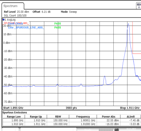
1-N2-PC3-15-15-H-2-DFT-PI2BPSK-Edge_1RB_Right-1@78-Ant14-1-seegraph-PASS-see graph
