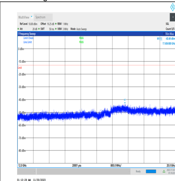
NTNV_N2_PC3_15_20_H_TID1_12000_20000_#1
