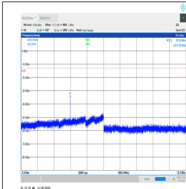
NTNV_N2_PC3_15_20_H_TID1_3000_12000_#1
