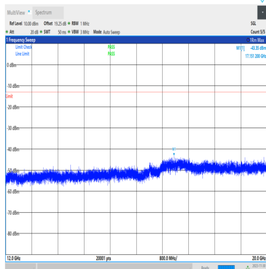
NTVN_N2_PC3_15_20_M_TID1_12000_20000_#1
