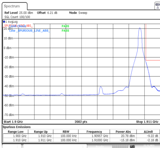
1-N2-PC3-15-10-H-2-DFT-PI2BPSK-Edge_1RB_Right-1@51-Ant14-1-seegraph-PASS-see graph
