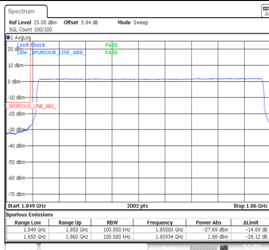
1-N2-PC3-15-10-L-6-CP-QPSK-Outer_Full-52@0-Ant14-1-seegraph-PASS-see graph
