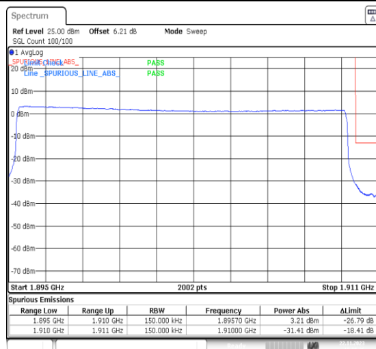
1-N2-PC3-15-15-H-6-CP-QPSK-Outer_Full-79@0-Ant14-1-seegraph-PASS-see graph
