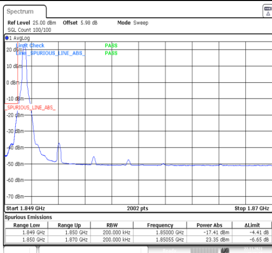
1-N2-PC3-15-20-L-1-DFT-PI2BPSK-Edge_1RB_Left-1 @0-Ant14-1-seegraph-PASS-see graph
