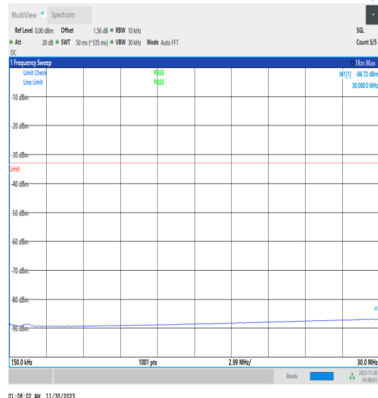
NTNV_N2_PC3_15_20_L_TID1_0.15_30_#1
