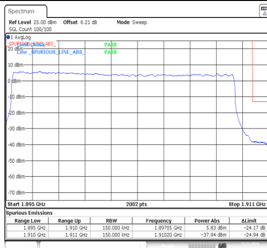
1-N2-PC3-15-15-H-3-DFT-PI2BPSK-Outer_Full-75@0-Ant14-1-seegraph-PASS-see graph
