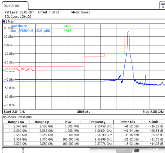
1-N38-PC3-30-10-L-4-CP-QPSK-Edge_1RB_Left-1@0-Ant31-1--PASS-see graph
