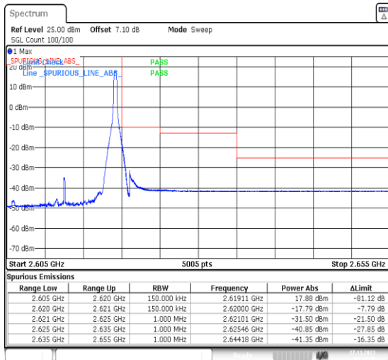
1-N38-PC3-30-15-H-2-DFT-PI2BPSK-Edge_1RB_Righ t-1@37-Ant31-1--PASS-see graph
