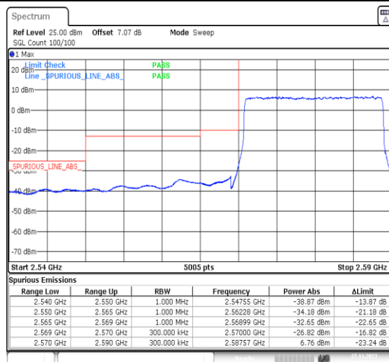
1-N38-PC3-30-20-L-3-DFT-PI2BPSK-Outer_Full-50@0-Ant31-1--PASS-see graph
