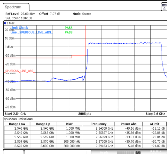
1-N38-PC3-30-30-L-3-DFT-PI2BPSK-Outer_Full-75@0-Ant31-1--PASS-see graph
