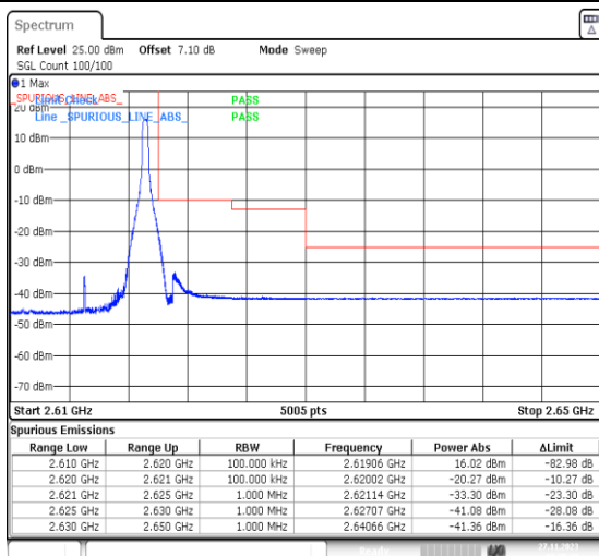
1-N38-PC3-30-10-H-2-DFT-PI2BPSK-Edge_1RB_Right-t-1@23-Ant31-1--PASS-see graph
