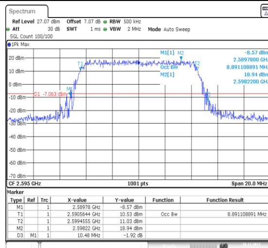
1-N38-PC3-30-10-M-4-DFT-64QAM-Outter_Full-24@ 0-Ant31-8.891-10.480-≤10-PASS
