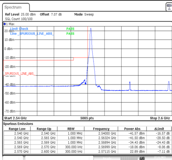
1-N38-PC3-30-30-L-1-DFT-PI2BPSK-Edge_1RB_Left-1@0-Ant31-1--PASS-see graph
