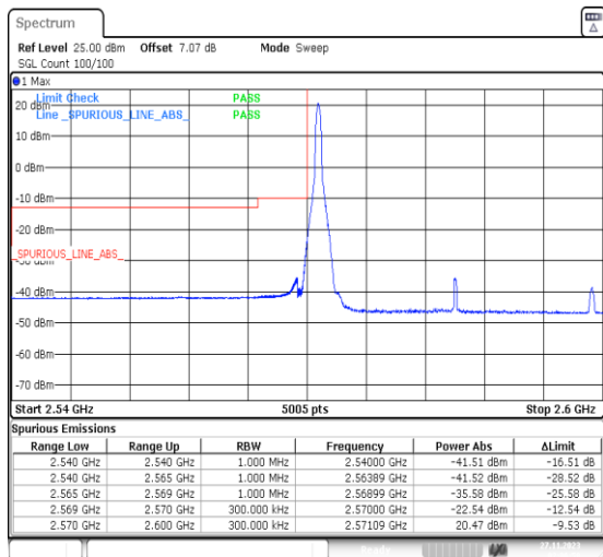
1-N38-PC3-30-30-L-4-CP-QPSK-Edge_1RB_Left-1@0-Ant31-1--PASS-see graph
