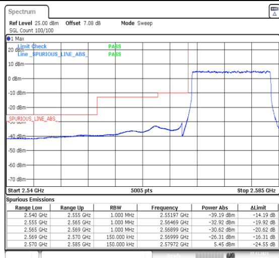
1-N38-PC3-30-15-L-3-DFT-PI2BPSK-Outer_Full-36@0-Ant31-1--PASS-see graph
