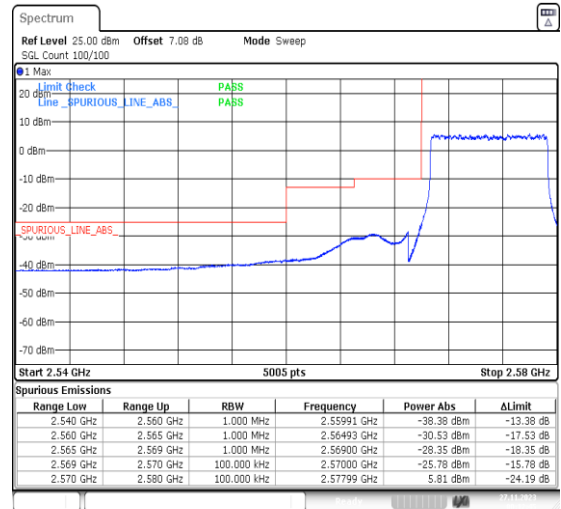
1-N38-PC3-30-10-L-3-DFT-PI2BPSK-Outer_Full-24@0-Ant31-1--PASS-see graph
