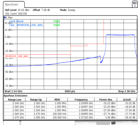
1-N38-PC3-30-10-L-6-CP-QPSK-Outer_Full-24@0-Ant31-1--PASS-see graph
