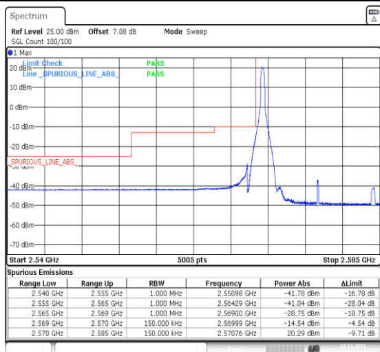
1-N38-PC3-30-15-L-1-DFT-PI2BPSK-Edge_1RB_Left-1@0-Ant31-1--PASS-see graph
