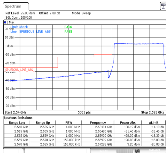
1-N38-PC3-30-15-L-6-CP-QPSK-Outer_Full-38@0-Ant31-1--PASS-see graph
