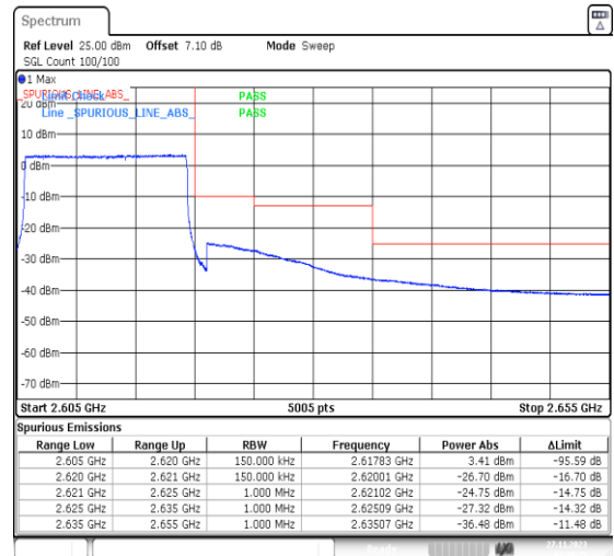
1-N38-PC3-30-15-H-3-DFT-PI2BPSK-Outer_Full-3 6@0-Ant31-1--PASS-see graph
