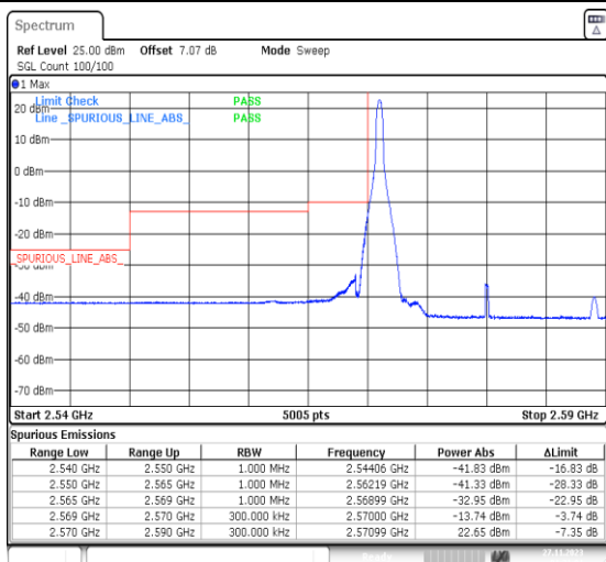
1-N38-PC3-30-20-L-1-DFT-PI2BPSK-Edge_1RB_Left-1@0-Ant31-1--PASS-see graph
