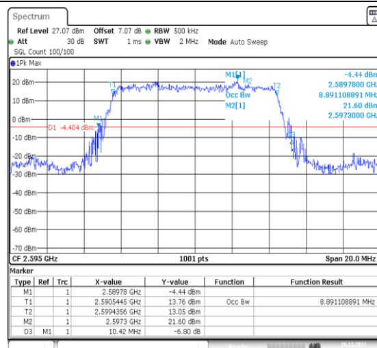
1-N38-PC3-30-10-M-2-DFT-PI2BPSK-Outter_Full-24 @0-Ant31-8.891-10.420-≤10-PASS
