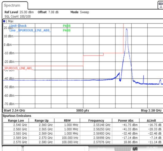
1-N38-PC3-30-10-L-1-DFT-PI2BPSK-Edge_1RB_Left-1@0-Ant31-1--PASS-see graph
