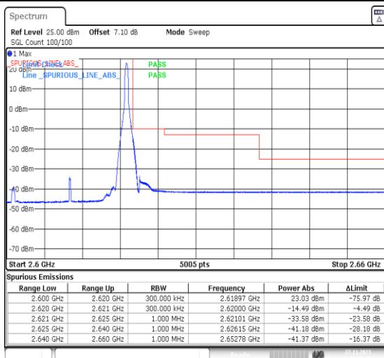
1-N38-PC3-30-20-H-2-DFT-PI2BPSK-Edge_1RB_Righ t-1@50-Ant31-1--PASS-see graph
