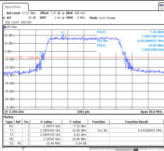
1-N38-PC3-30-10-M-3-DFT-16QAM-Outter_Full-24@ 0-Ant31-8.931-10.460-≤10-PASS
