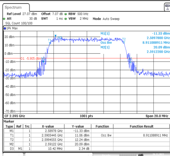
1-N38-PC3-30-10-M-1-DFT-QPSK-Outter_Full-24@0 -Ant31-8.911-10.420-≤10-PASS
