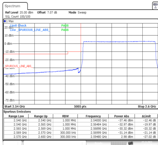
1-N38-PC3-30-30-L-6-CP-QPSK-Outer_Full-78@0-Ant31-1--PASS-see graph
