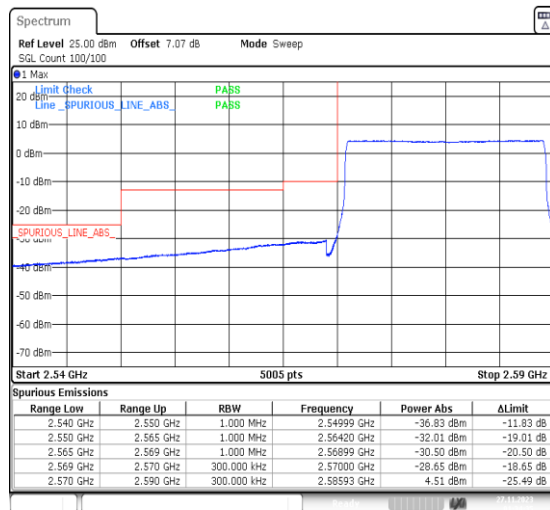
1-N38-PC3-30-20-L-6-CP-QPSK-Outer_Full-51@0-Ant31-1--PASS-see graph
