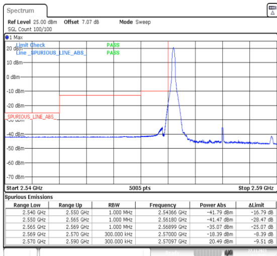
1-N38-PC3-30-20-L-4-CP-QPSK-Edge_1RB_Left-1@0-Ant31-1--PASS-see graph
