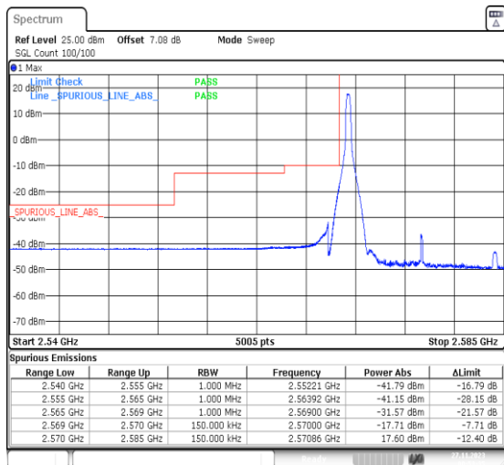
1-N38-PC3-30-15-L-4-CP-QPSK-Edge_1RB_Left-1@0-Ant31-1--PASS-see graph
