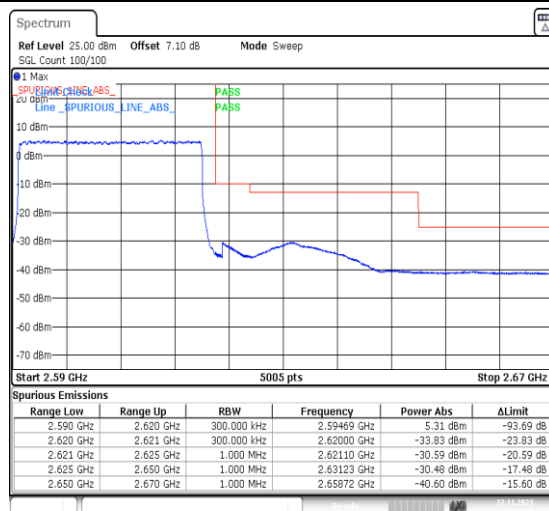
1-N38-PC3-30-30-H-3-DFT-PI2BPSK-Outer_Full-75@0-Ant31-1--PASS-see graph
