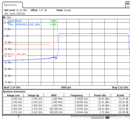
1-N38-PC3-30-40-L-6-CP-QPSK-Outer_Full-106@0-Ant31-1--PASS-see graph
