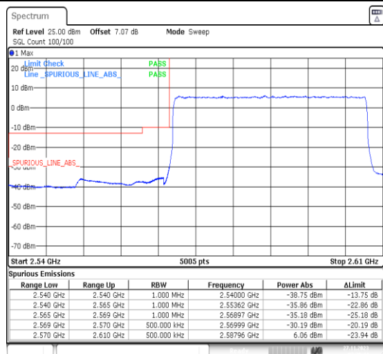
1-N38-PC3-30-40-L-3-DFT-PI2BPSK-Outer_Full-100@0-Ant31-1--PASS-see graph
