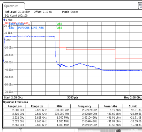
1-N38-PC3-30-40-H-3-DFT-PI2BPSK-Outer_Full-100@0-Ant31-1--PASS-see graph
