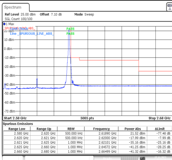
1-N38-PC3-40-H-2-DFT-PI2BPSK-Edge_1RB_Right-t-1@105-Ant31-1--PASS-see graph
