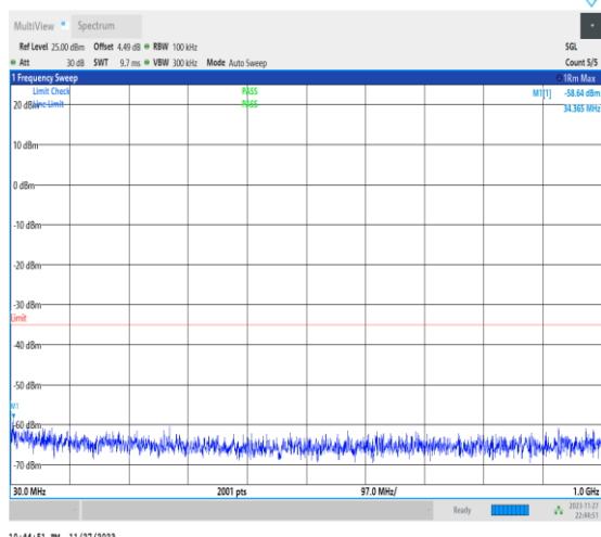
1-N38-PC3-30-40-M-1-DFT-PI2BPSK-Inner_1RB_L eft-1@1-30-1000-Ant31-866.14--58.64--35-PASS
