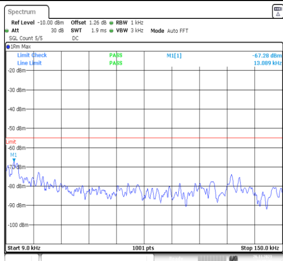
1-N38-PC3-30-40-H-1-DFT-PI2BPSK-Inner_1RB_L eft-1@1-0.009-0.15-Ant31-0.01--67.28--55-PASS
