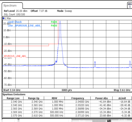
1-N38-PC3-30-40-L-1-DFT-PI2BPSK-Edge_1RB_Left-1@0-Ant31-1--PASS-see graph
