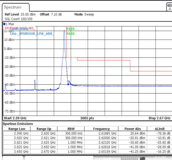
1-N38-PC3-30-30-H-2-DFT-PI2BPSK-Edge_1RB_Right-t-1@77-Ant31-1--PASS-see graph
