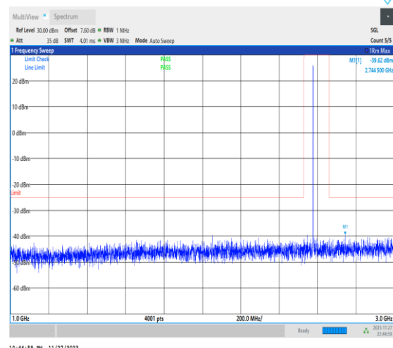
1-N38-PC3-30-40-M-1-DFT-PI2BPSK-Inner_1RB_Lef t-1@1-1000-3000-Ant31-2910.50--39.62--25-PASS
