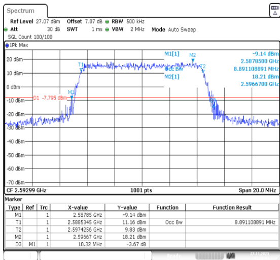
1-N41-PC2-30-10-M-3-DFT-16QAM-Outter_Full-24 @0-Ant31-8.891-10.320-≤10-PASS
