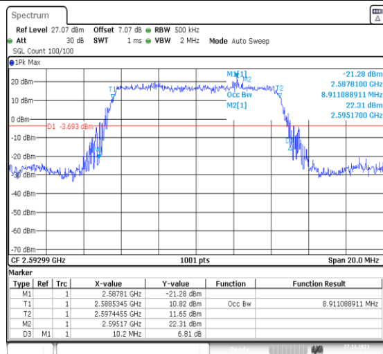
1-N41-PC2-30-10-M-2-DFT-PI2BPSK-Outter_Full-24 @0-Ant31-8.911-10.200-≤10-PASS
