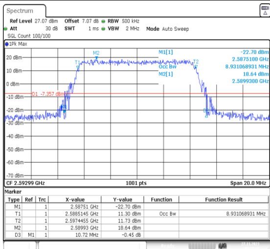
1-N41-PC2-30-10-M-1-DFT-QPSK-Outter_Full-24@0 -Ant31-8.931-10.720-≤10-PASS
