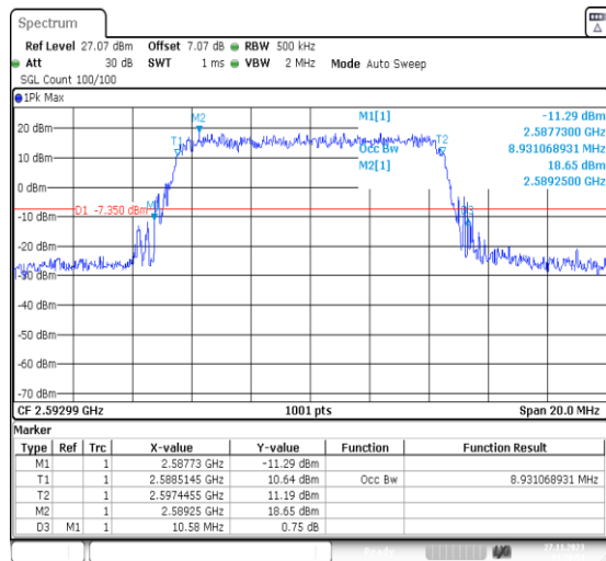
1-N41-PC2-30-10-M-4-DFT-64QAM-Outter_Full-24@ 0-Ant31-8.931-10.580-≤10-PASS
