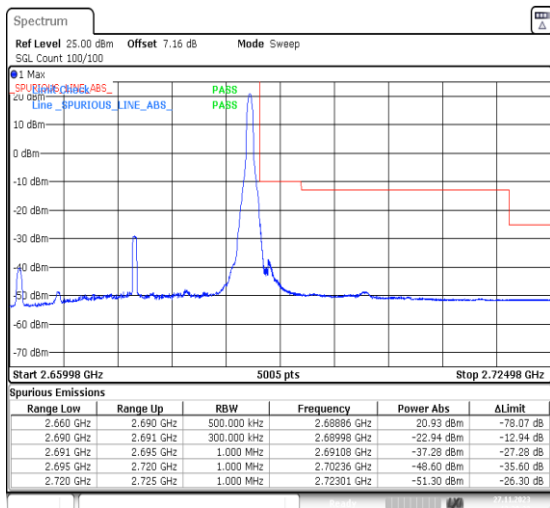
1-N41-PC2-30-30-H-5-CP-QPSK-Edge_1RB_Right-1 @77-Ant31-1--PASS-see graph
