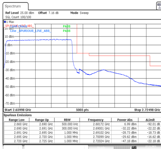
1-N41-PC2-30-30-H-3-DFT-PI2BPSK-Outer_Full-7 5@0-Ant31-1--PASS-see graph
