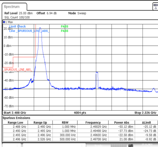
1-N41-PC2-30-30-L-4-CP-QPSK-Edge_1RB_Left-1@0-Ant31-1--PASS-see graph
