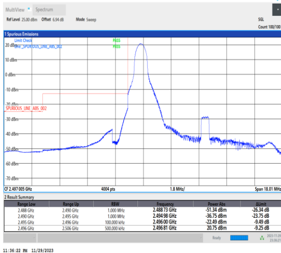
1-N41-PC2-30-10-L-4-CP-QPSK-Edge_1RB_Left-1@0-Ant31-1--PASS-see graph
