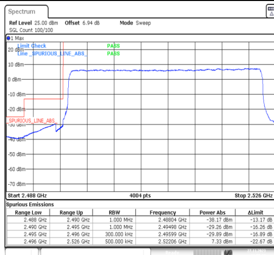
1-N41-PC2-30-30-L-3-DFT-PI2BPSK-Outer_Full-75@0-Ant31-1--PASS-see graph
