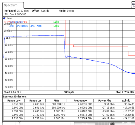
1-N41-PC2-30-40-H-6-CP-QPSK-Outer_Full-106@0-Ant31-1--PASS-see graph
