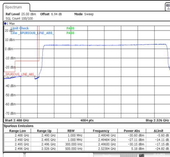
1-N41-PC2-30-30-L-6-CP-QPSK-Outer_Full-78@0-Ant31-1--PASS-see graph
