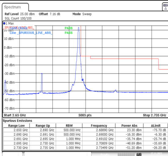
1-N41-PC2-30-40-H-2-DFT-PI2BPSK-Edge_1RB_Right-t-1@105-Ant31-1--PASS-see graph
