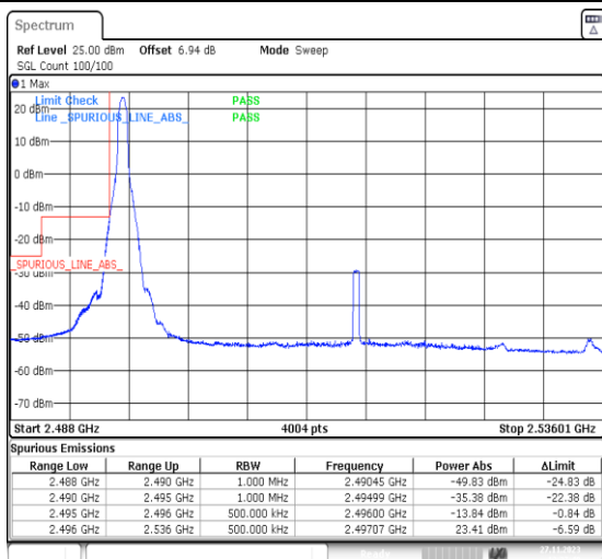
1-N41-PC2-30-40-L-1-DFT-PI2BPSK-Edge_1RB_Left-1@0-Ant31-1--PASS-see graph
