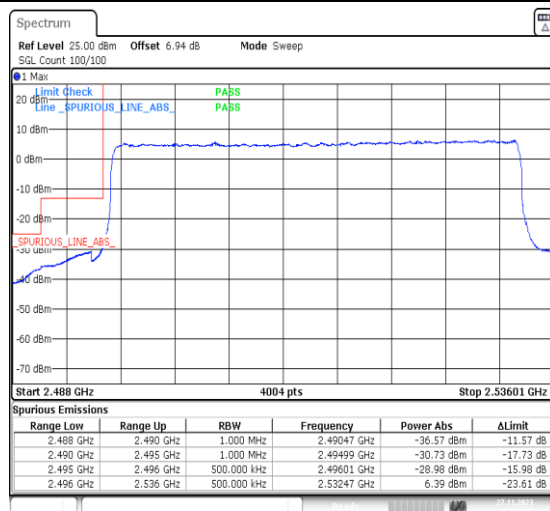
1-N41-PC2-30-40-L-3-DFT-PI2BPSK-Outer_Full-100@0-Ant31-1--PASS-see graph
