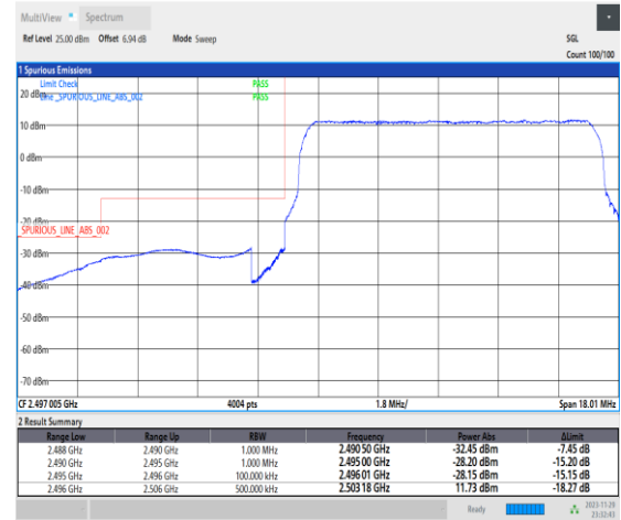
1-N41-PC2-30-10-L-3-DFT-PI2BPSK-Outer_Full-24@0-Ant31-1--PASS-see graph
