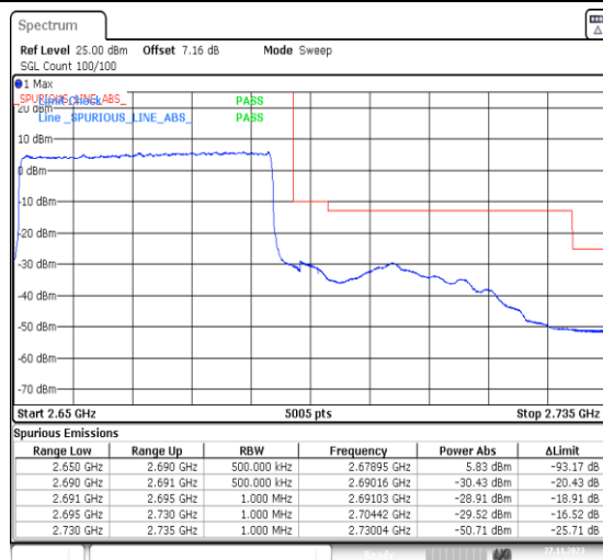
1-N41-PC2-30-40-H-3-DFT-PI2BPSK-Outer_Full-100@0-Ant31-1--PASS-see graph
