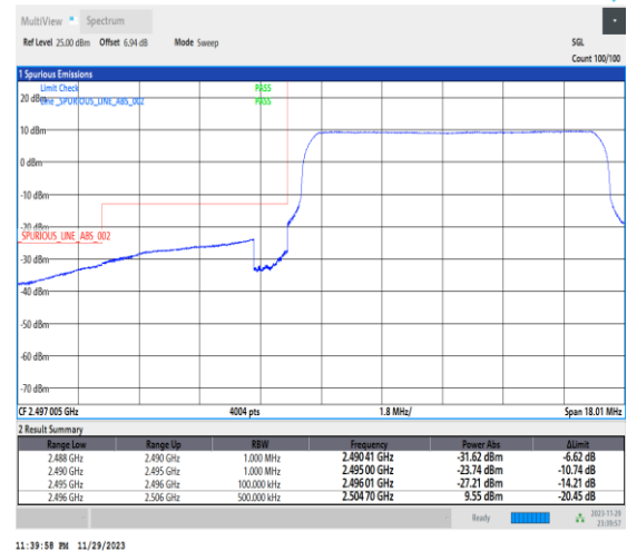
1-N41-PC2-30-10-L-6-CP-QPSK-Outer_Full-24@0-Ant31-1--PASS-see graph
