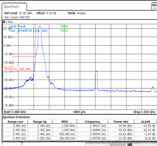
1-N41-PC2-30-30-L-1-DFT-PI2BPSK-Edge_1RB_Left-1@0-Ant31-1--PASS-see graph
