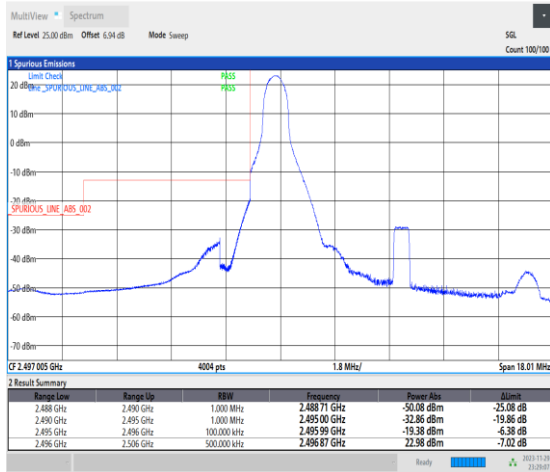
1-N41-PC2-30-10-L-1-DFT-PI2BPSK-Edge_1RB_Left-1@0-Ant31-1--PASS-see graph
