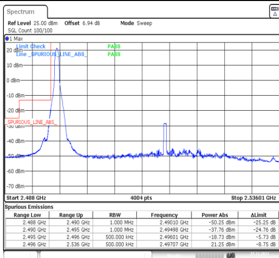
1-N41-PC2-30-40-L-4-CP-QPSK-Edge_1RB_Left-1@0-Ant31-1--PASS-see graph
