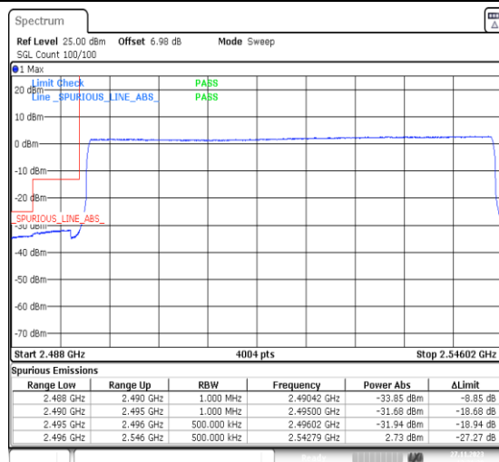
1-N41-PC2-30-50-L-6-CP-QPSK-Outer_Full-133@0-Ant31-1--PASS-see graph
