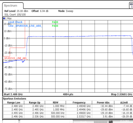
1-N41-PC2-30-40-L-6-CP-QPSK-Outer_Full-106@0-Ant31-1--PASS-see graph
