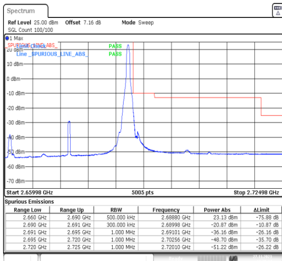
1-N41-PC2-30-30-H-2-DFT-PI2BPSK-Edge_1RB_Righ t-1@77-Ant31-1--PASS-see graph
