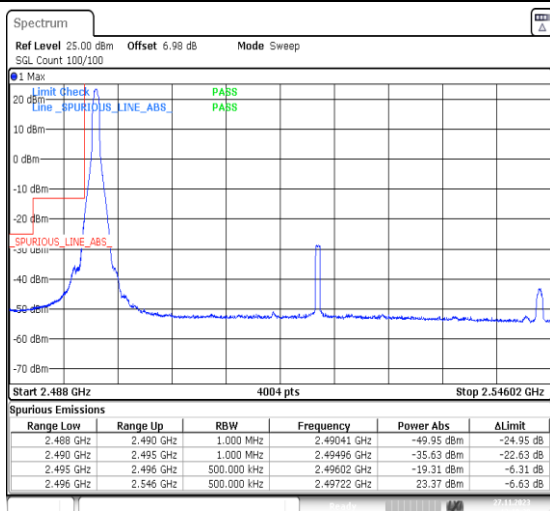
1-N41-PC2-30-50-L-1-DFT-PI2BPSK-Edge_1RB_Left-1@0-Ant31-1--PASS-see graph
