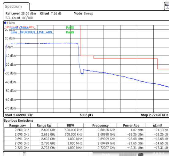
1-N41-PC2-30-30-H-6-CP-QPSK-Outer_Full-78@ 0-Ant31-1--PASS-see graph
