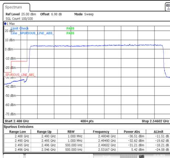
1-N41-PC2-30-50-L-3-DFT-PI2BPSK-Outer_Full-128@0-Ant31-1--PASS-see graph
