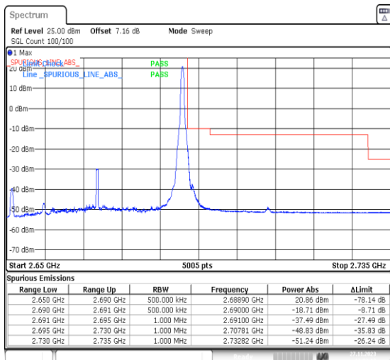
1-N41-PC2-30-40-H-5-CP-QPSK-Edge_1RB_Right-1@105-Ant31-1--PASS-see graph
