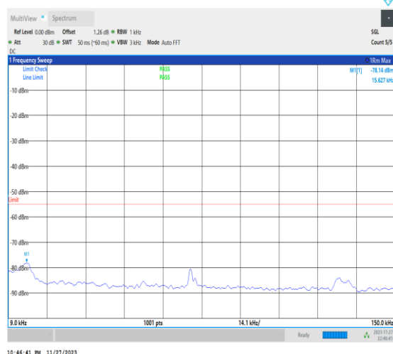
1-N41-PC2-30-100-M-1-DFT-PI2BPSK-Inner_1RB_L Left-1@1-0.009-0.15-Ant31-0.01--78.14--55-PASS
