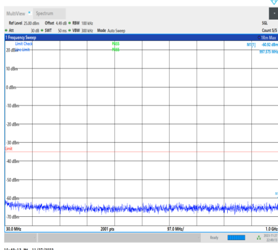
1-N41-PC2-30-100-H-1-DFT-PI2BPSK-Inner_1RB_L eft-1@1-30-1000-Ant31-916.58--60.92--35-PASS
