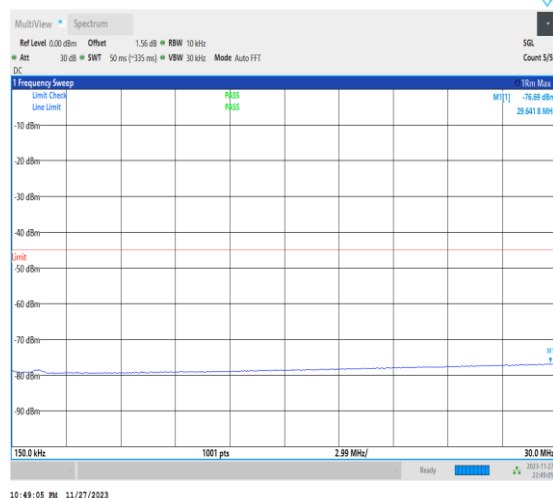
1-N41-PC2-30-100-H-1-DFT-PI2BPSK-Inner_1RB_L eft-1@1-0.15-30-Ant31-28.21--76.69--45-PASS
