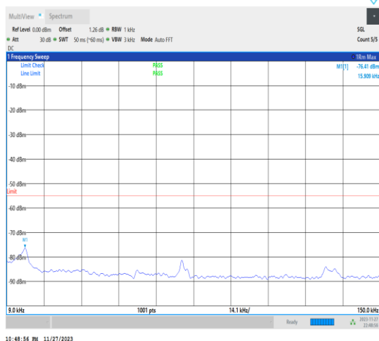
1-N41-PC2-30-100-H-1-DFT-PI2BPSK-Inner_1RB_L eft-1@1-0.009-0.15-Ant31-0.01--76.41--55-PASS
