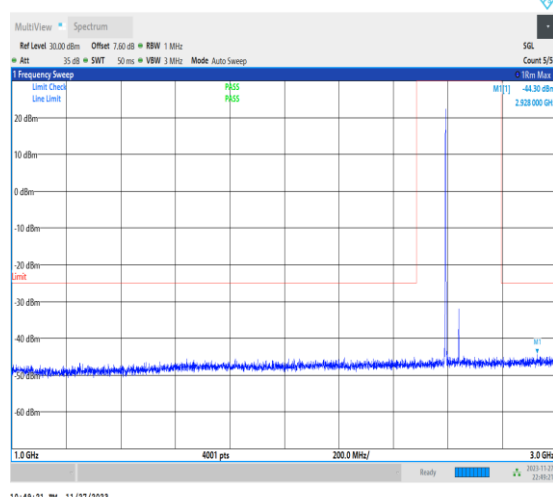
1-N41-PC2-30-100-H-1-DFT-PI2BPSK-Inner_1RB_L eft-1@1-1000-3000-Ant31-2849.50--44.30--25-PASS
